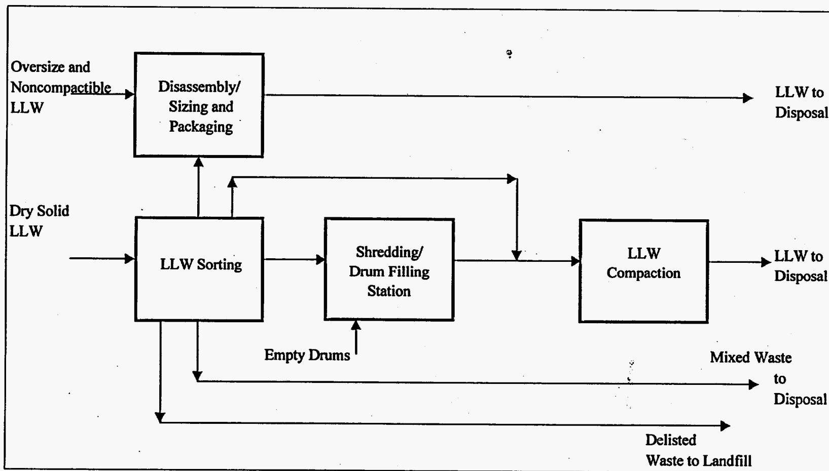
Figure IV-3. Dry Active Waste Processing (Baseline Option)
