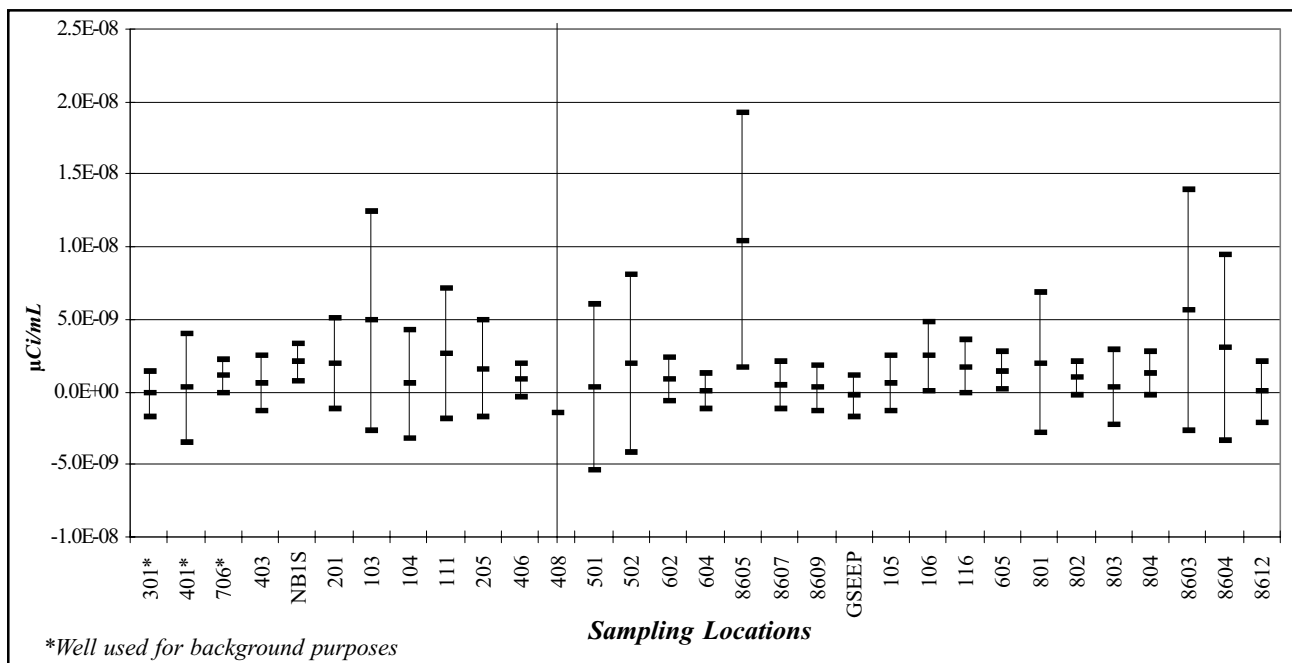
Figure E-3a. Gross Alpha ( \mu\text{Ci/mL} ) in Groundwater Samples from the Sand and Gravel Unit (magnified scale of Fig. E-3)
