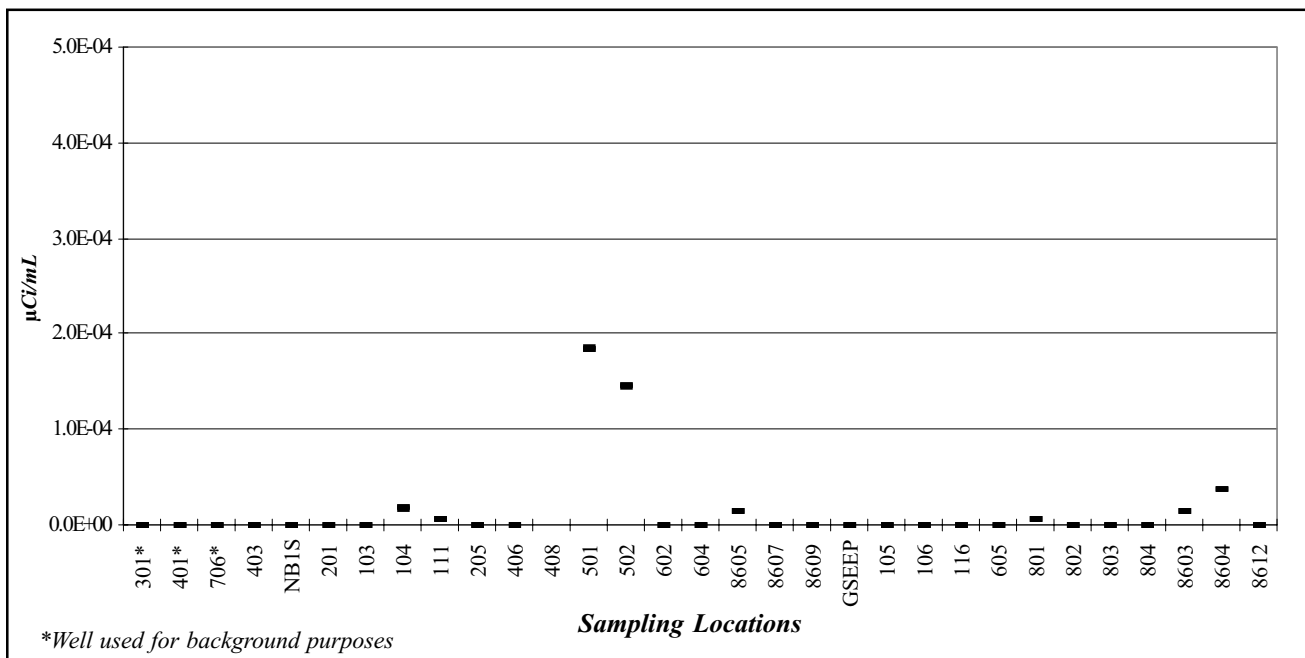
Figure E-4. Gross Beta ( \mu\text{Ci/mL} ) in Groundwater Samples from the Sand and Gravel Unit (Fig. E-4a follows with magnified scale.)
