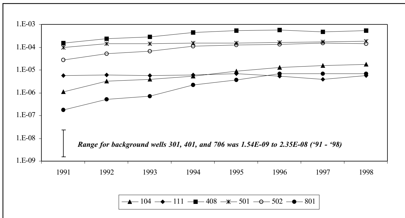
Figure 3-5. Eight-Year Trends of Averaged Gross Beta Activity (µCi/mL) at Selected Locations in the Sand and Gravel Unit
