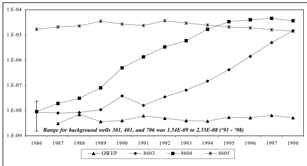
Figure 3-6. Thirteen-Year Trends of Averaged Gross Beta Activity (µCi/mL) at Selected Locations in the Sand and Gravel Unit
