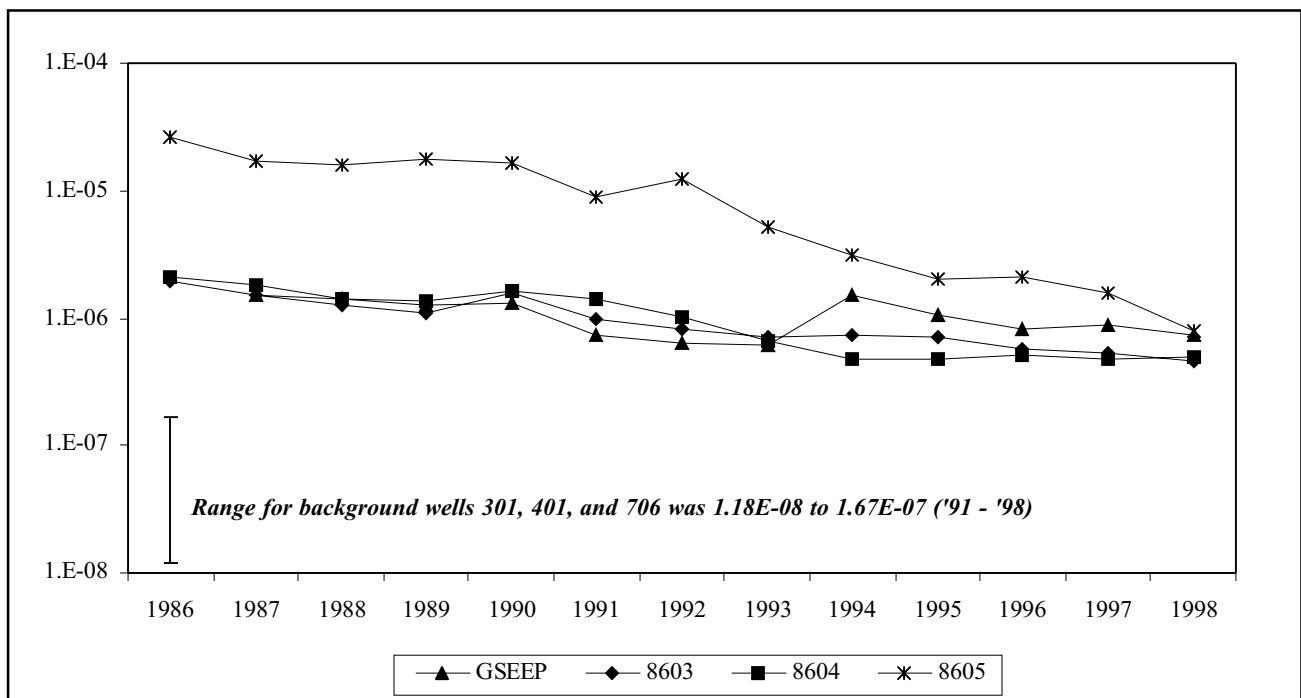
Figure 3-8. Thirteen-Year Trends of Averaged Tritium Activity ( \mu\text{Ci/mL} ) at Selected Locations in the Sand and Gravel Unit
