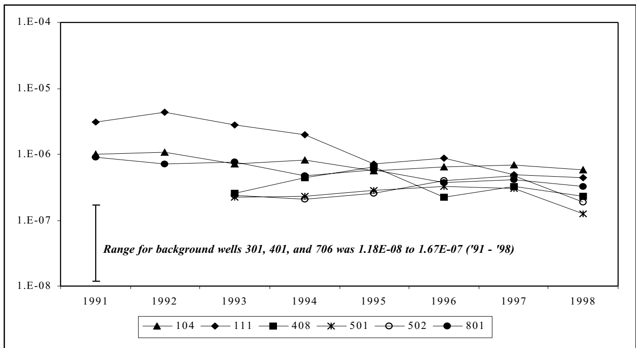
Figure 3-7. Eight-Year Trends of Averaged Tritium Activity ( \mu\text{Ci/mL} ) at Selected Locations in the Sand and Gravel Unit
