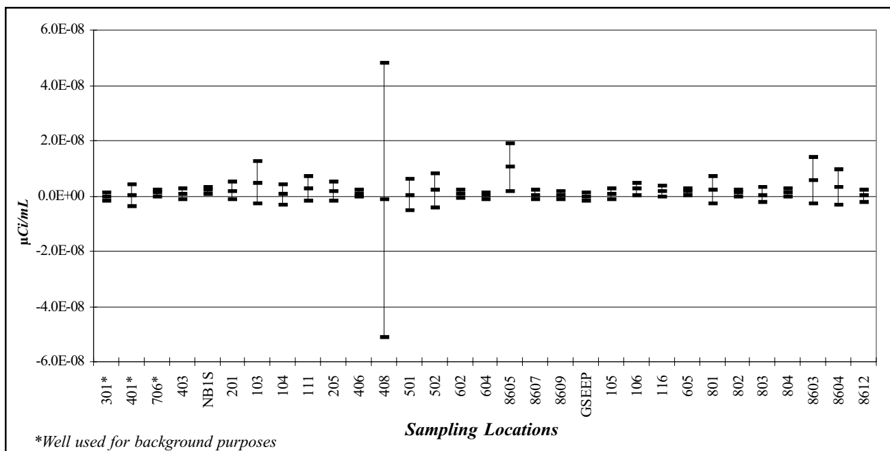
Figure E-3. Gross Alpha ( \mu\text{Ci/mL} ) in Groundwater Samples from the Sand and Gravel Unit (Fig. E-3a follows with magnified scale.)
