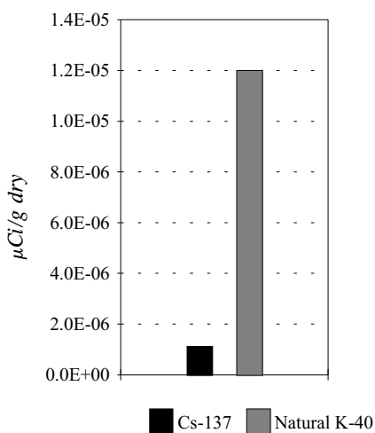
Figure 2-5. Comparison of Cesium-137 with Naturally Occurring Potassium-40 Concentrations in 1998 at Downstream Sampling Location SFTCESED
