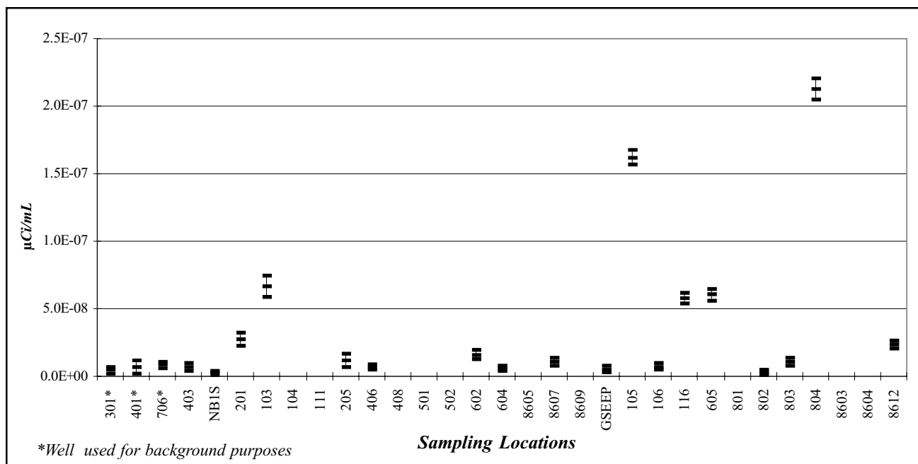
Figure E-4b. Gross Beta (μCi/mL) in Groundwater Samples from the Sand and Gravel Unit (magnified scale of Fig. E-4a)*
