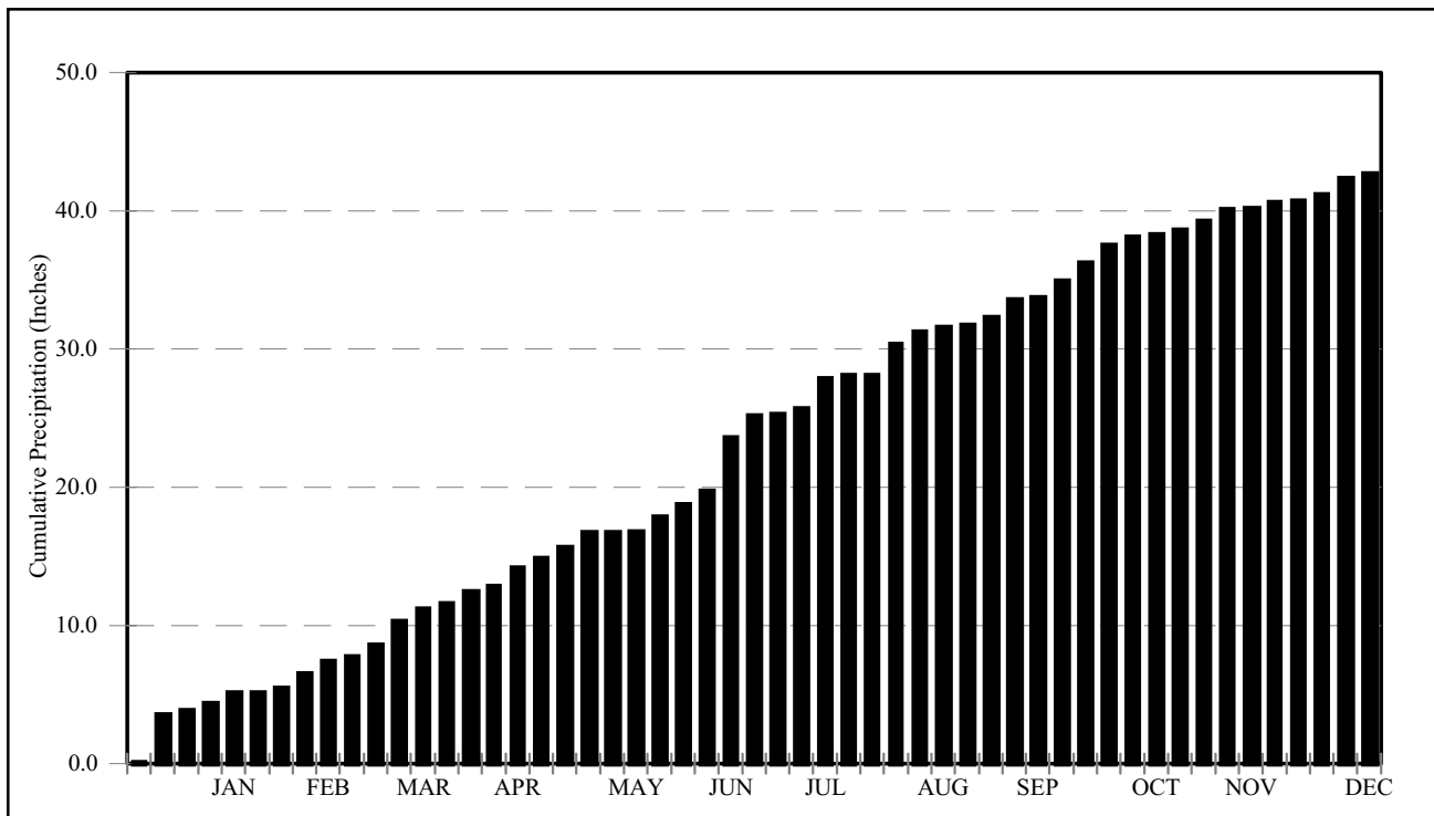
Figure I - 5. 1998 Cumulative Precipitation
