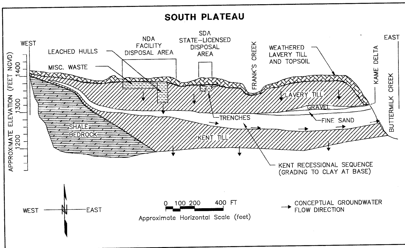
Figure 3-2. Geologic Cross Section through the South Plateau
