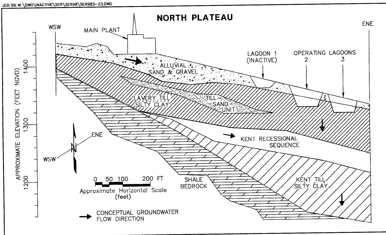
Figure 3-1. Geologic Cross Section through the North Plateau
