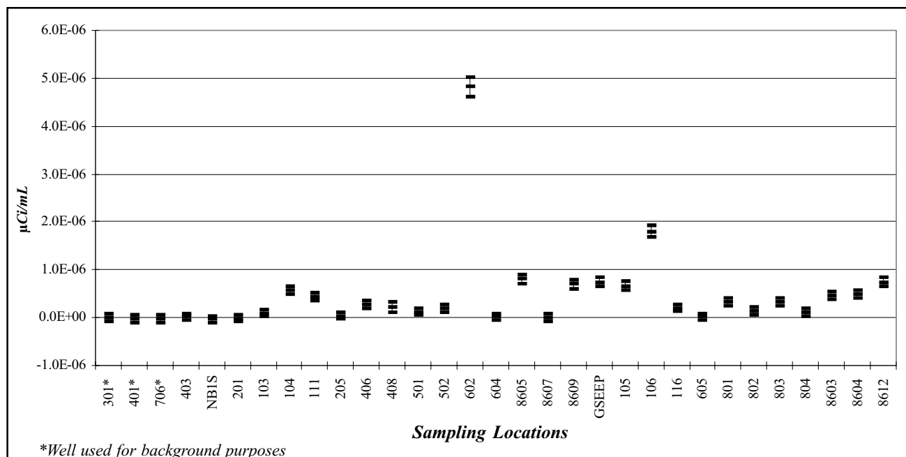
Figure E-5. Tritium Activity (μCi/mL) in Groundwater Samples from the Sand and Gravel Unit (Fig. E-5a follows with magnified scale.)
