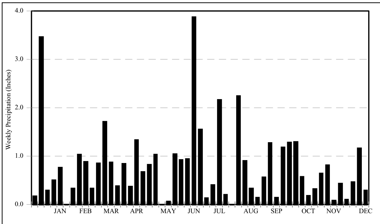
Figure I - 4. 1998 Weekly Precipitation
