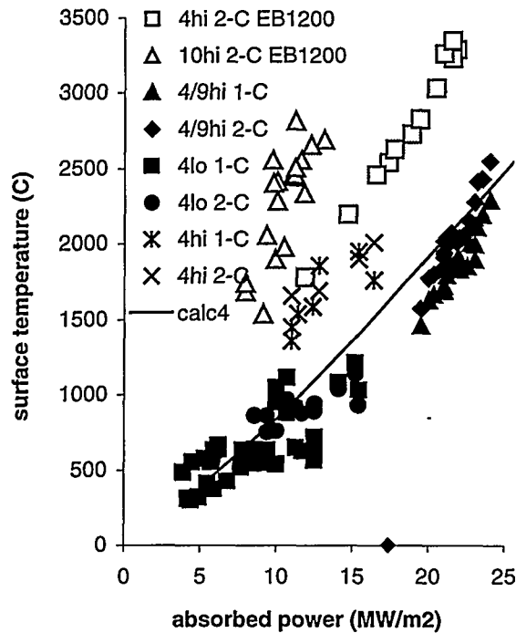
Fig.2. EB1200 and EBTS data on PW4, 9 and 10 and 1-D thermal model. EB1200 data are large open triangles and squares. "4lo 1-C" refers to PW4 and a one color low temperature pyrometer
