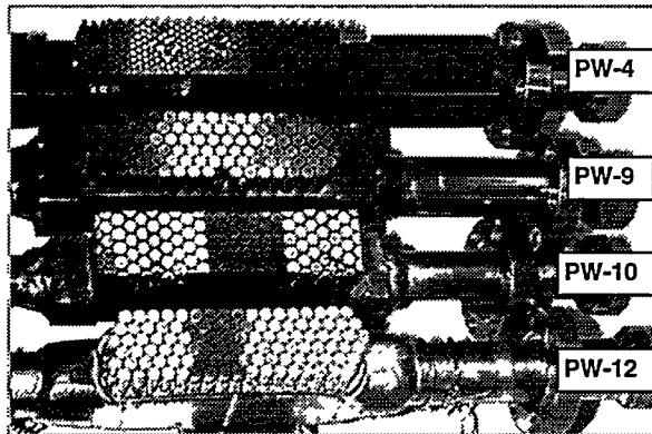
Fig.1. W-armored mockups after testing in EBTS.
