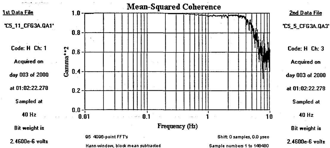
Figure 10 – Coherence Between Chaparral 5 Sensors
