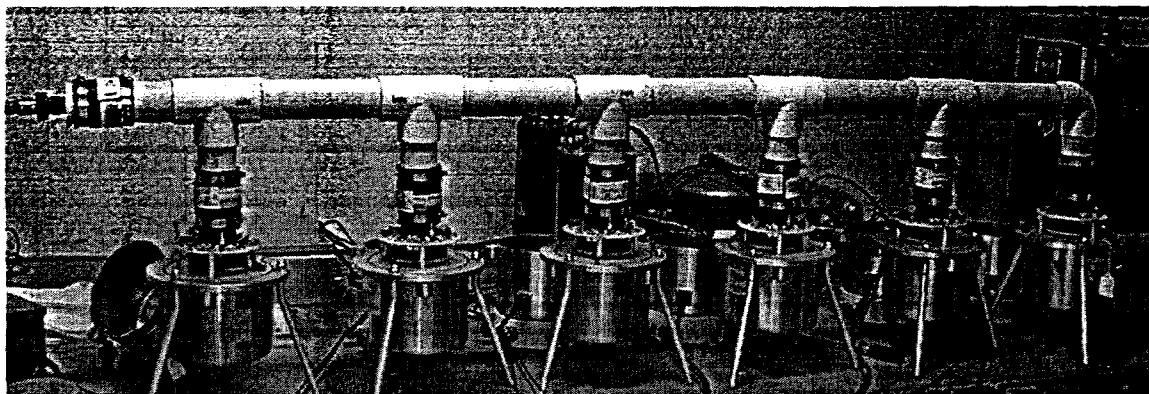
Figure 2 – Reference Sensor (left) and Five IS-59 Acoustically Paralleled Chaparral 5 Production Sensors
