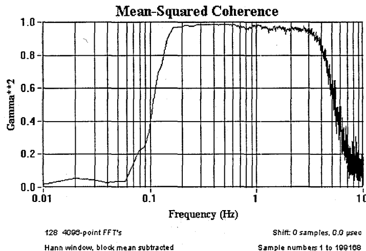
Figure 7 – Coherence Between Chaparral 5 and MB2000 Sensors
