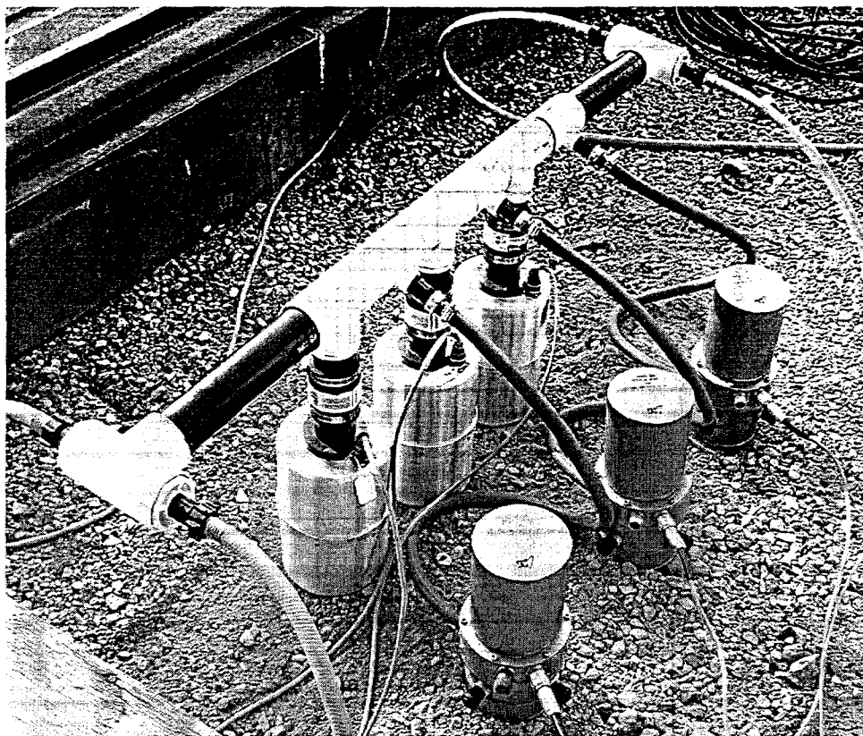
Figure 4 – MB2000 and Chaparral 5 Comparison Test at Sandia FACT Site
