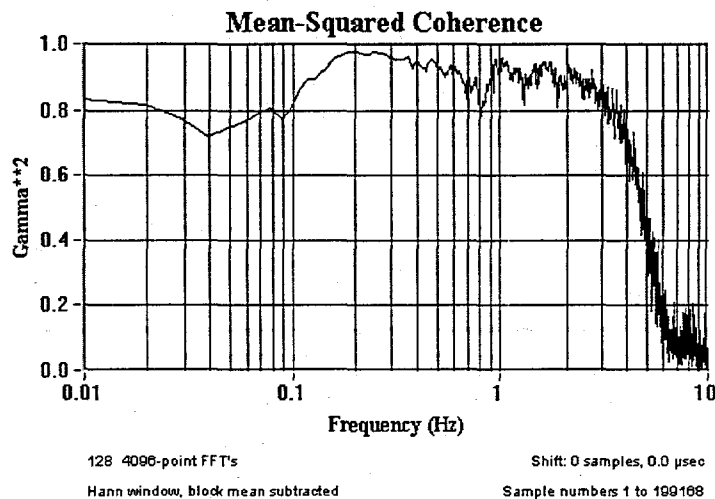
Figure 6 – Coherence Between Chaparral 5 Sensors
