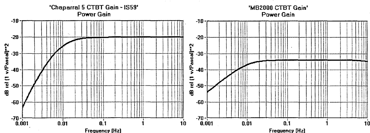
Figure 3 - IS-59 Chaparral 5 Sensor Power Gain and CEA CTBT MB2000 Power Gain
