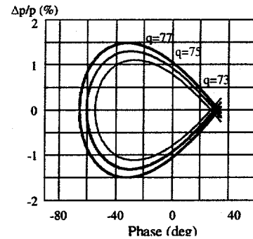
Figure 3: Separatrices in the longitudinal phase space for charge states 73, 75 and 77 of uranium beam.
