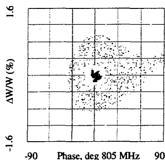
Figure 6: Phase space plots of multi-Q beam at the location of the second stripper. Blue dots represent the acceptance of high-energy section.
