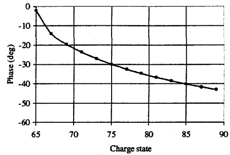
Figure 2: Synchronous phase as a function of uranium ion charge state. The designed synchronous phase is -30^\circ for q_0=75 .
