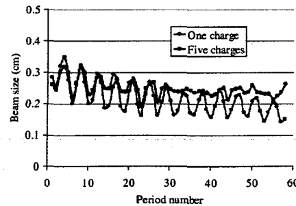
Figure 4: Transverse beam envelopes for one charge state beam (blue dots) and 5 charge state beam (magenta dots). Input beam is mismatched by a factor 1.4.
