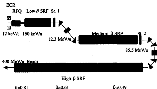
Figure 1: General design of the Linac.
