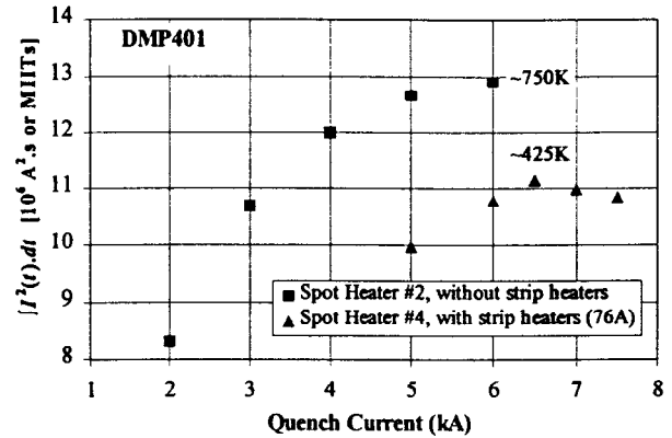
Figure 9: Measurements of quench temperatures in the magnet. Using the strip heaters as designed, the maximum temperature measured is an acceptable 425 K.
