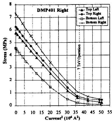
Figure 3: Stress vs. current in the right aperture. Four independent strain gauges measure the coil stress at a particular axial location. The behavior is as expected.
