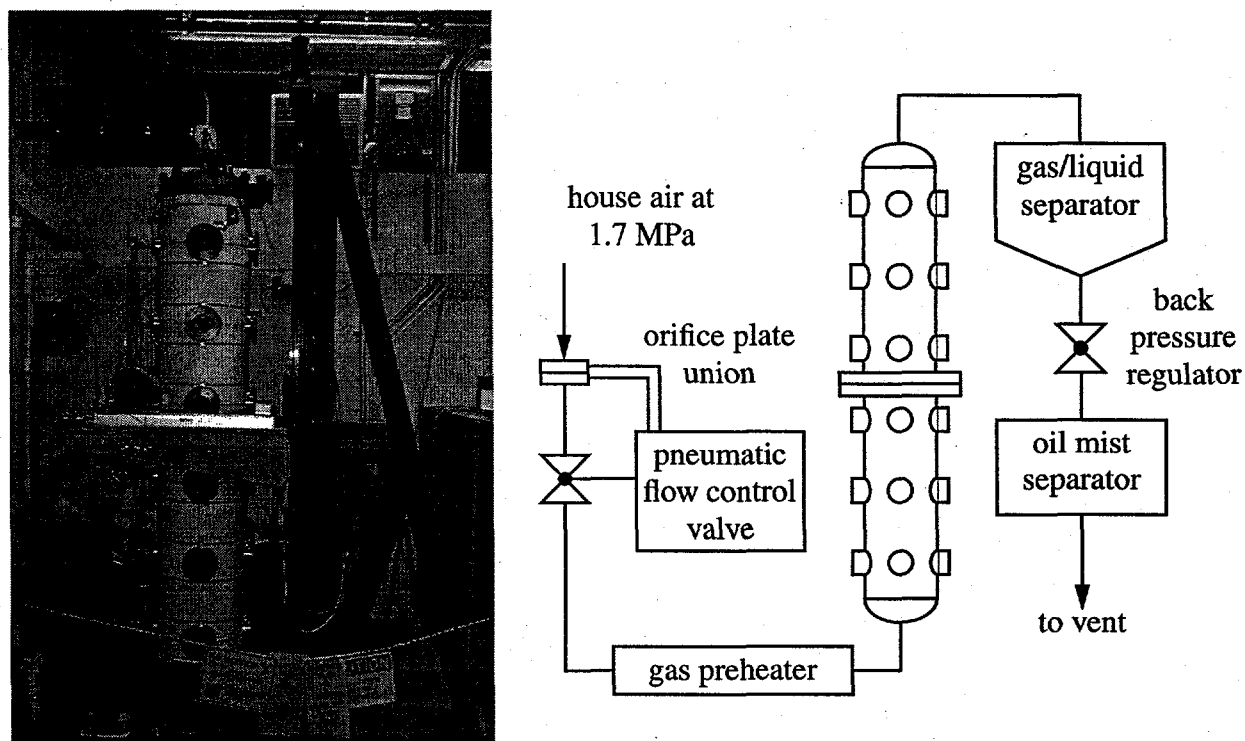
Figure 2. Picture and schematic of the slurry bubble-column reactor (SBCR). In the picture the vertical traverse is to the right of the column; the source and its horizontal traverse are in front.
