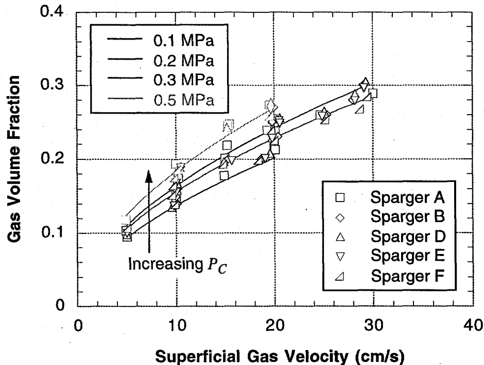
Figure 17. Fully-developed average gas volume fraction as a function of superficial gas velocity and column pressure for all spargers tested.
