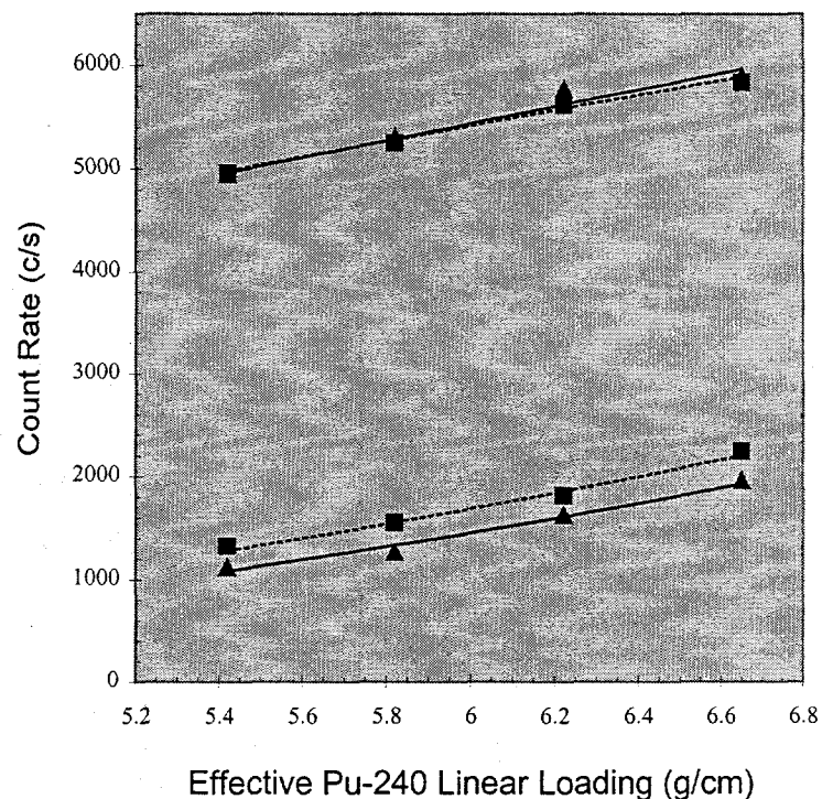
Fig. 4. Comparison of MCNP-REN simulation ( \blacktriangle ) and the experimental measurement ( \blacksquare ) of mixed oxide fresh fuel using the UWCC. Count rates greater than 4000 counts/s were obtained in unborated water while those below this were obtained in borated water (2250 mg/l of boron). The experimental boron concentrations actually achieved were most probably less than 2250 mg/l used in the calculation owing to the solubility limit of Borax being locally exceeded. Borax precipitation was observed in the tank.
