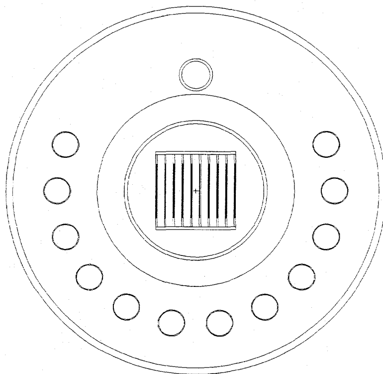
Fig. 5. Horizontal slice through the RRFC with an IAN-R1 fuel assembly centered in the detector. The slice shows the 12 detector tubes as well as the position of one of the AmLi sources located at the top of the image.
