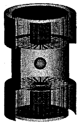
Z-Pinch-Driven Hohlraum
