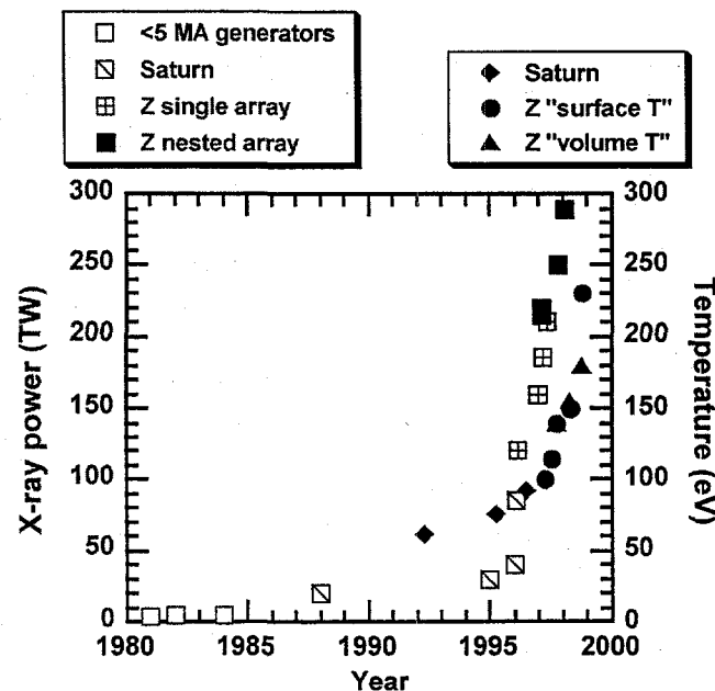
Figure 1. Increase in radiated x-ray power and radiation temperature vs. year
