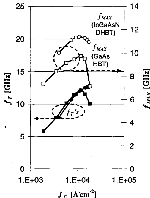
Figure 5 : The f_T and f_{\text{MAX}} of the GaAs/InGaAsN/GaAs P-n-P HBT, and of the AlGaAs/GaAs P-n-p HBT.
