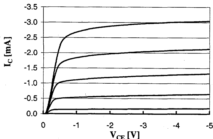
Figure 4 : The common emitter IV characteristics of the 3 \times 25 \mu\text{m}^2 P-n-P GaAs/InGaAsN/GaAs HBT. The base current varies from 20 \mu\text{A} to 100 \mu\text{A} at 20 \mu\text{A}/\text{step} .
