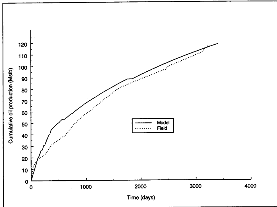
Figure 7: Comparison of oil cumulative production in Malnar Pike with the modified model predictions
