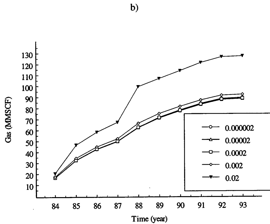
Figure 4: Effect of fracture porosity on cumulative production from Michelle Ute well: a) oil, b) gas.
