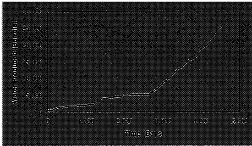
Figure 10: Water produced from the Michele-Ute; observe the sharp transition at around 2700 days.
