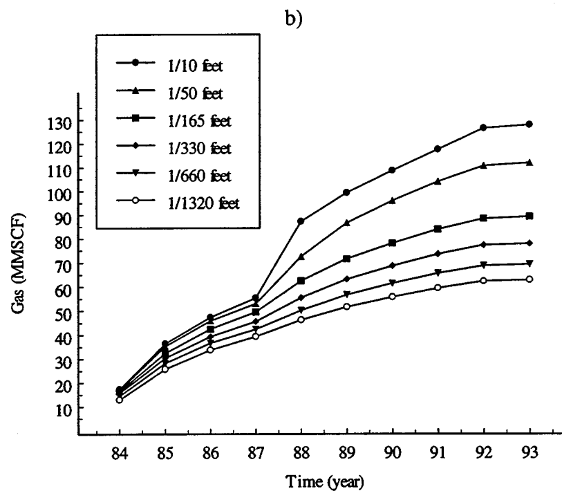
Figure 5: Effect of fracture frequency on cumulative production for Michelle Ute well: a) oil, b) gas.
