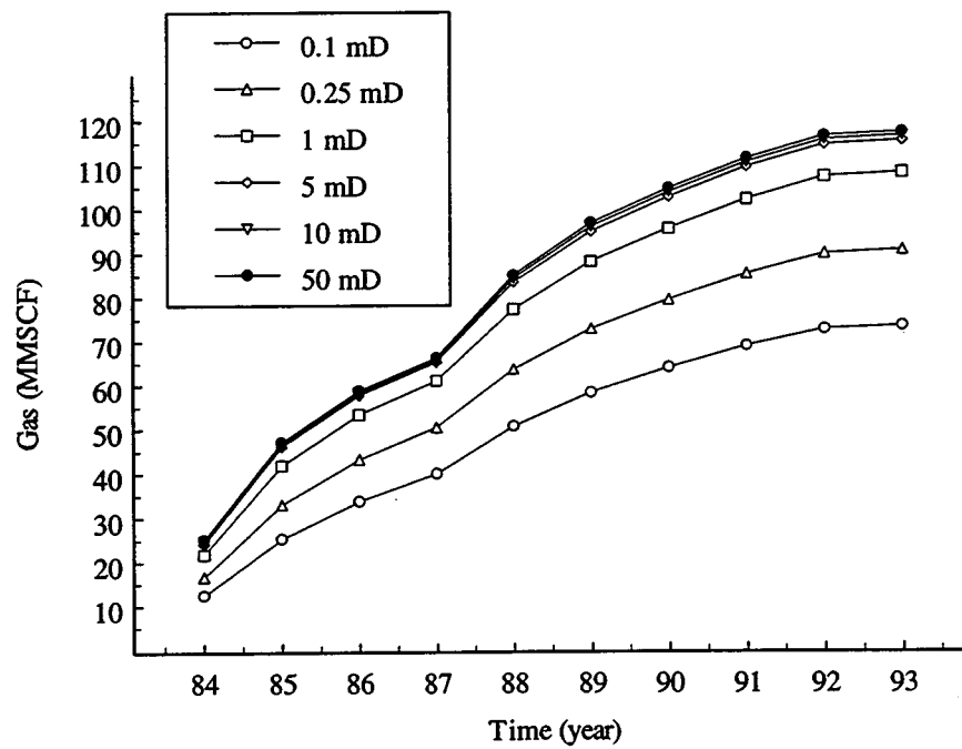
Figure 6: Effect of permeability on cumulative production from Michelle Ute well: a) oil, b) gas.
