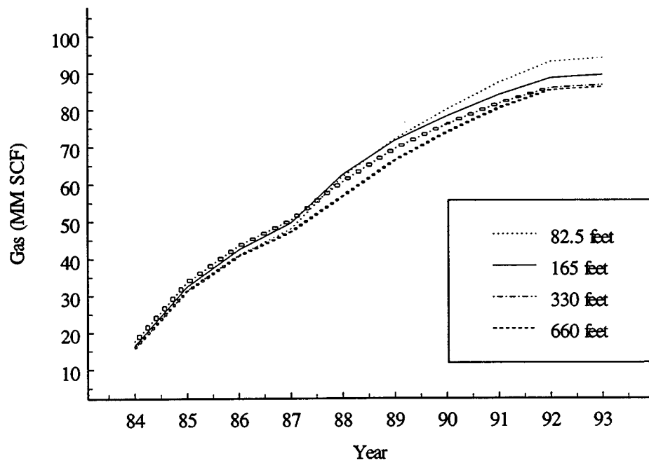
Figure3: Effect of block size on cumulative production for Michelle Ute well: a) oil, b) gas.
