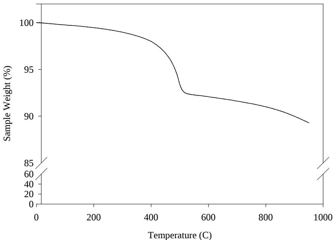
Figure 1. Thermal gravimetric analysis (TGA) of 80% waste load PET 99-2 sample.
