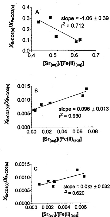
Fig. 4. Partitioning of Sr into carbonate minerals formed during HFO reduction in Ca-free 1 mM (A), 0.1 mM (B) and 0.01 mM (C) \Sigma Sr cultures.
