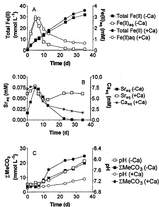
Fig. 2. HFO reduction (A), aqueous [Sr] & [Ca] (B), and pH & solid-phase inorganic carbon ( \Sigma MeCO 3 ) concentration in 0.1 mM \Sigma Sr cultures.
