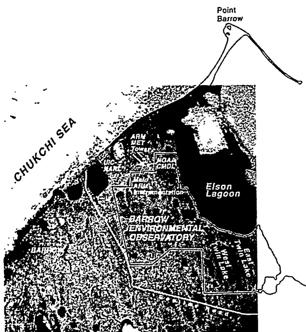
Figure 2. Aerial view of the Barrow region, showing the locations of the ARM and NOAA instrumentation relative to the BEO and the UIC-(former) NARL. (For a color version of the figure, please see http://www.arm.gov/docs/documents/technical/conf_9803/zak-98.pdf .)
