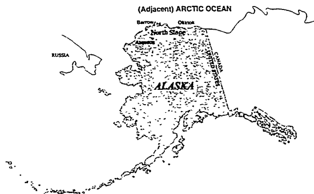
Figure 1. Location of the Barrow ARM NSA/AAO facility. Atkasuk and Olinok are other locations within the ARM NSA/AAO locale where additional ARM instrumentation may eventually be located.
