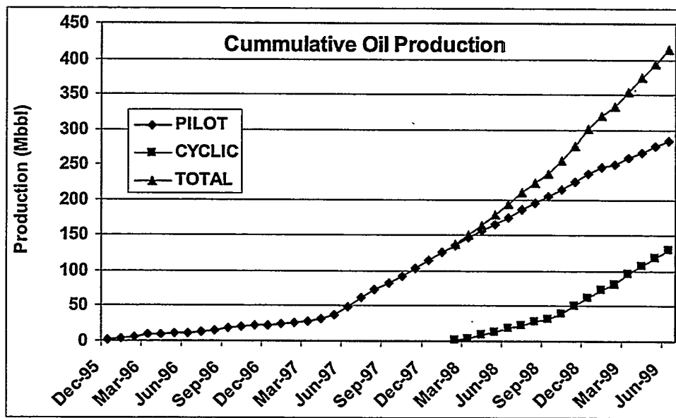
Figure 1-2: Cummulative oil production from the Pru Fee property since the start of the DOE oil technology demonstration in late 1995. The steam flood pilot was initiated in mid-1997 and the "300-series" cyclic wells were put online early in 1998.
