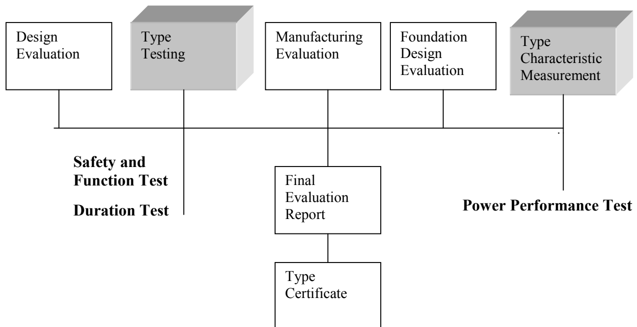
FIGURE 2. TESTS REQUIRED FOR SMALL WIND TURBINE CERTIFICATION
