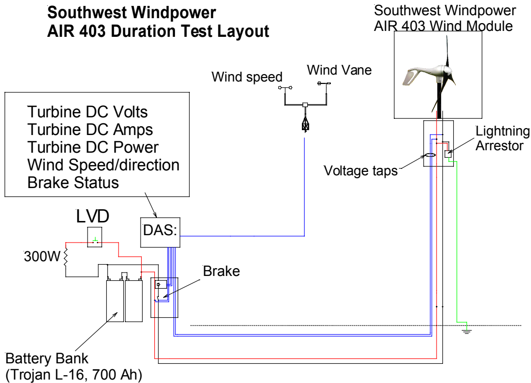
FIGURE 3. AIR 403 DURATION TEST SCHEMATIC
