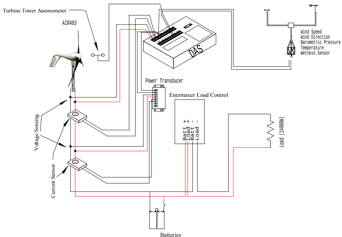
FIGURE 4. TURBINE CONFIGURATION FOR POWER PERFORMANCE TEST
