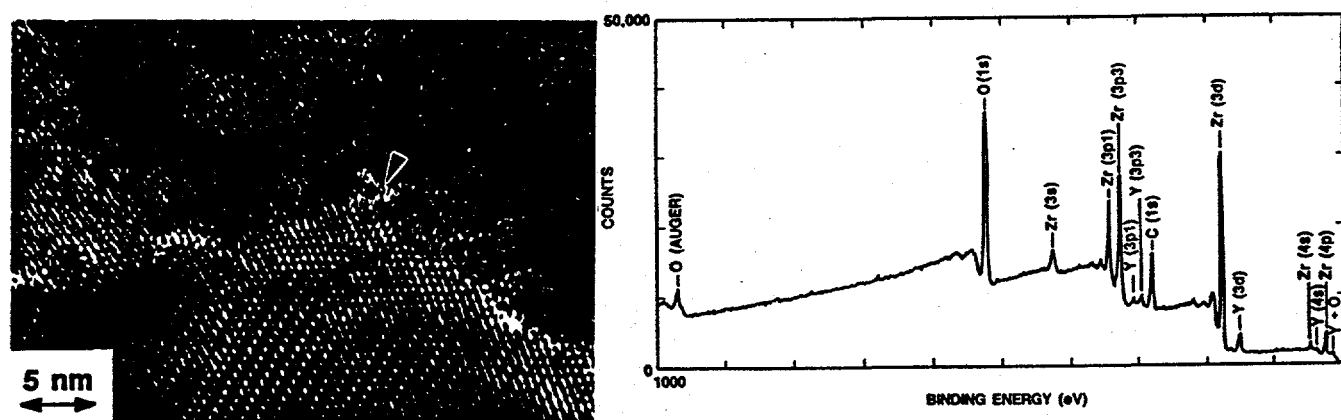
Fig. 4 (left) High resolution lattice image of a grain boundary triple junction in fine-grained superplastic YTZP, and (right) XPS spectrum from the fracture surface of a superplastic YTZP sample, indicating the absence of any second phase. (from Ref. [36])
