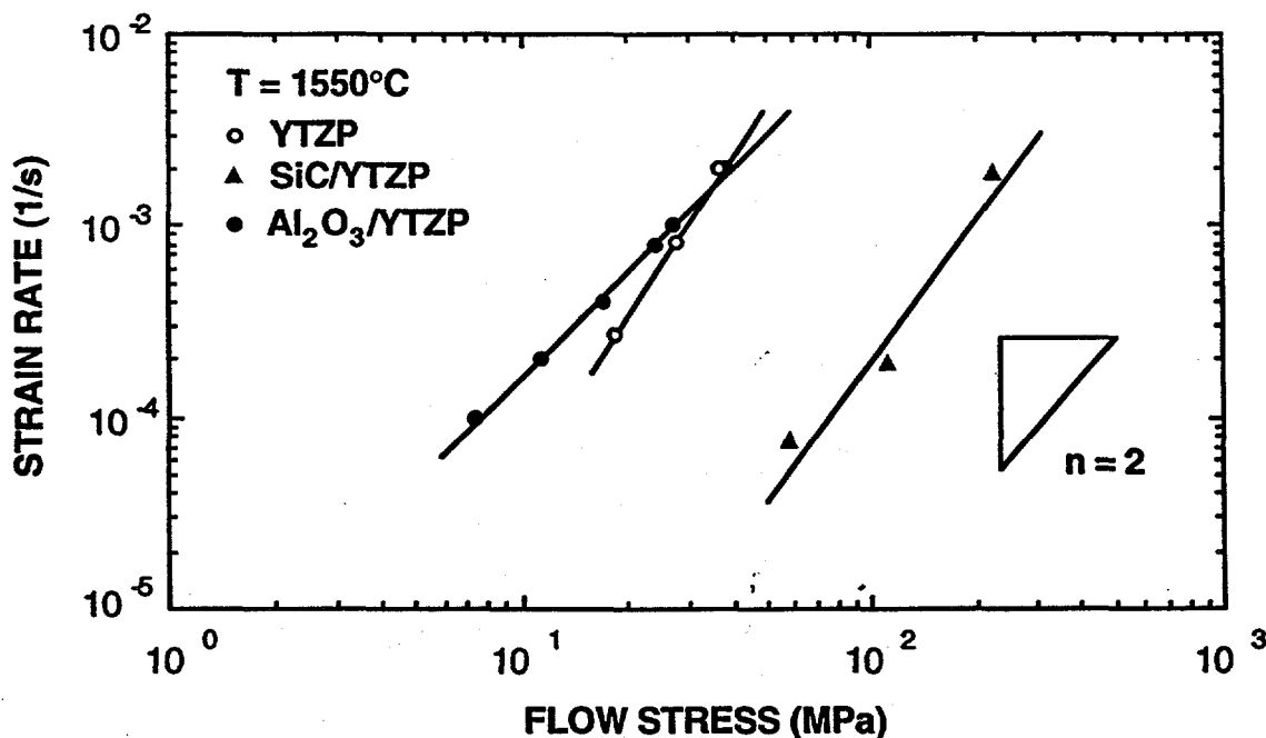
Fig. 3 Direct comparison of the strengths of YTZP and SiC/YTZP and \text{Al}_2\text{O}_3/\text{YTZP} composites at 1550^\circ\text{C} . (from Ref. [35])
