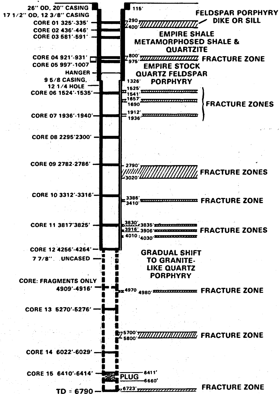
Fig. 2. Casing, coring, and formation data, well No. 1
