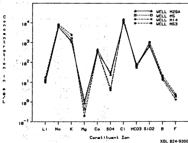
Figure 2b. Schoeller diagram for producing wells located along an E-W section.
