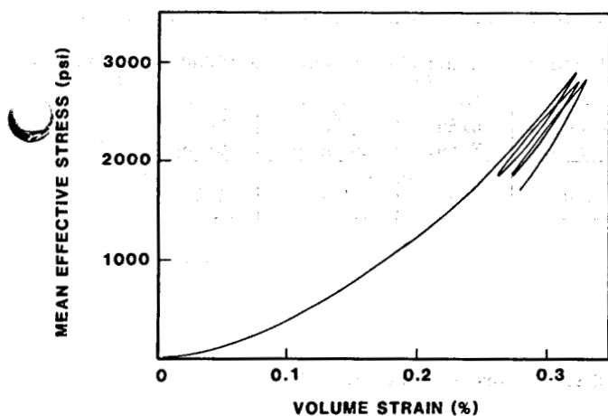
Figure 4. Basic pore pressure cycling test on Cerro Prieto core from Well M-107, depth 6,936 ft, initial porosity 18.6%.
