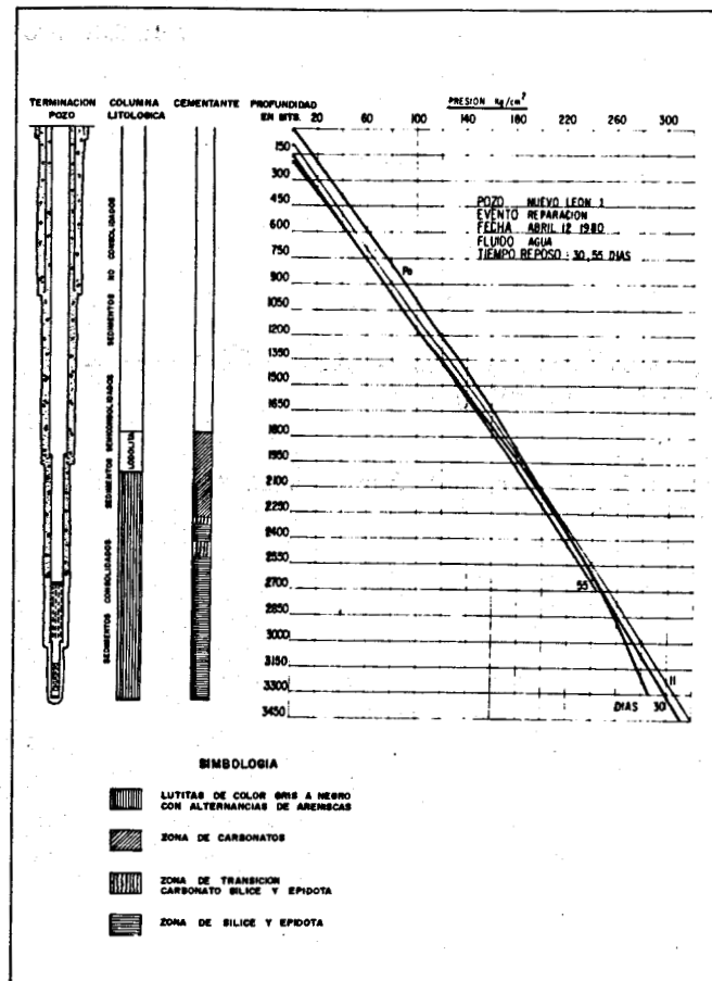
Figure 7. Pressure logs of well Nuevo León 1 after undergoing repairs.
