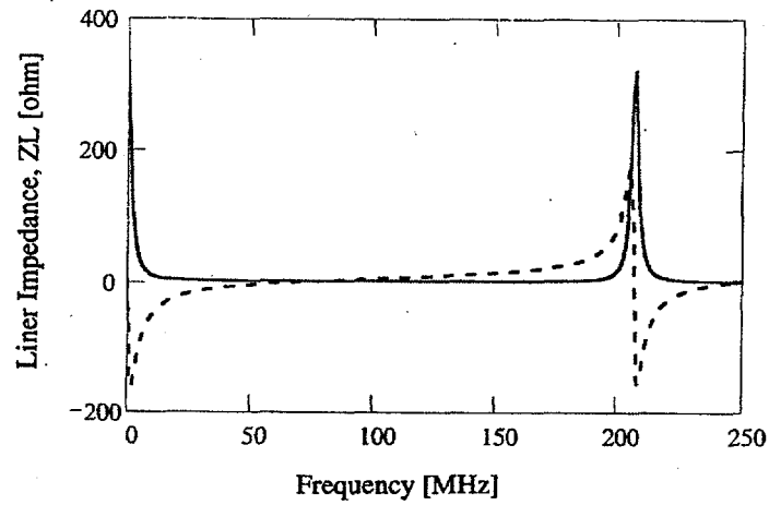
Figure 2: Impedance of the liner. Solid — ReZ_L[\text{Ohm}] . Dashed — ImZ_L[\text{ohm}] .
