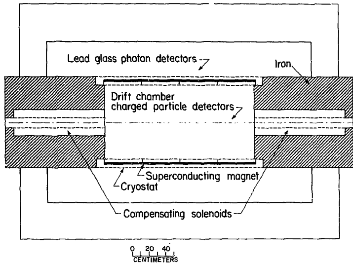
Fig. 3 Continuous Thin Superconducting Solenoid Magnet
