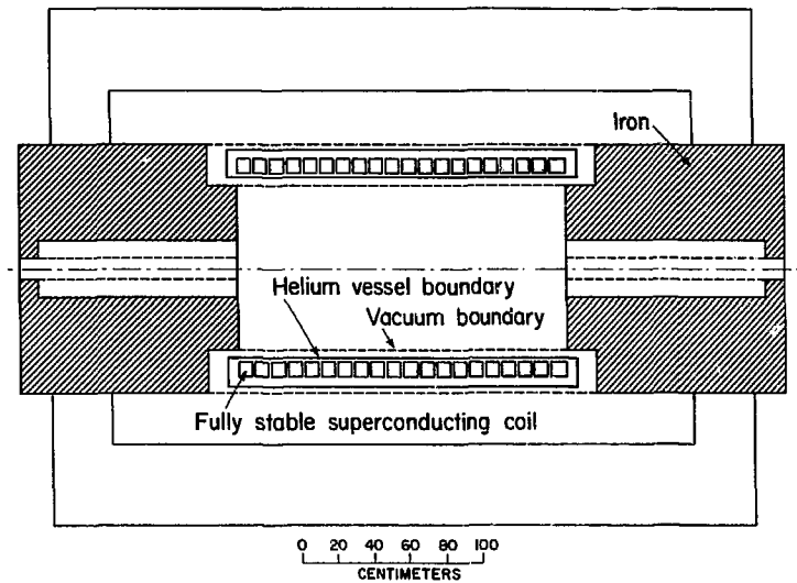
Fig. 2 Conventional Superconducting Solenoid Magnet
