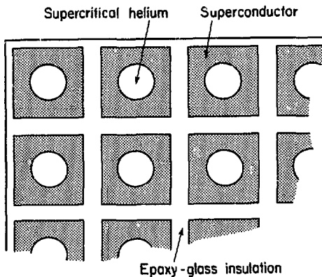
b. Tubular Supercritical Helium Cooled Coil Configuration (like the OMEGA magnet coil)
