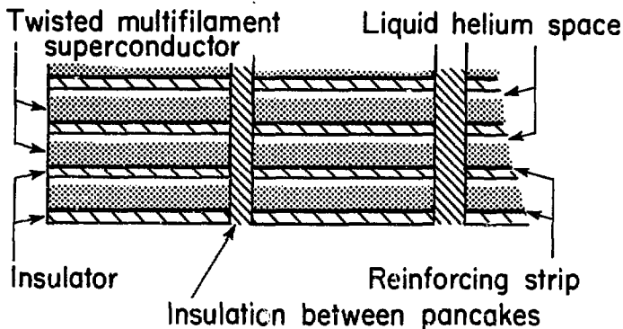
a. Bubble Chamber Coil Configuration
