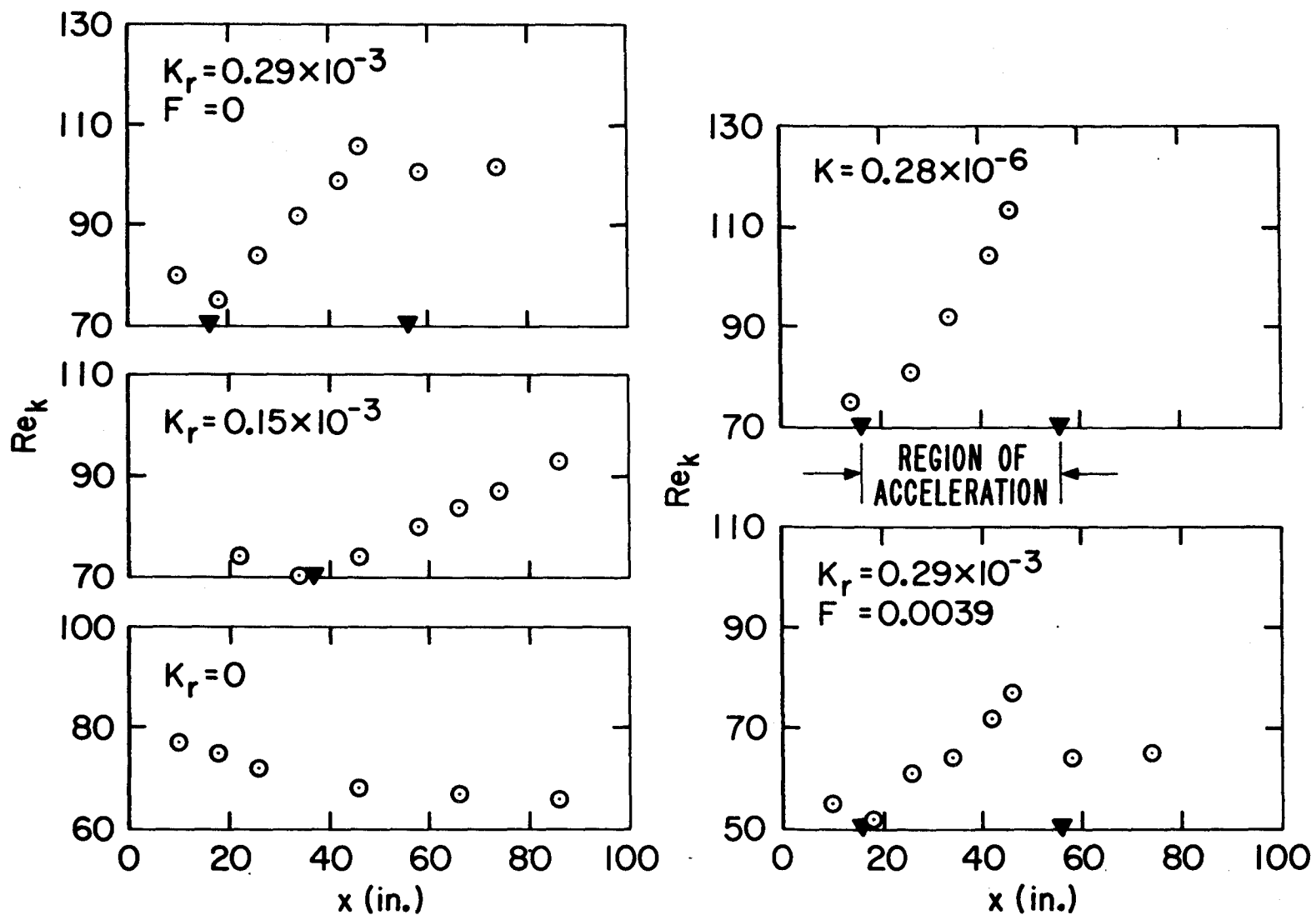
Figure 3-14. Roughness Reynolds Number Variation with Axial Distance
