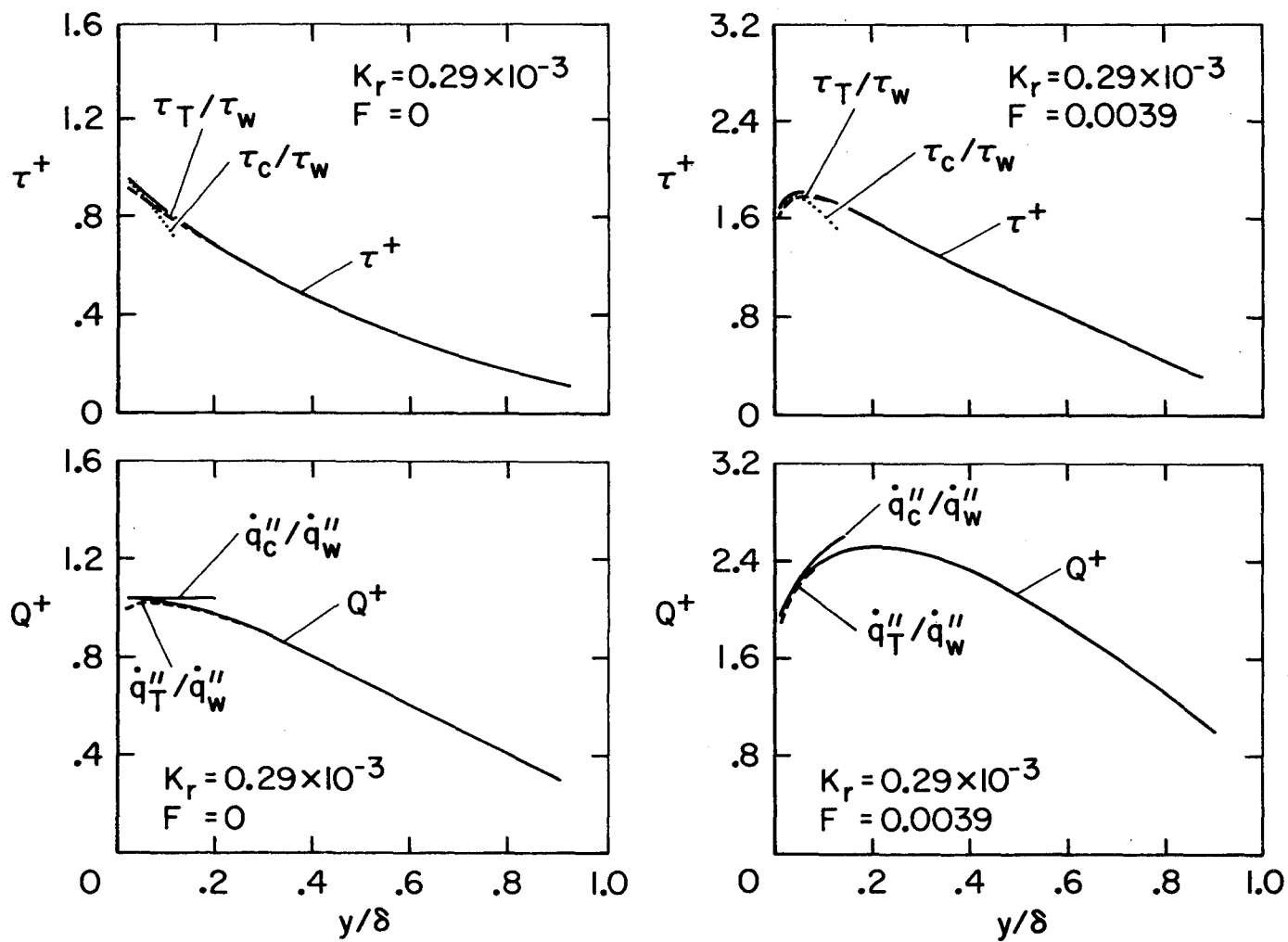
Figure 3-41. \tau^+ and Q^+ Distributions for the K_r = 0.29 \times 10^{-3} , F = 0 and F = 0.0039 Runs
