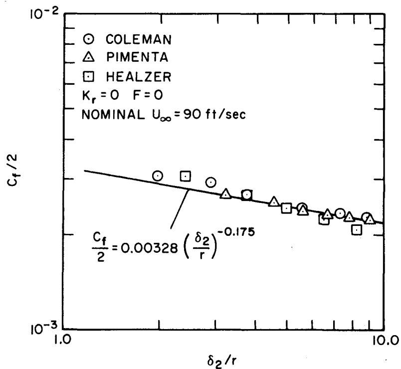
Figure 3-2. Zero Pressure Gradient Skin Friction Coefficient Data
