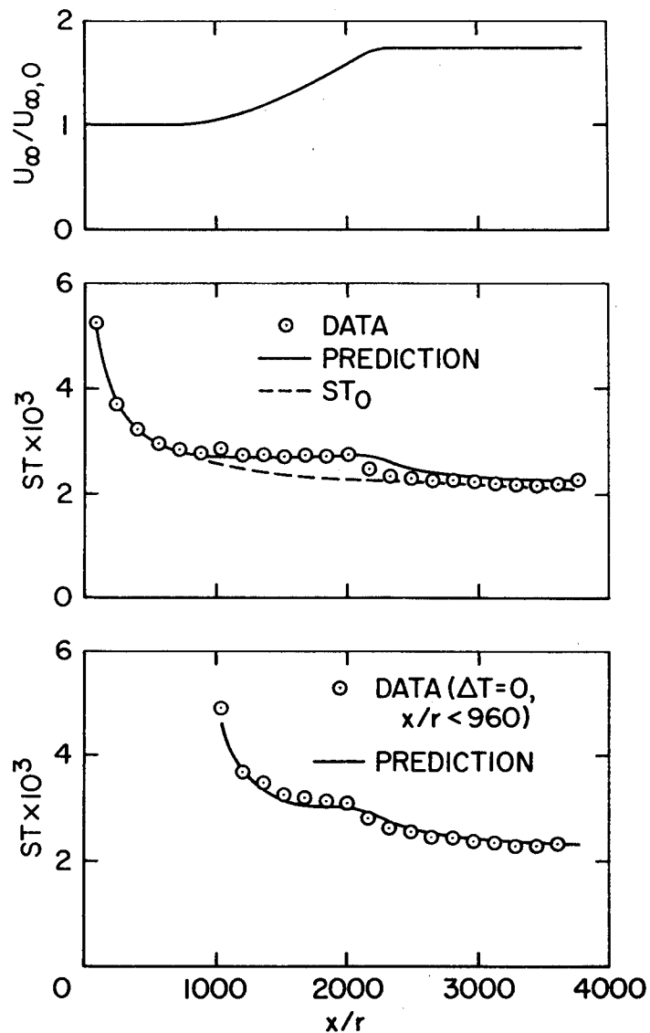
Figure 3-47. Comparison of St Data and Predictions for K = 0.28 \times 10^{-6} , F = 0 Run Both with and Without an Unheated Starting Length
