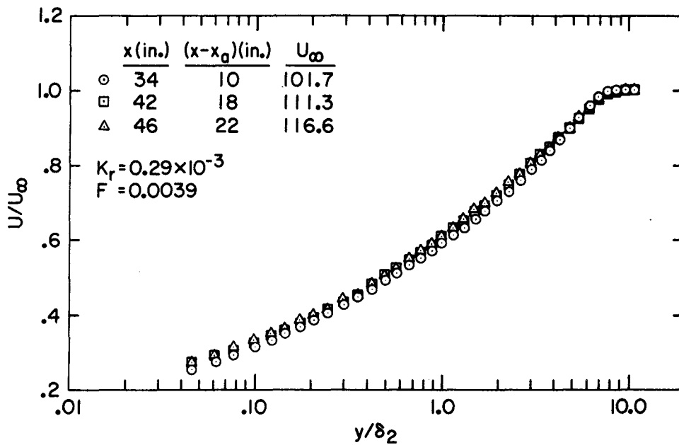
Figure 3-17. Mean Velocity Profiles Illustrating Similarity in Flow Direction ( K_r = 0.29 \times 10^{-3} , F = 0.0039 )
