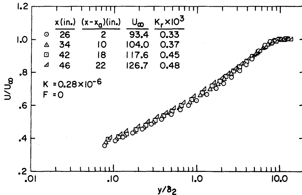
Figure 3-18. Mean Velocity Profiles Illustrating Lack of Similarity in Flow Direction ( K = 0.28 \times 10^{-6} )
