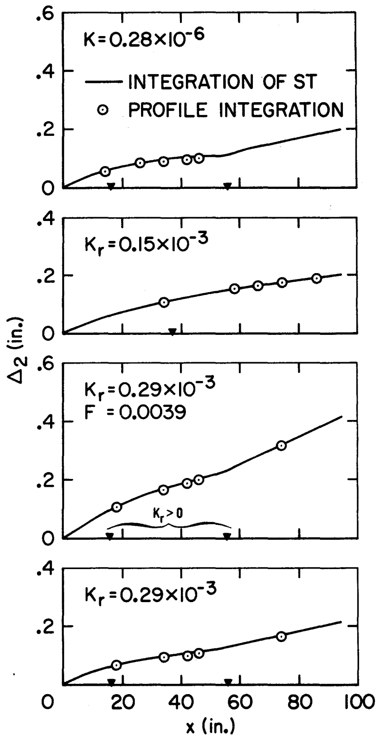
Figure 3-13. Enthalpy Thickness Variation with Axial Distance
