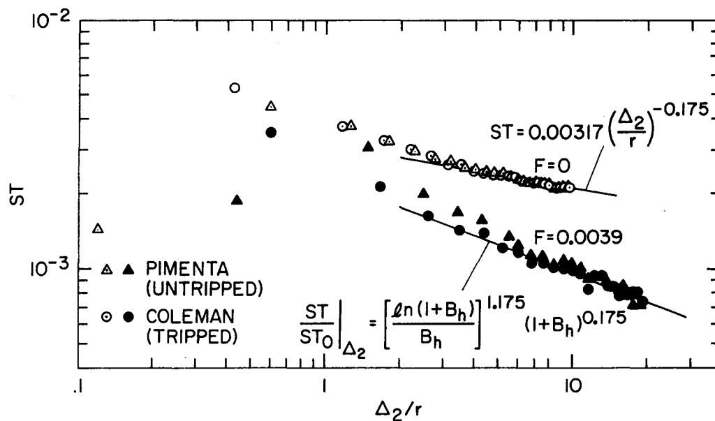
Figure 3-1. Zero Pressure Gradient Stanton Number Data
