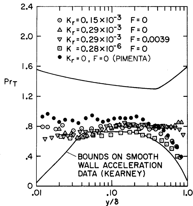
Figure 3-39. Turbulent Prandtl Number Distributions for the Acceleration Cases of the Present Study
