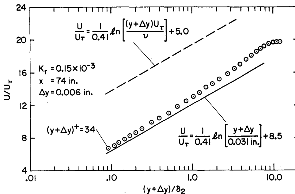
Figure 3-19. Mean Velocity Profile Plotted Using Shifted Wall Position ( K_r = 0.15 \times 10^{-3} )
