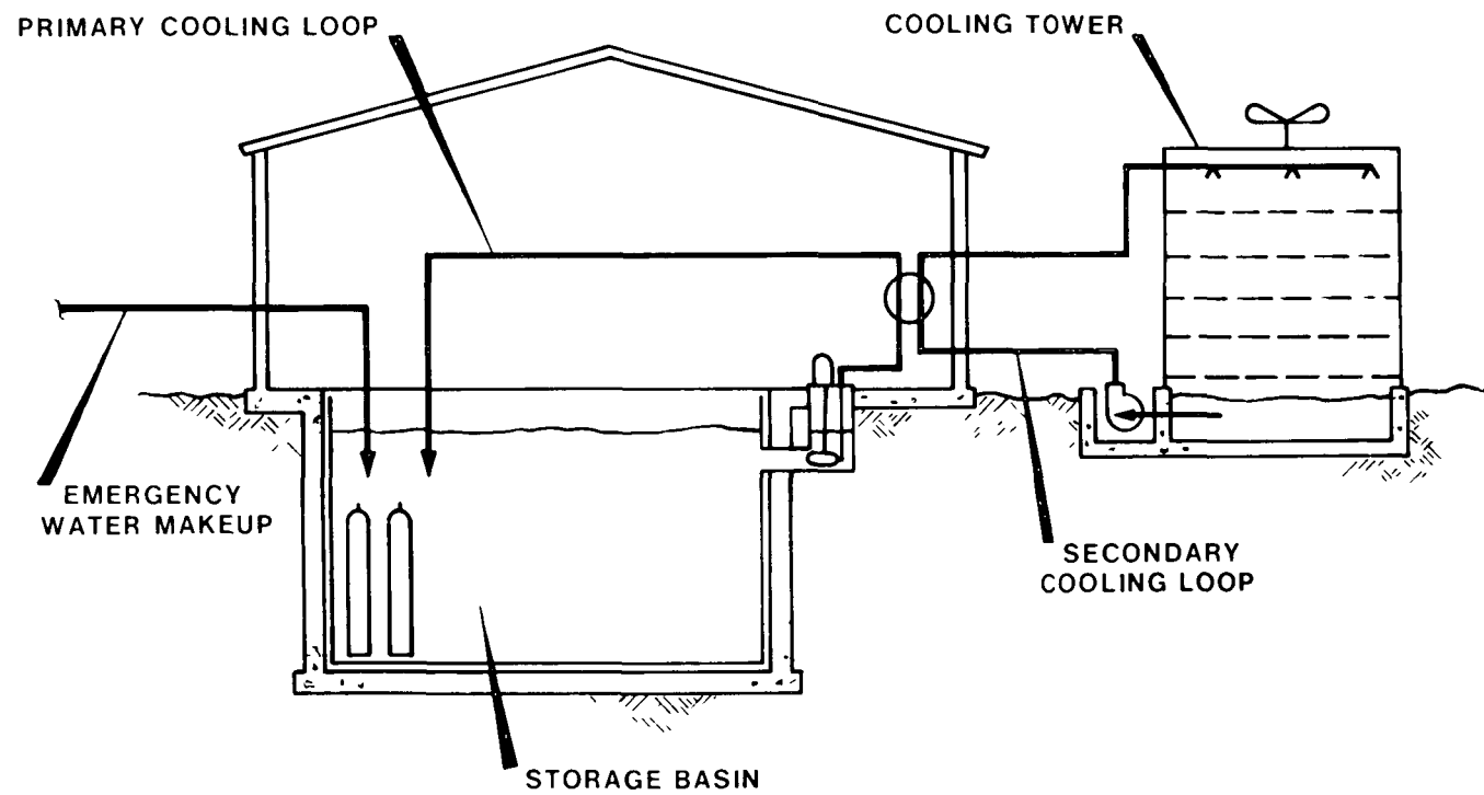
FIGURE 4.4 - HEAT REMOVAL SYSTEM; WATER BASIN CONCEPT
