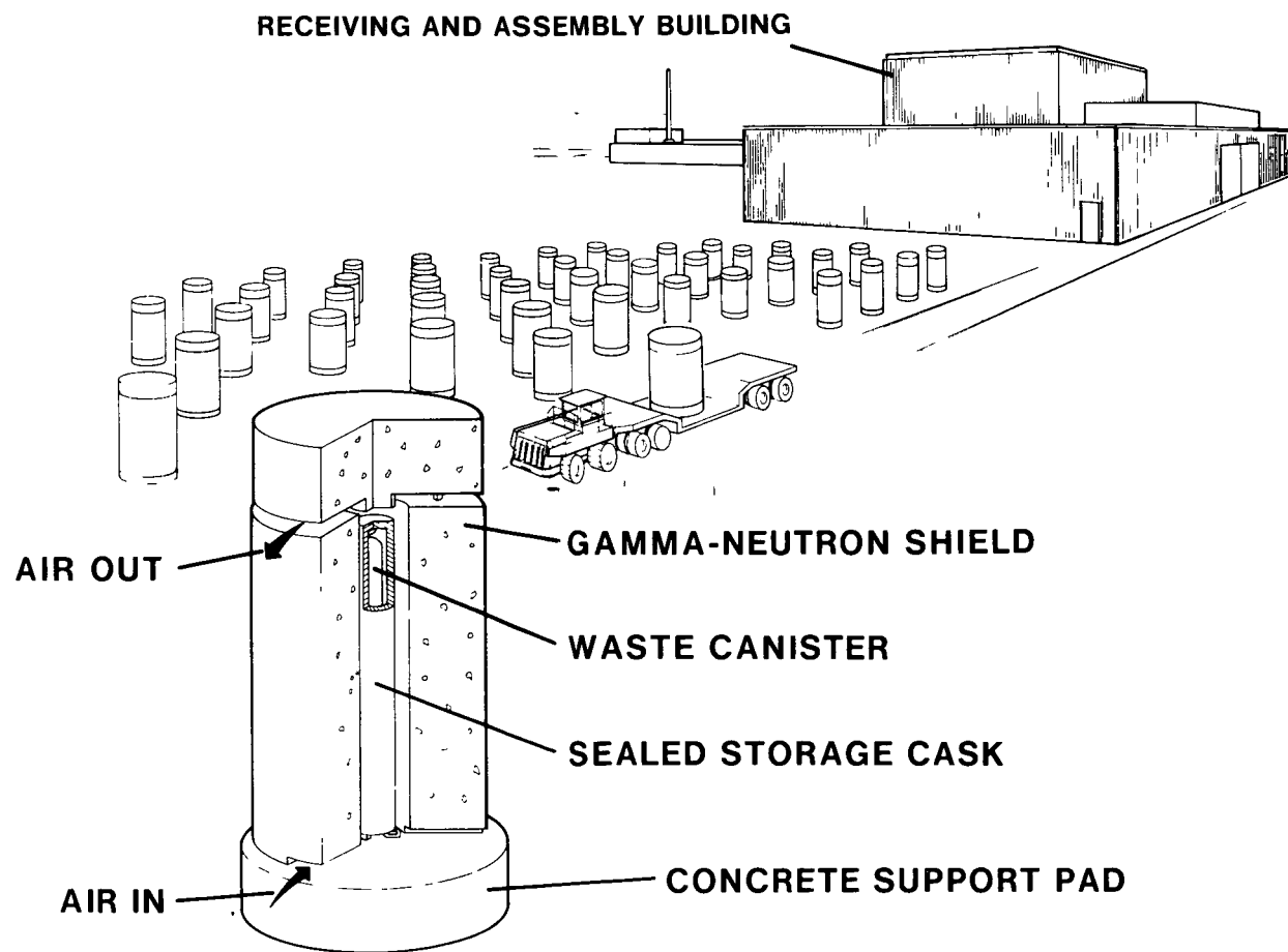
FIGURE 4.6 - RETRIEVABLE SURFACE STORAGE FACILITY (RSSF)
