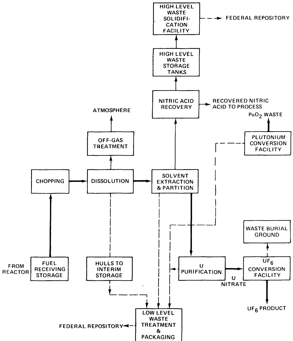
FIGURE 4.1 - FLOW DIAGRAM OF REPROCESSING PLANT (URANIUM-ONLY RECYCLE)
