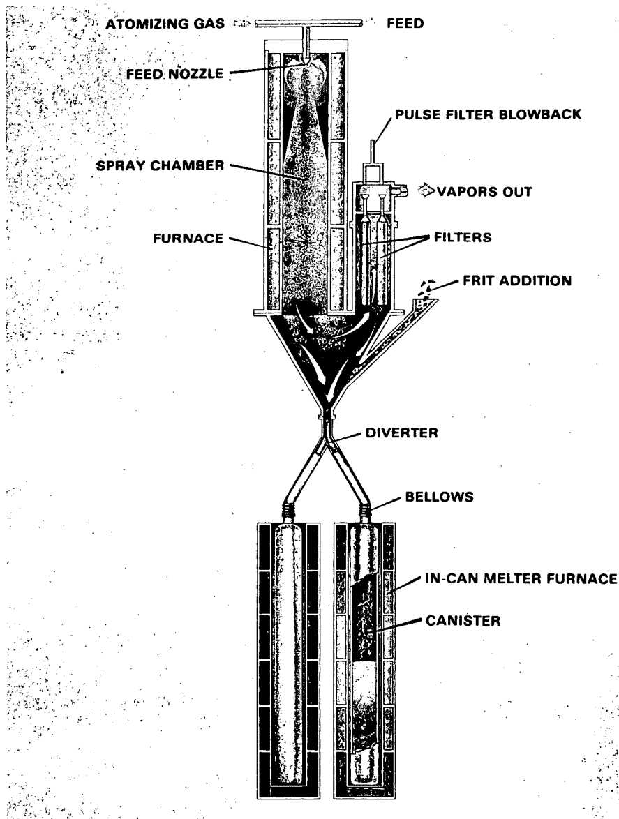
FIGURE 4.3 - SPRAY CALCINER/IN-CAN MELTER
