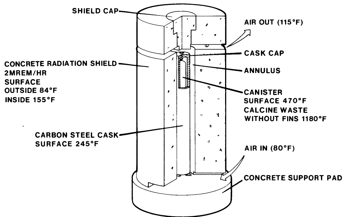
FIGURE 4.5 - SEALED STORAGE CASK CONCEPT (SSCC)
