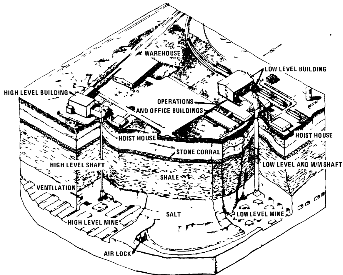
FIGURE 4.8 - PROBABLE LAYOUT OF BEDDED SALT REPOSITORY
