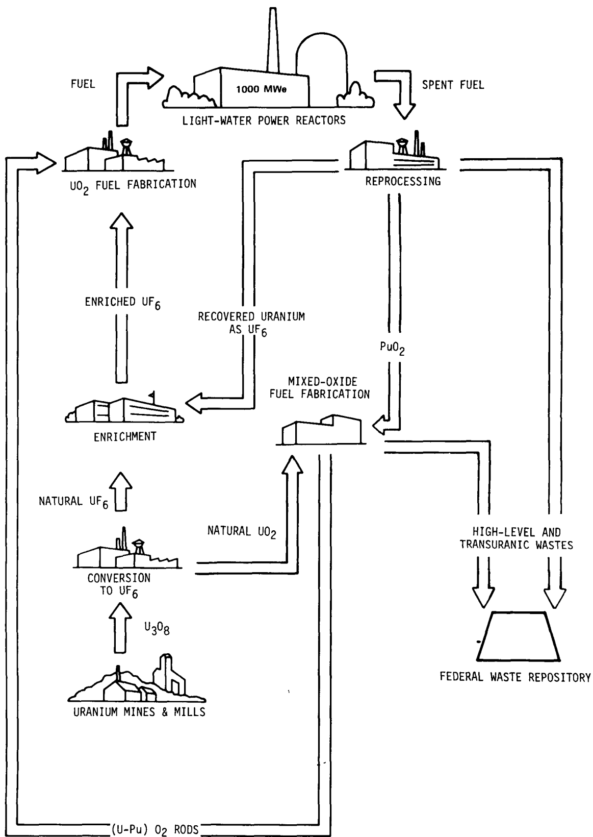
FIGURE 3.3 - URANIUM/PLUTONIUM RECYCLE
