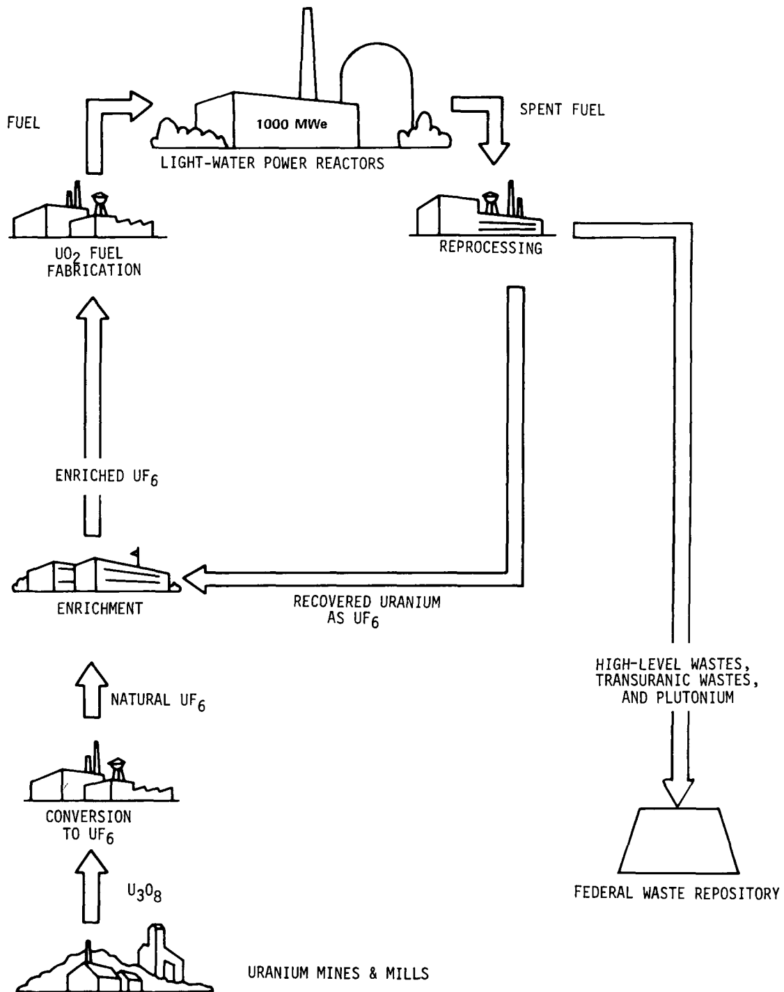
FIGURE 3.2 - URANIUM-ONLY RECYCLE
