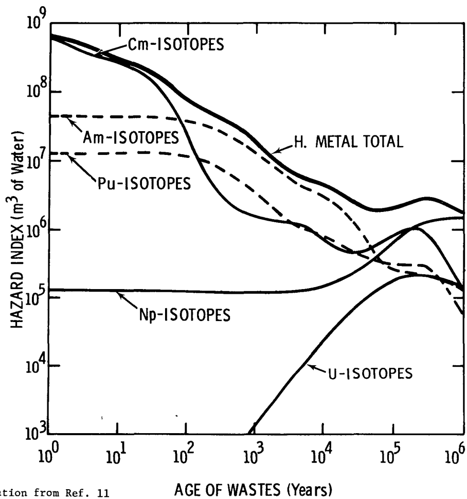
FIGURE 4.10 - HEAVY-METAL ISOTOPE HAZARDS FROM A 1000-MWE PWR (WASTES FROM 1 METRIC TON OF FUEL AT 34,000 \text{ MW}_{\text{TH D}} )
