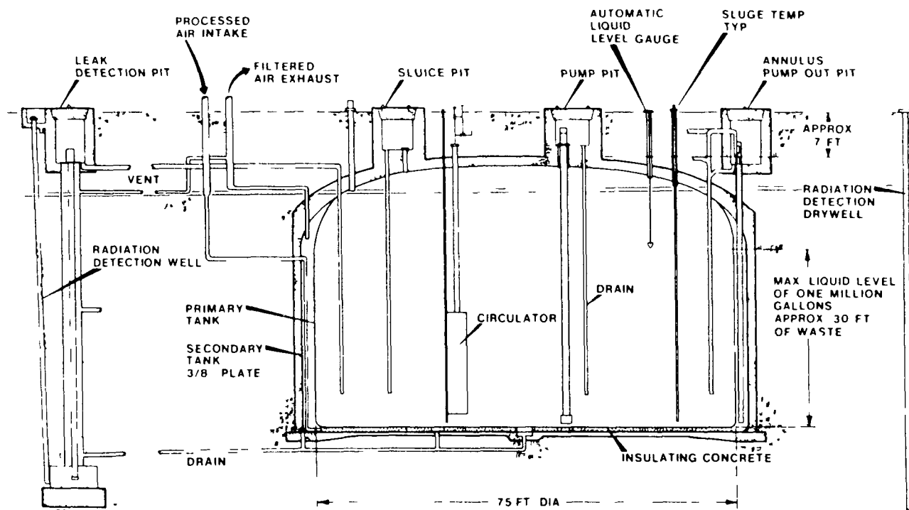
FIGURE E.3 - DOUBLE-WALL BOILING WASTE TANK
