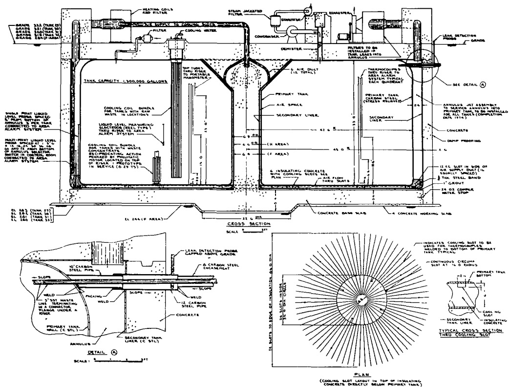
FIGURE E.5 - TYPE III STORAGE TANKS (1974-78)
