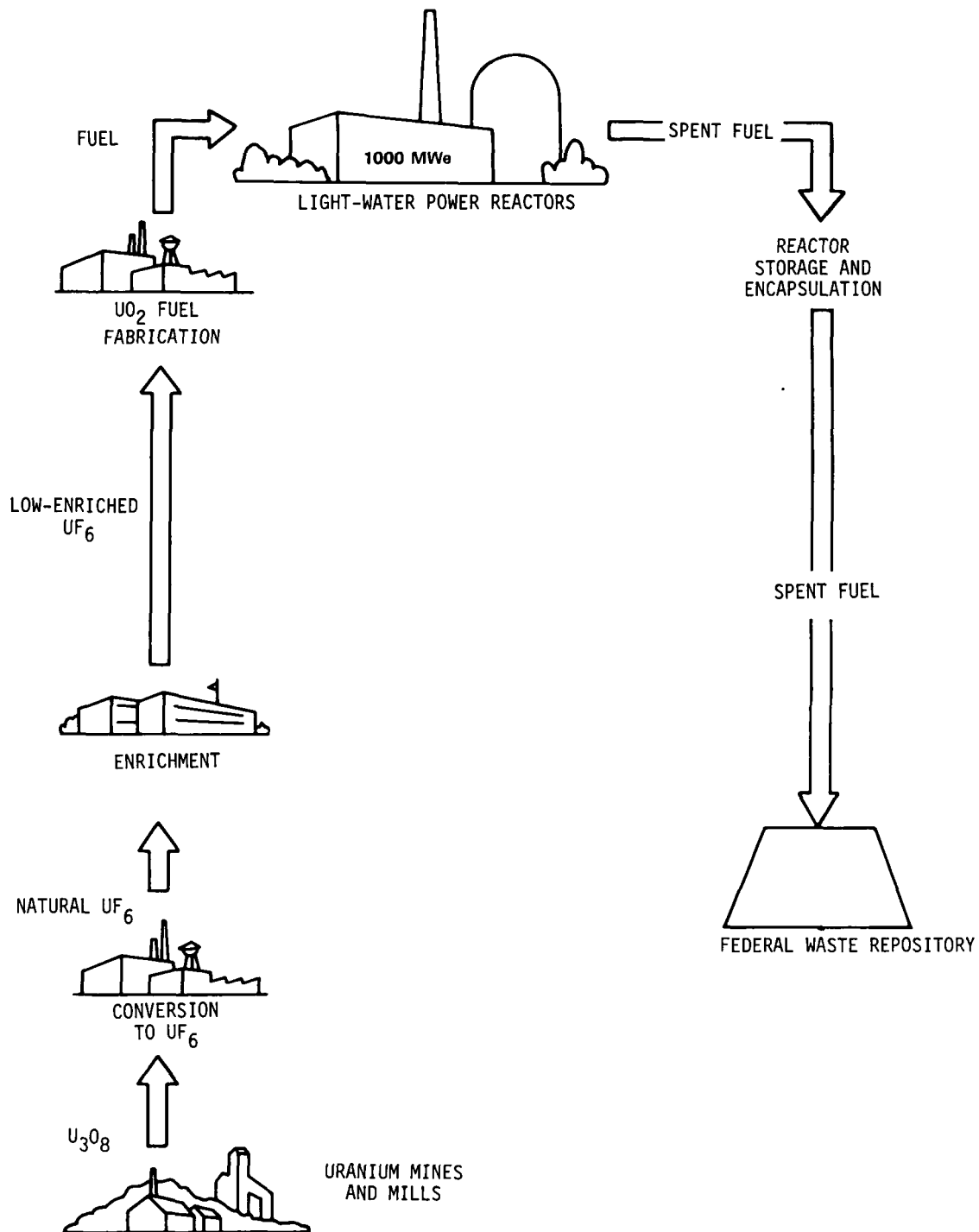
FIGURE 3.1 - NO RECYCLE
