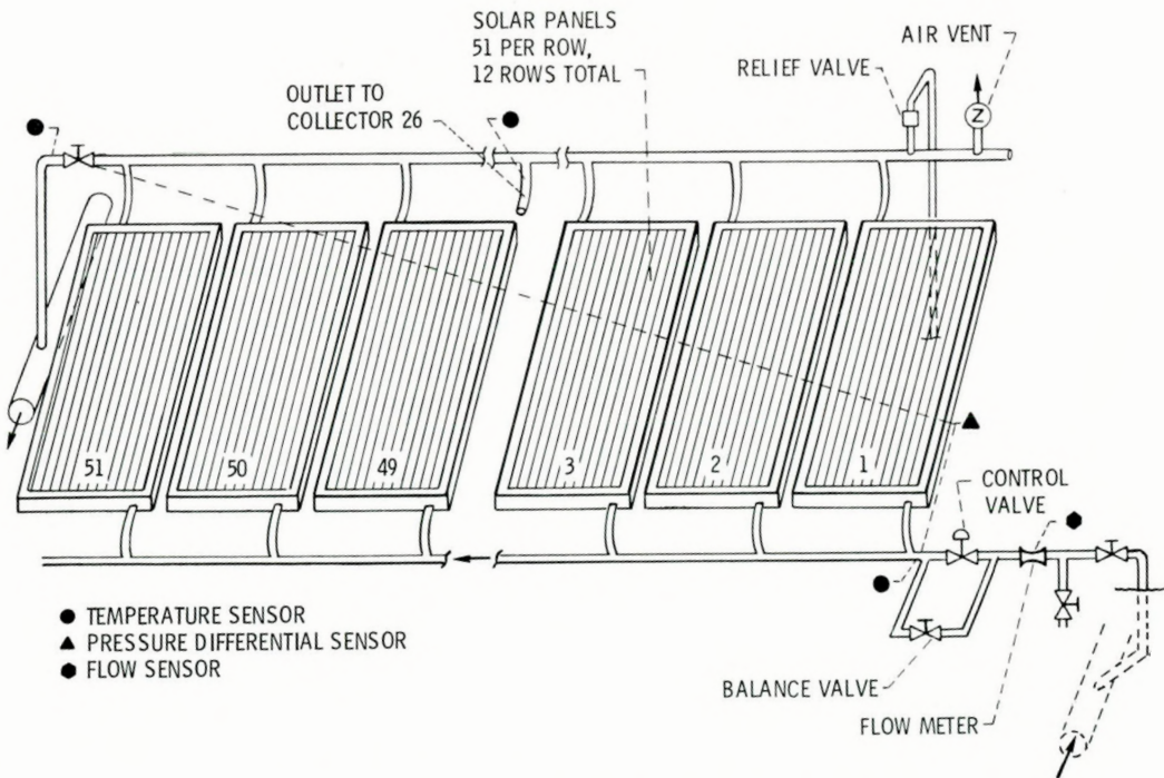
Figure 5. - Instrumentation for collector row 4 (typical for all rows).
