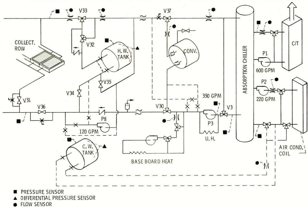
Figure 6. - Location of solar system pressure sensors and flow meters.
