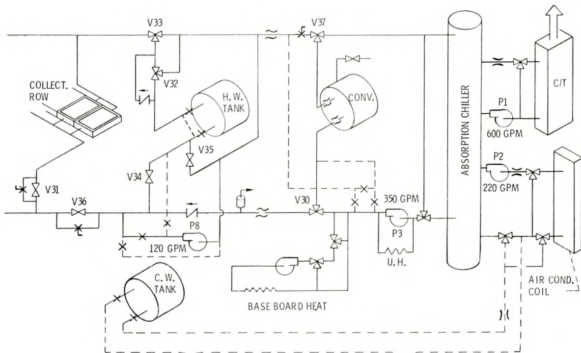
Figure 2. - Flow schematic for SBTF.
