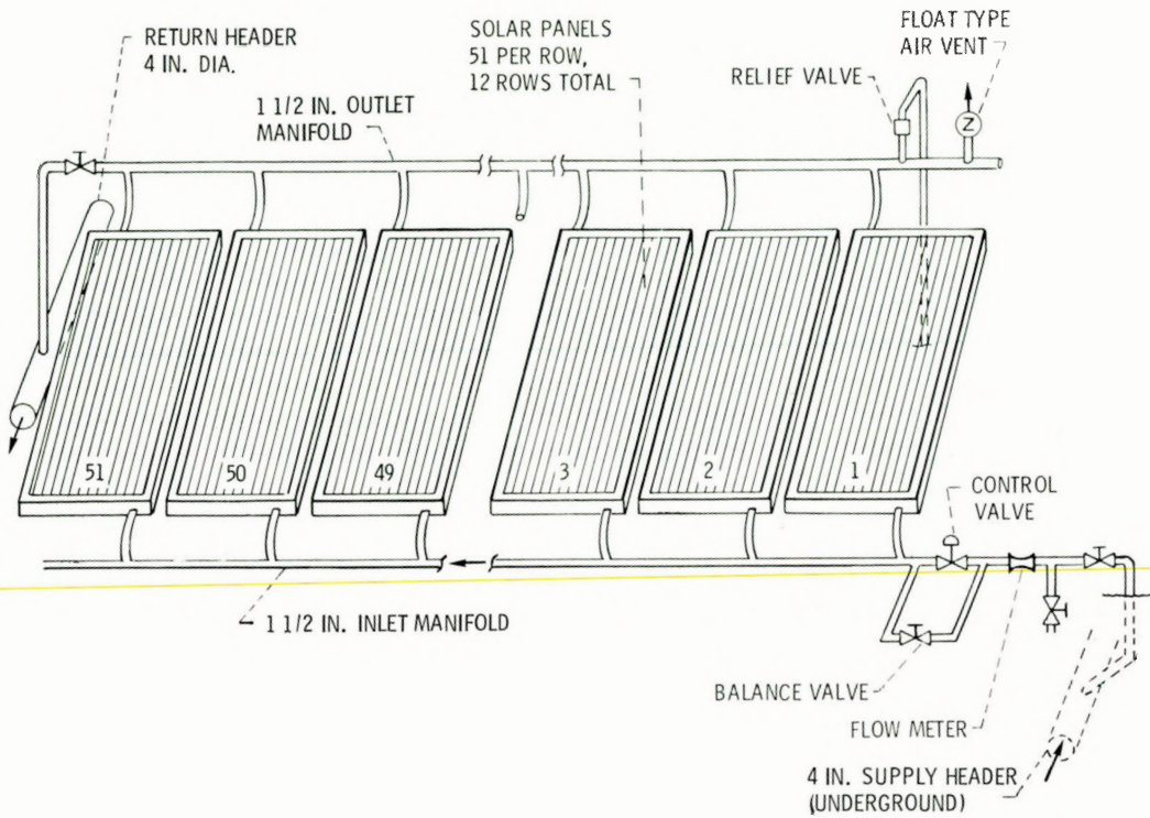
Figure 4. - Flow schematic for a typical collector row.
