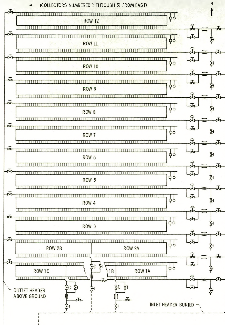
Figure 3. - General layout of solar collector field.
