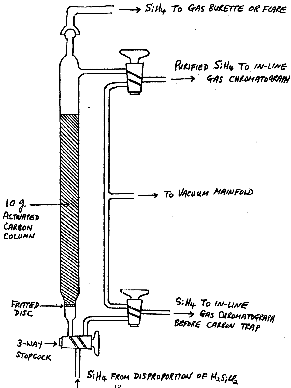
FIGURE 2 APPARATUS FOR PURIFICATION OF \text{SiH}_4
