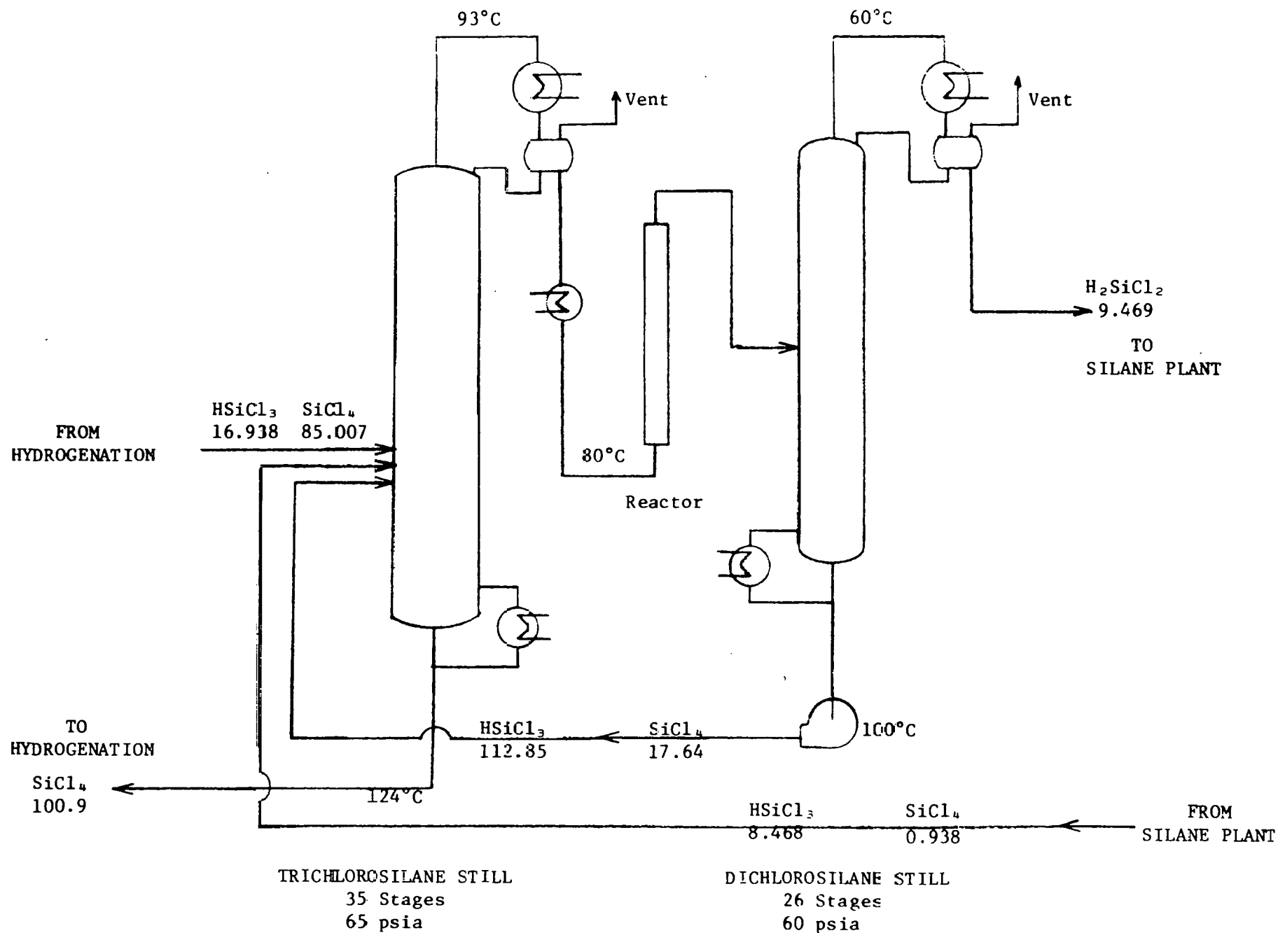
FIGURE 17 Dichlorosilane From Trichlorosilane Process Flowsheet
