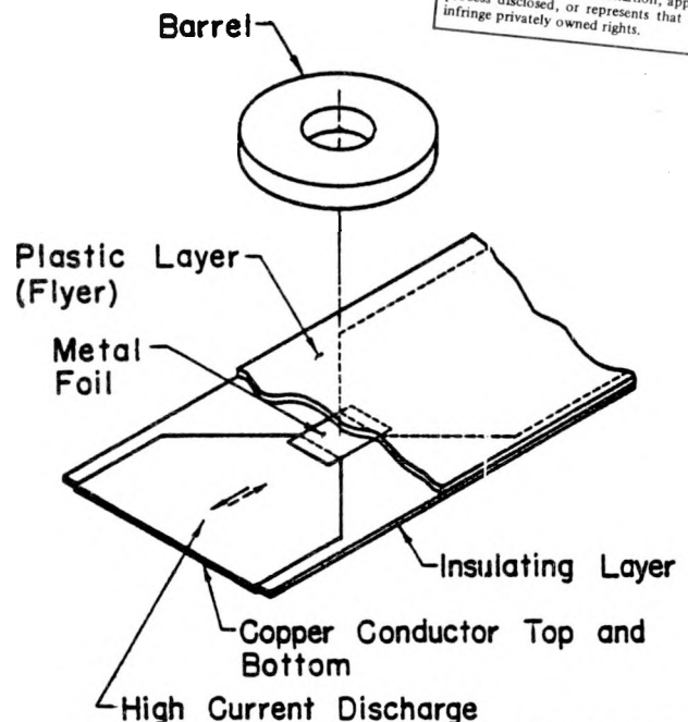
Fig. 1. Electrically driven flyer assembly.
