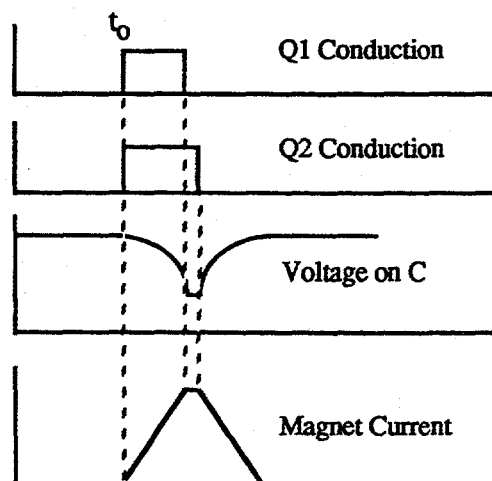
Figure 2. Waveforms for the pulse generator circuit.
