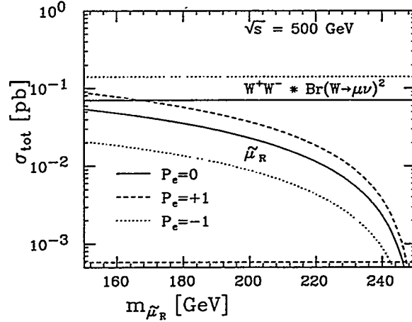
Figure 19: Total cross sections of \tilde{\mu}_R pair production at \sqrt{s} = 500 GeV, for unpolarized P_e = 0 and polarized beams P_e = \pm 1 . The background from W -pair is also shown.
