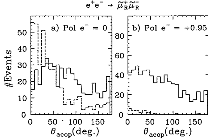
Figure 20: Acoplanarity distribution of lepton pair for \sqrt{s} = 350 GeV, m_{\tilde{l}} = 142 GeV, \int \mathcal{L} dt = 20 \text{ fb}^{-1} . Fig. b) shows the dramatic reduction of the backgrounds using the right-handed electron beam.
