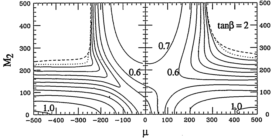
Figure 23: Contour of the total cross sections in pb of \tilde{\chi}_1^\pm pair production from the left-handed electron beam at \sqrt{s} = 500 \text{ GeV} , for m_{\tilde{\nu}_e} = 250 \text{ GeV} . The kinematic limit is shown in dashed line, while the discovery reach at 20 \text{ fb}^{-1} is shown in dotted line.
