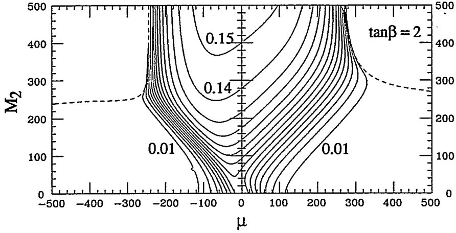
Figure 24: Contour of the total cross sections in pb of \tilde{\chi}_1^\pm pair production from the right-handed electron beam at \sqrt{s} = 500 \text{ GeV} . The kinematic limit is shown in dashed line.
