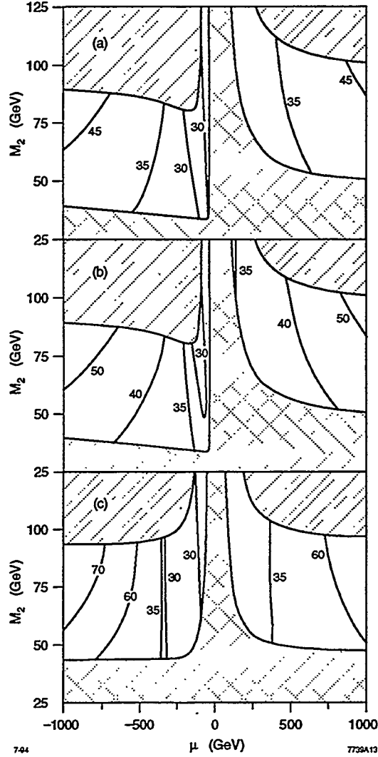
Figure 5: Contours of constant value of the leptonic branching fraction B_l (in %) in the (\mu, M_2) plane for M_1/M_2 = 0.5 and three sets of parameters (\tan \beta, m_t, m_{\bar{q}}) : (a) (2, 200, 200), (b) (2, 200, 800), and (c) (10, 200, 200). Note that we used different scales for \mu and M_2 to make the numbers visible and to expand the gaugino region. For all figures, the value of B_l is \frac{1}{3} in the Higgsino region and grows as one approaches the gaugino region. The growth is faster for large \tan \beta (c) than for low \tan \beta (a). In (a) and (b) the B_l contours differ by approximately 5% in the far gaugino region. Note also the “pocket” in the \mu < 0 near gaugino region, where B_l < \frac{1}{3} . The exchange of the charged Higgs is neglected in the decay process. Taken from Ref. [70].
