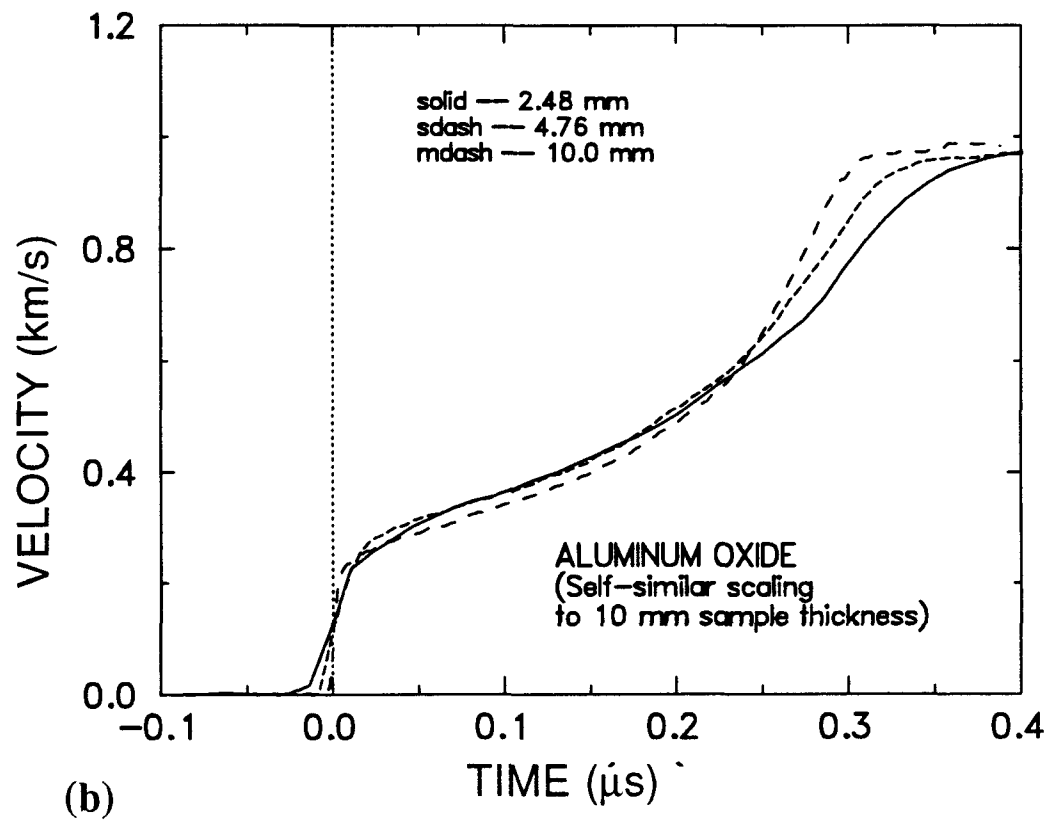
Figure 10.1 Velocity profiles for aluminum oxide. (a) Measured wave profiles. (b) Self-similar representation of wave profiles.
