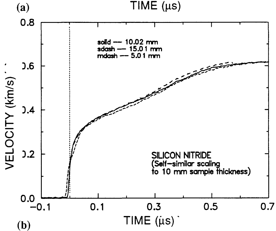
Figure 10.3 Velocity profiles for silicon nitride. (a) Measured wave profiles. (b) Self-similar representation of wave profiles.
