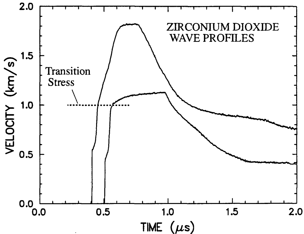
Figure 9.5 Experimental VISAR profiles for \text{ZrO}_2 indicating yield and transition characteristics.
