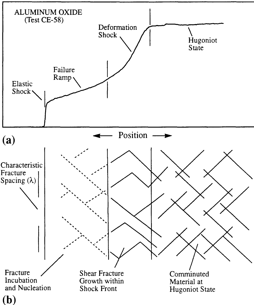
Figure 2.4 Shock wave compression profile for aluminum oxide (a) and schematic of brittle shear fracture process within the shock-wave front (b).
