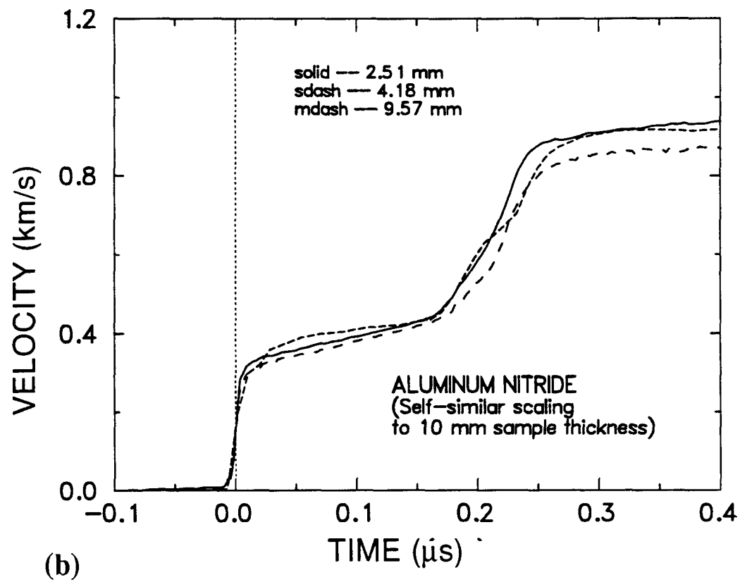
Figure 10.2 Velocity profiles for aluminum nitride. (a) Measured wave profiles. (b) Self-similar representation of wave profiles.
