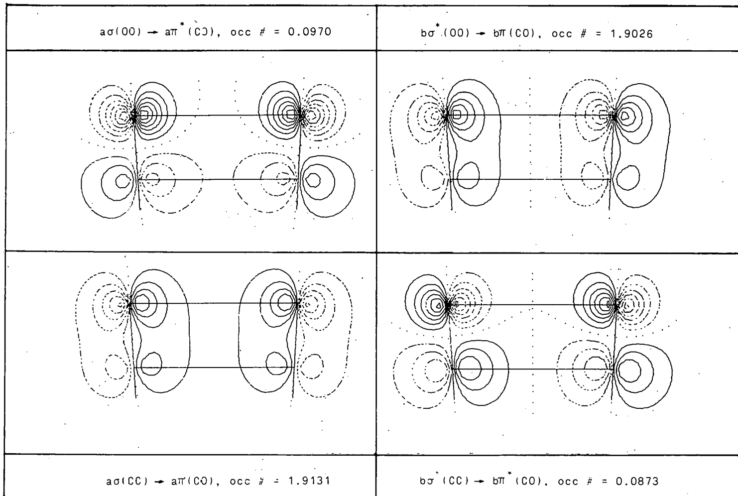
Figure 21. NRO's for 1,2-dioxetane at R_{CC} = 5.8754 a.u.
