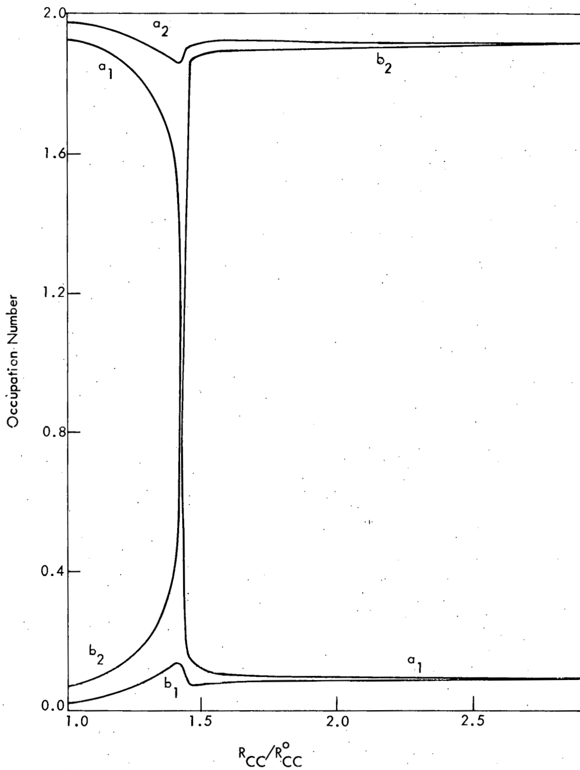
Figure 23. Occupation numbers for the MCSCF function \Psi
