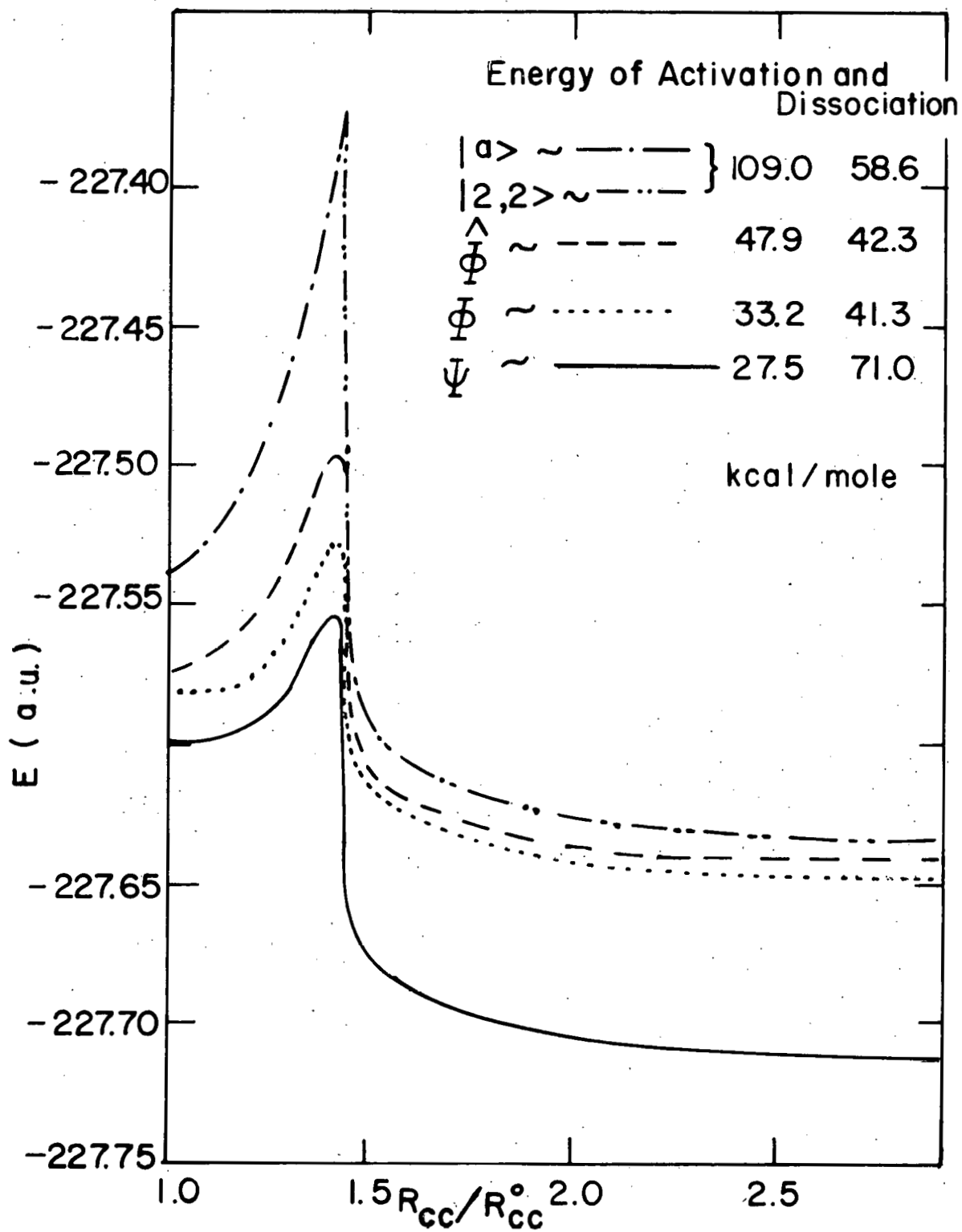
Figure 24. Total molecular energies for several wavefunctions
