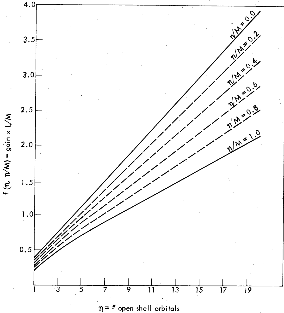
Figure 2. Relation of the gain of the SPIP method as a function of the number of open shell orbitals for several values of the ratio of the number of open to closed shell orbitals.
