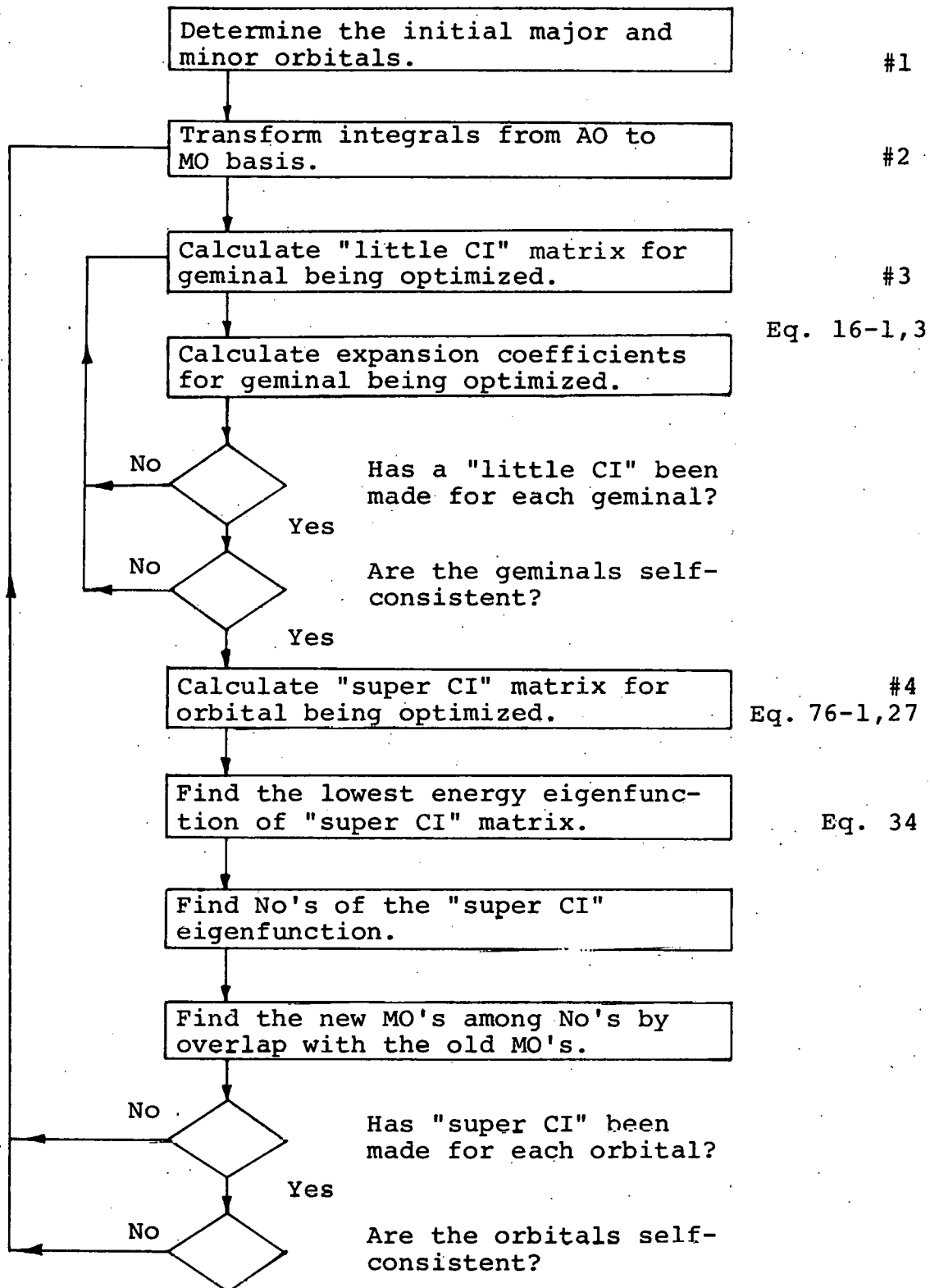
Figure 1. Flow diagram of the SPIP algorithm.
