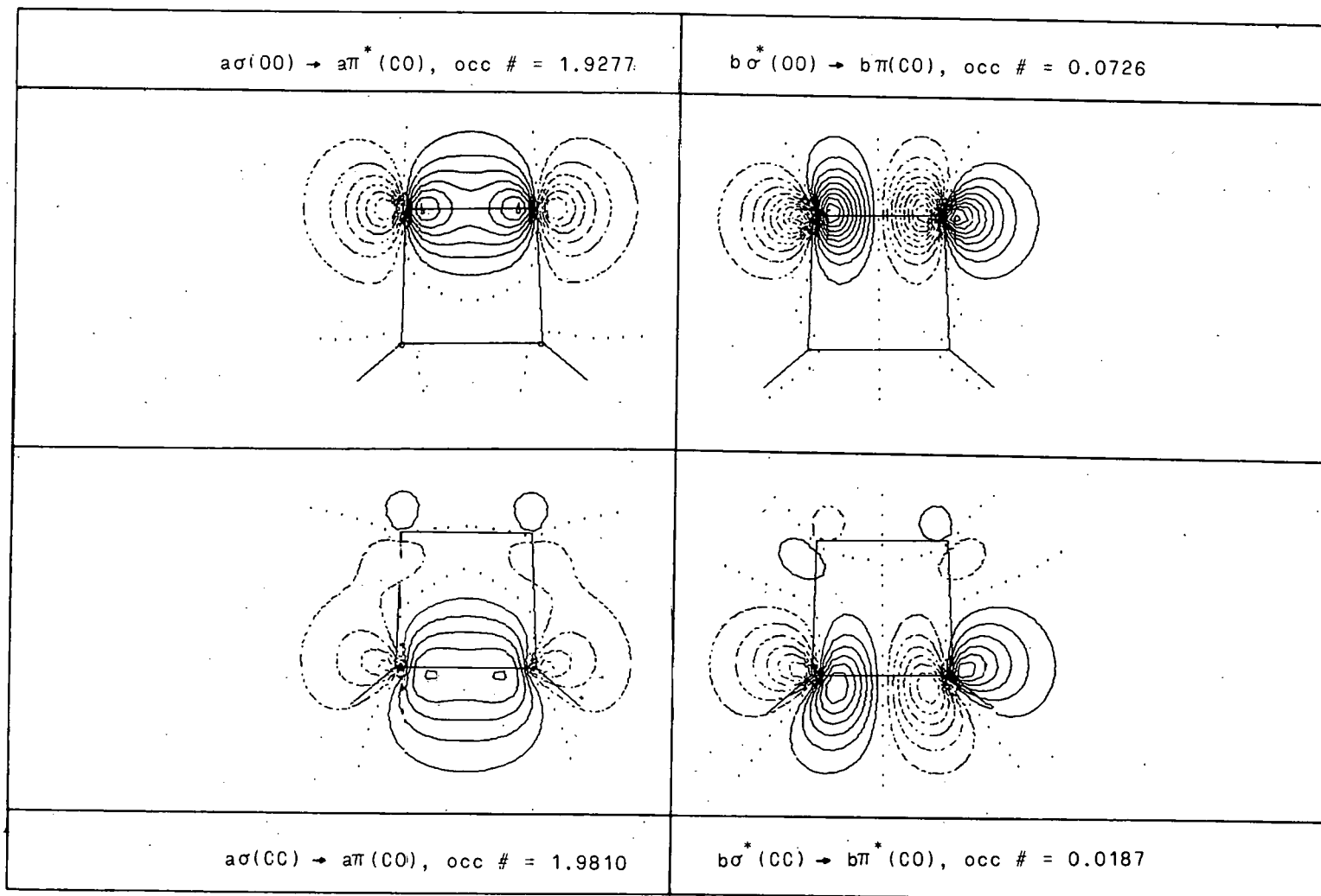
Figure 13. NRO's for 1,2-dioxetane at R_{CC} = 2.8754 a. u. (molecular equilibrium).
