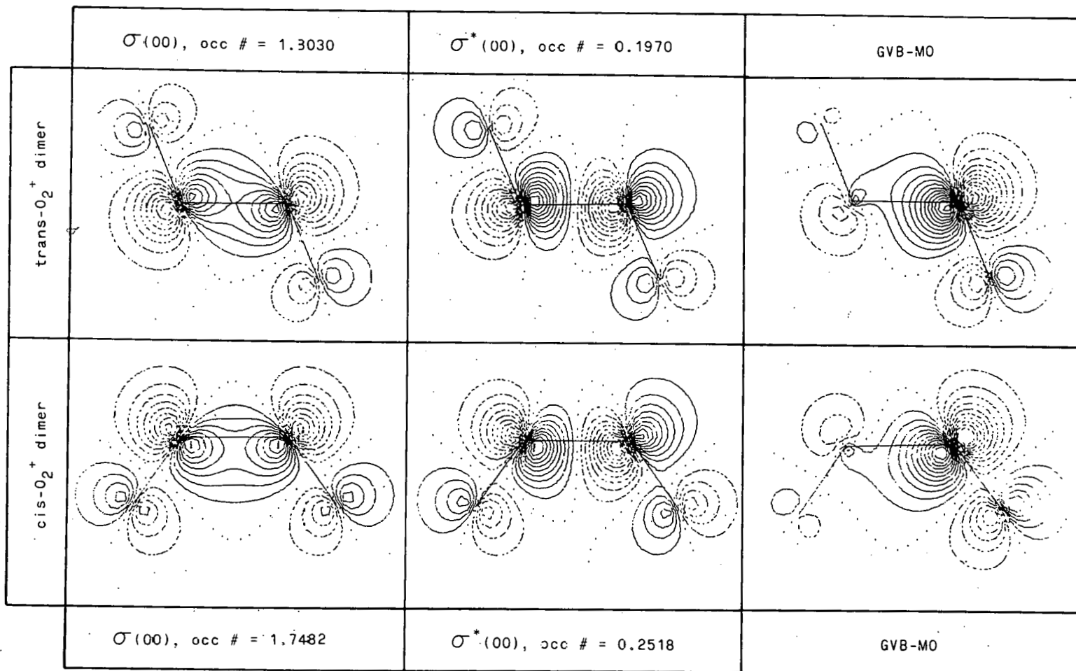
Figure 7. Major and minor natural orbitals and GVB orbitals for O_2^+ dimer.
