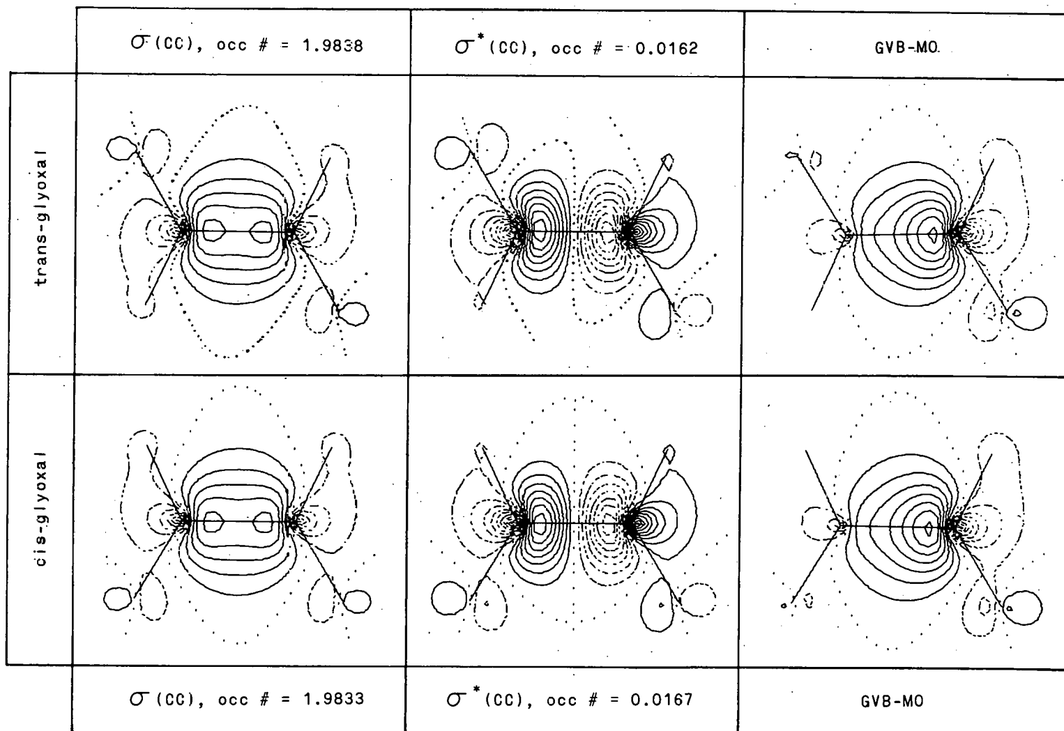
Figure 5. Major and minor natural orbitals and GVB orbitals for glyoxal.
