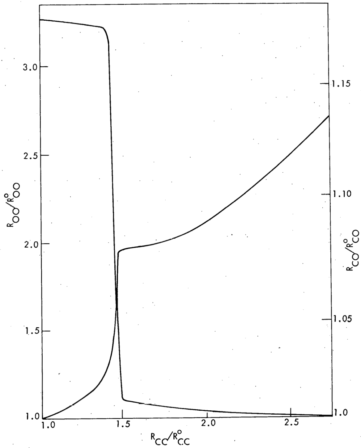
Figure 8. Major bond lengths along reaction path
