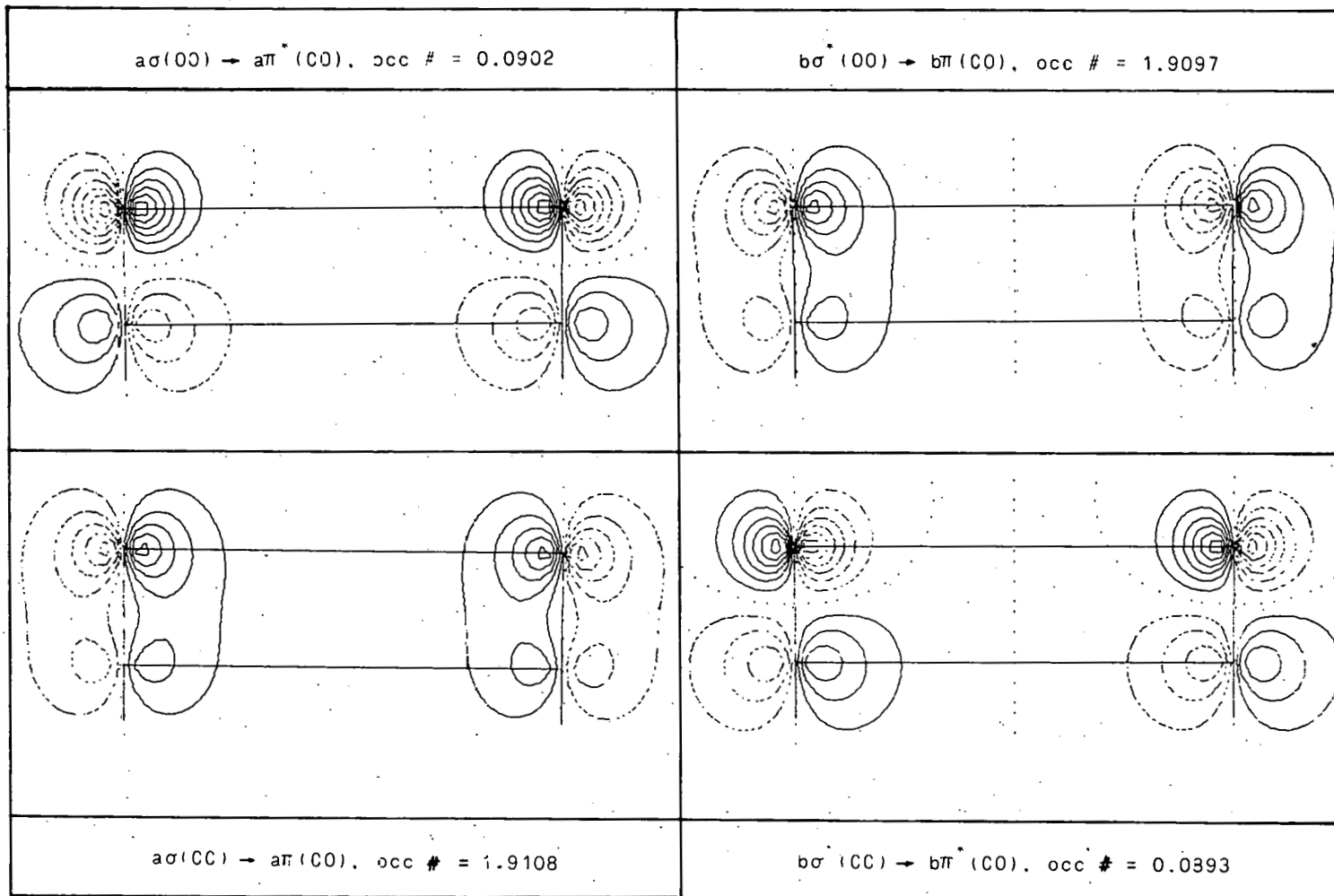
Figure 22. NRO's for 1,2-dioxetane at R_{CC} = 8.8754 a.u.
