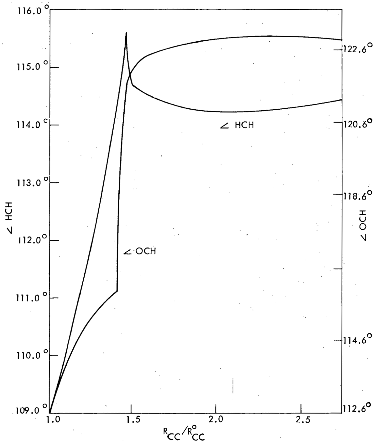
Figure 9. Bond angles along the reaction path
