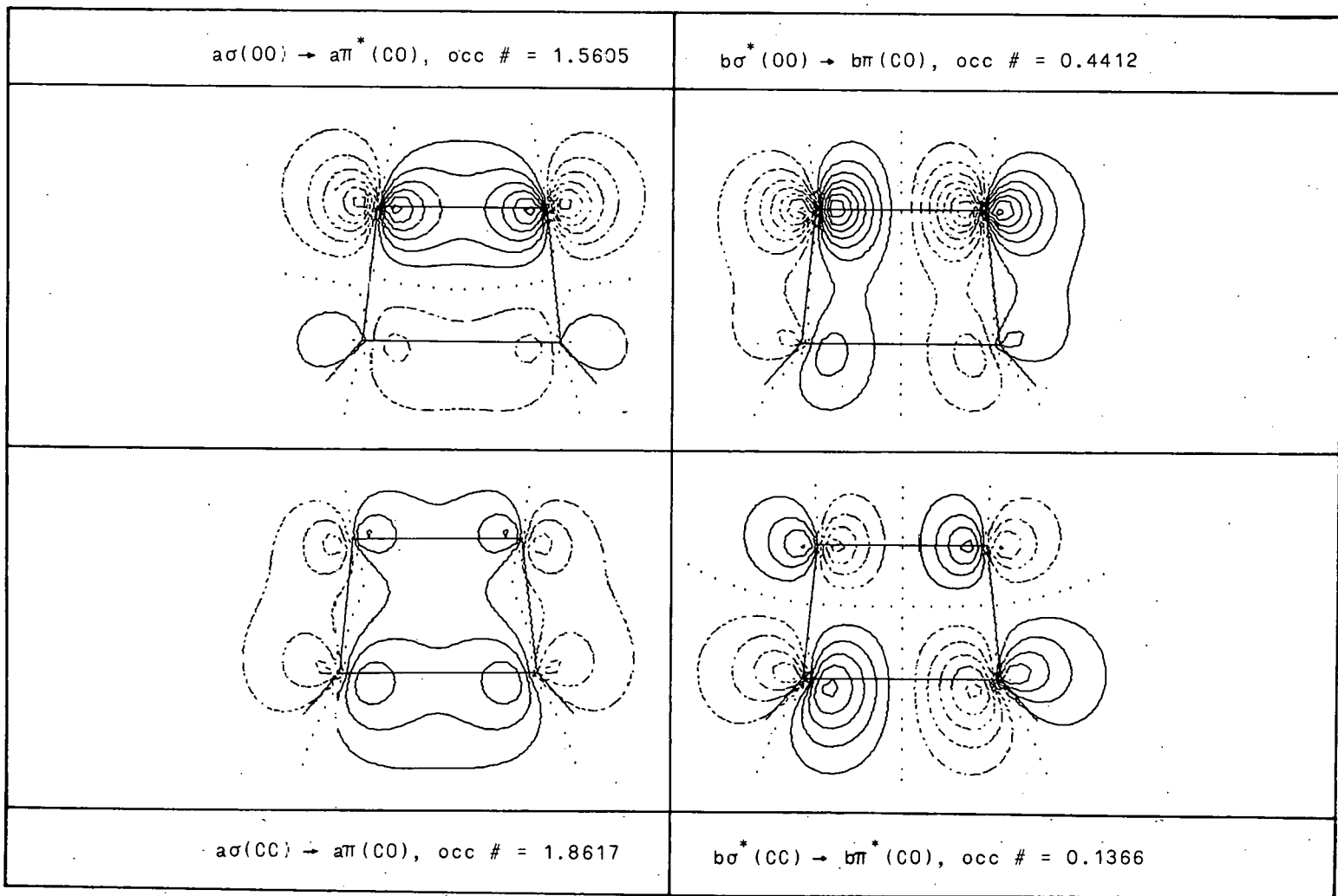
Figure 17. NRO's for 1,2-dioxetane at R_{CC} = 4.0369 a.u. (barrier maximum)
