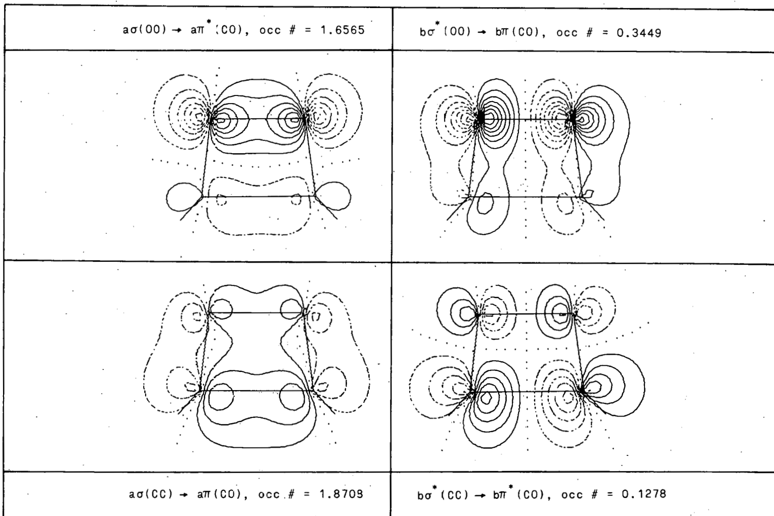
Figure 16. NRO's for 1,2-dioxetane at R_{CC} = 3.9872 a.u.
