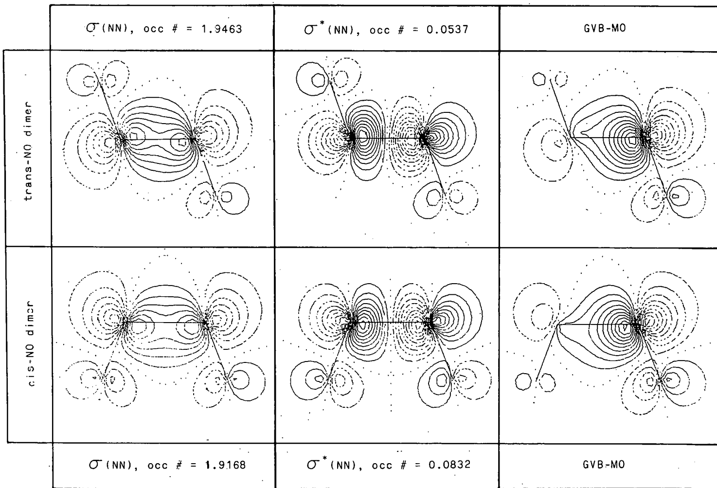
Figure 6. Major and minor natural orbitals and GVB orbitals for NO dimer.
