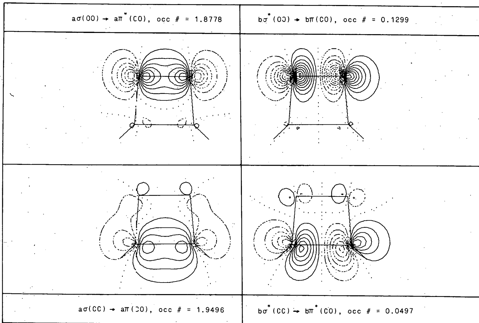
Figure 14. NRO's for 1,2-dioxetane at R_{CC} = 3.3754 a.u.
