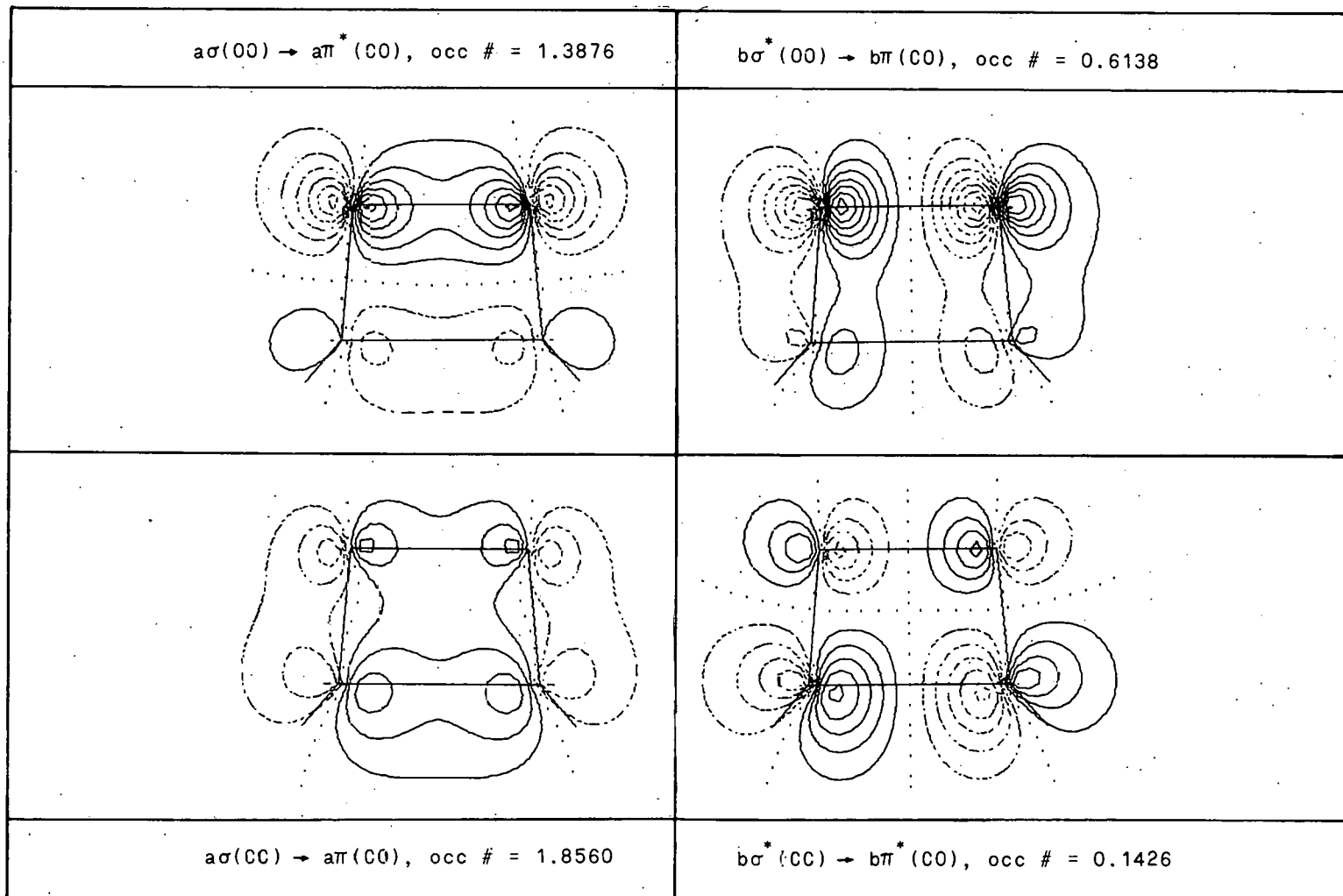
Figure 18. NRO's for 1,2-dioxetane at R_{CC} = 4.0754 a.u.
