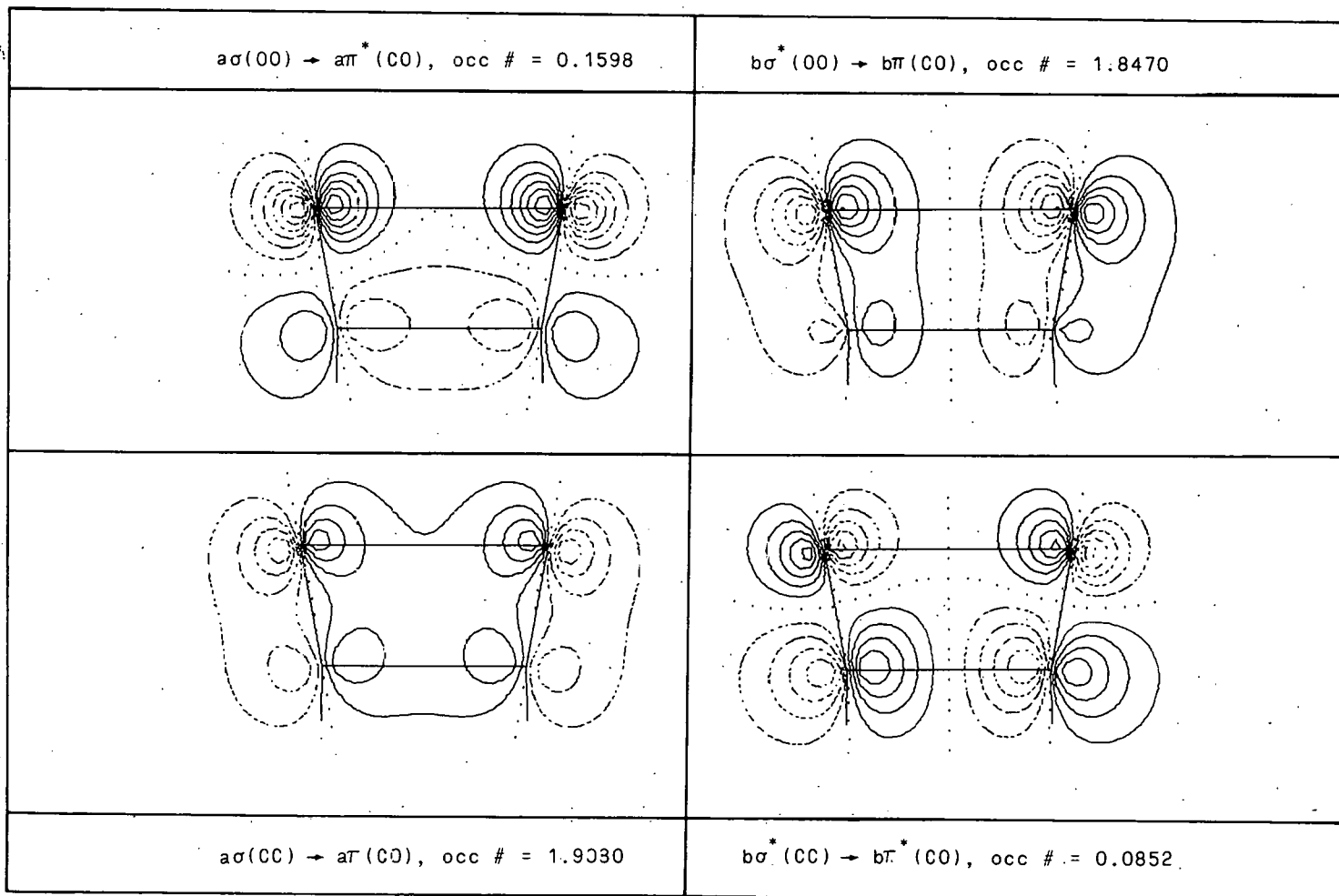
Figure 19. NRO's for 1,2-dioxetane at R_{CC} = 4.1754 a.u.
