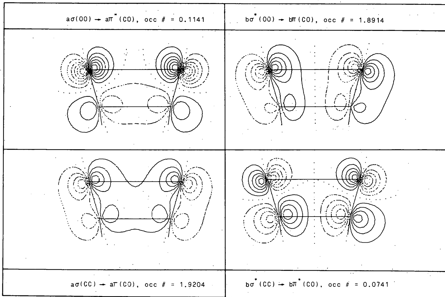
Figure 20. NRO's for 1,2-dioxetane at R_{CC} = 4.3754 a.u.
