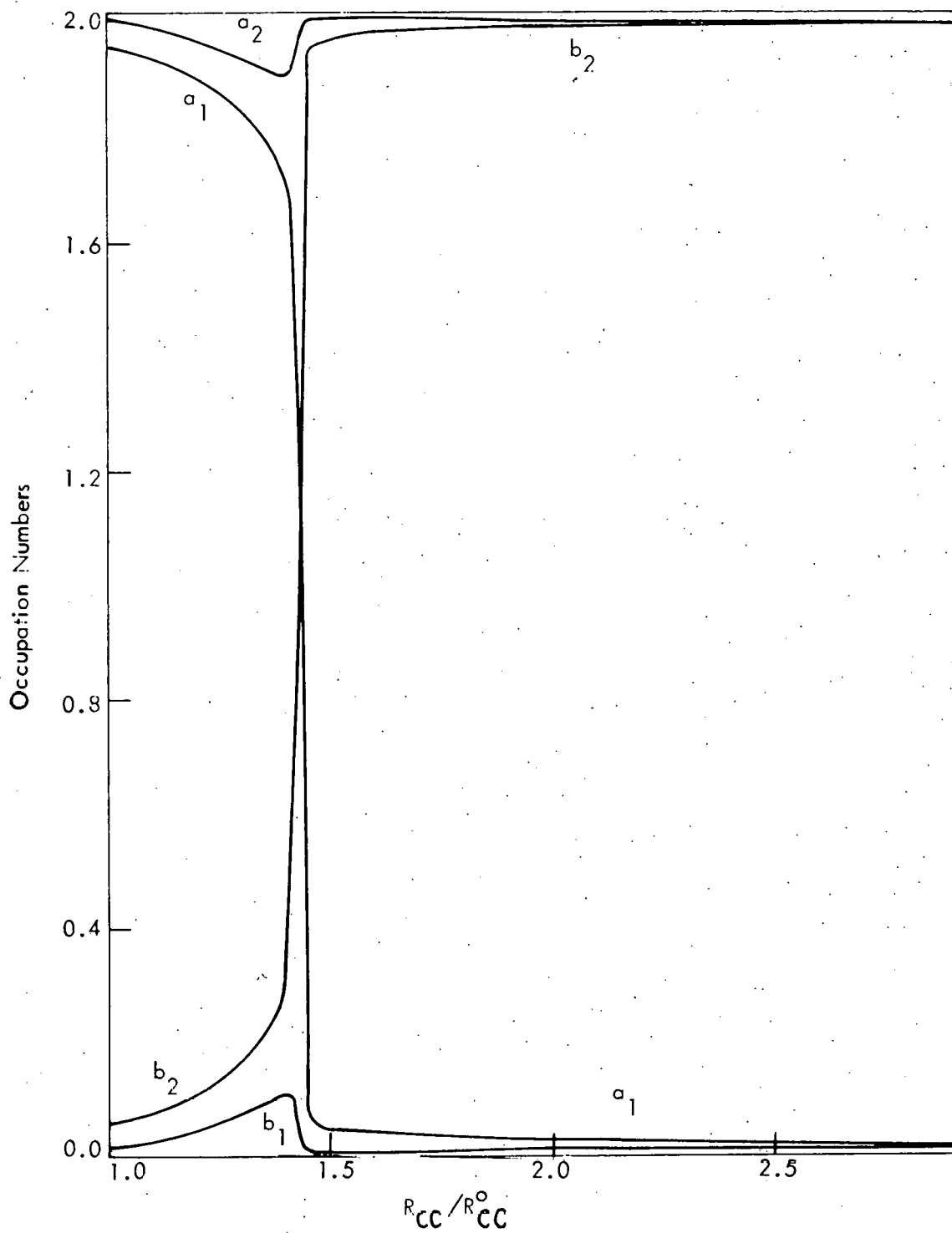
Figure 12. Occupation numbers from the two-geminal SPIP function \Phi
