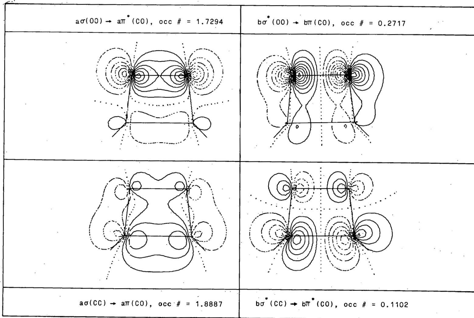
Figure 15. NRO's for 1,2-dioxetane at R_{CC} = 3.8754 a.u.
