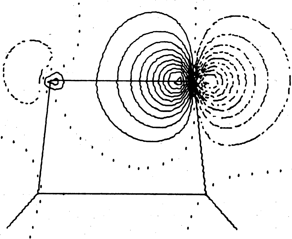
Figure 25. GVB orbital for the one-geminal SPIP function \hat{\phi} at the barrier maximum
