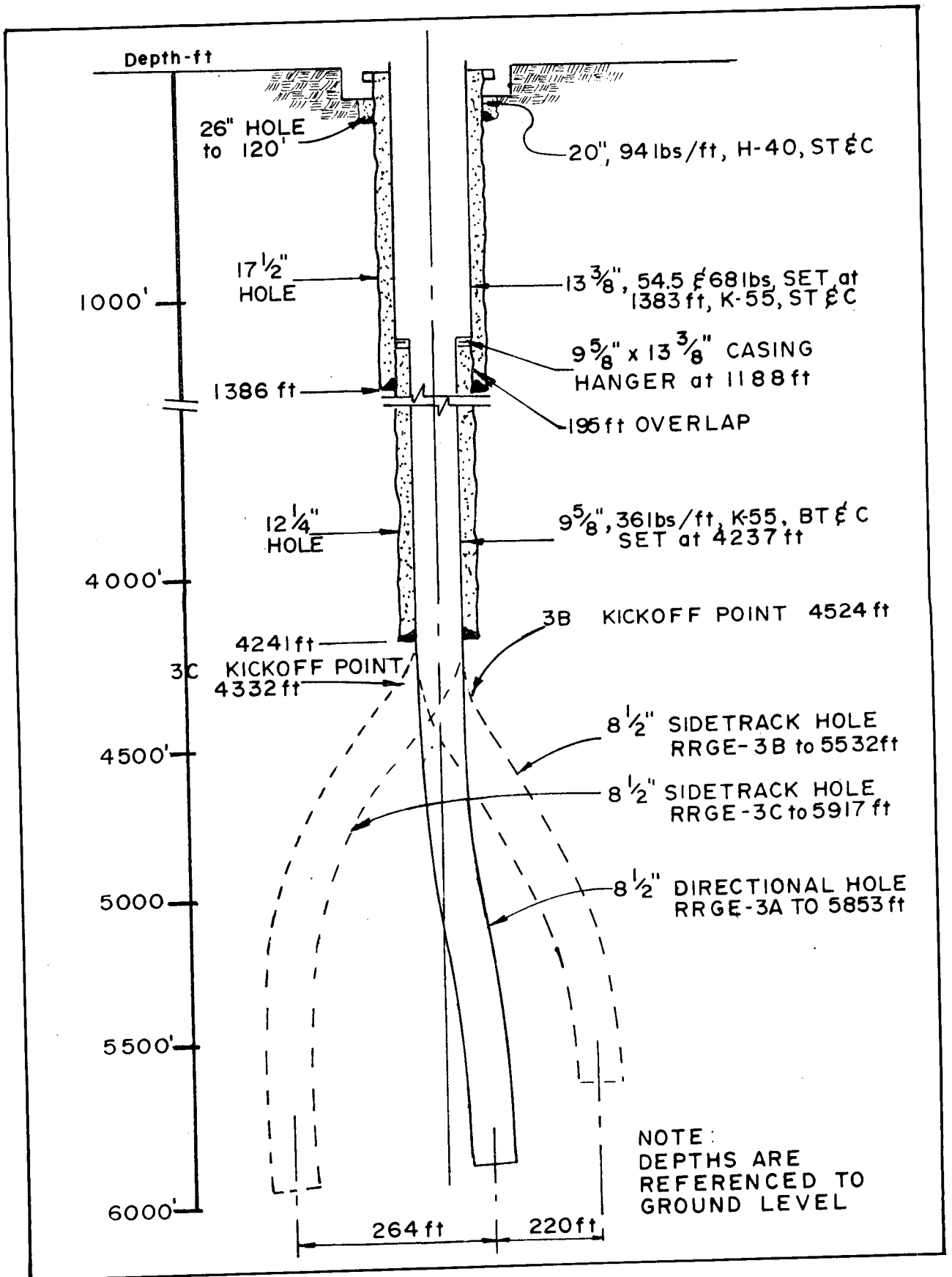
Figure 4. Subsurface Well Status
