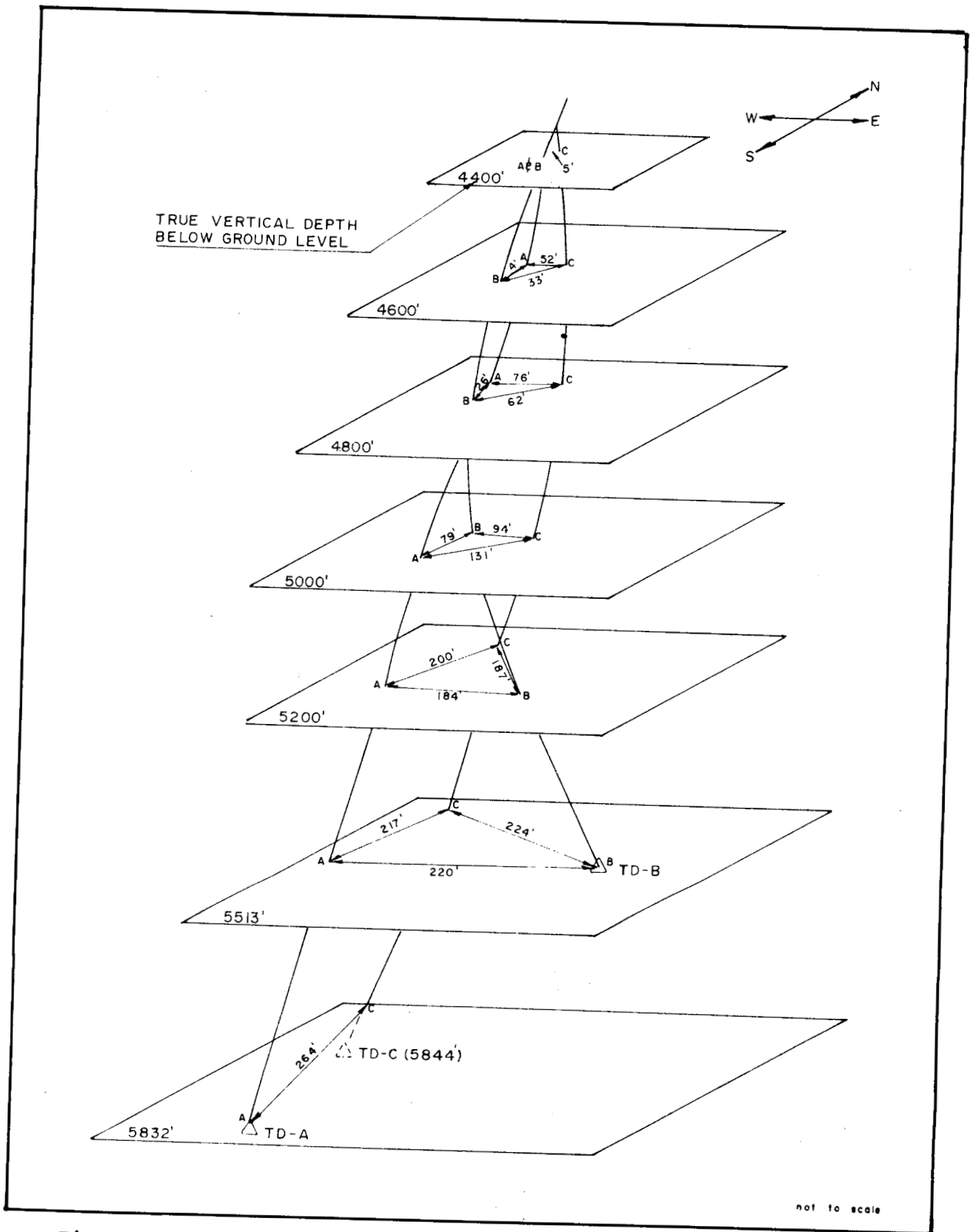
Figure 5. RRGE-3 Hole Relationship, Depth vs Horizontal Separation
