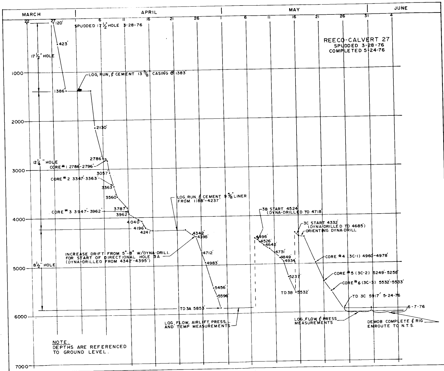
Figure 6. Drilling and Operations Summary
