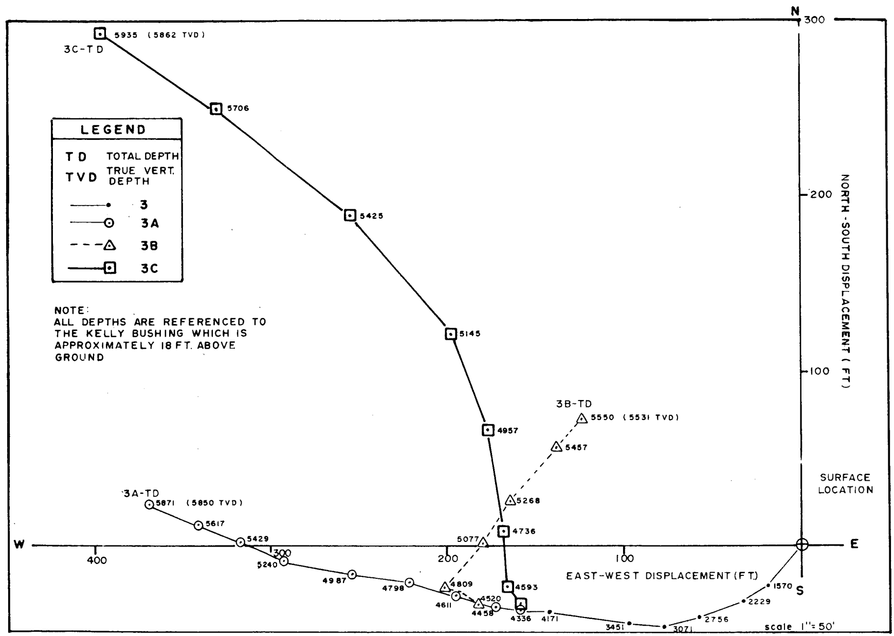
Figure 7. RRGE-3 Directional Survey Summary
