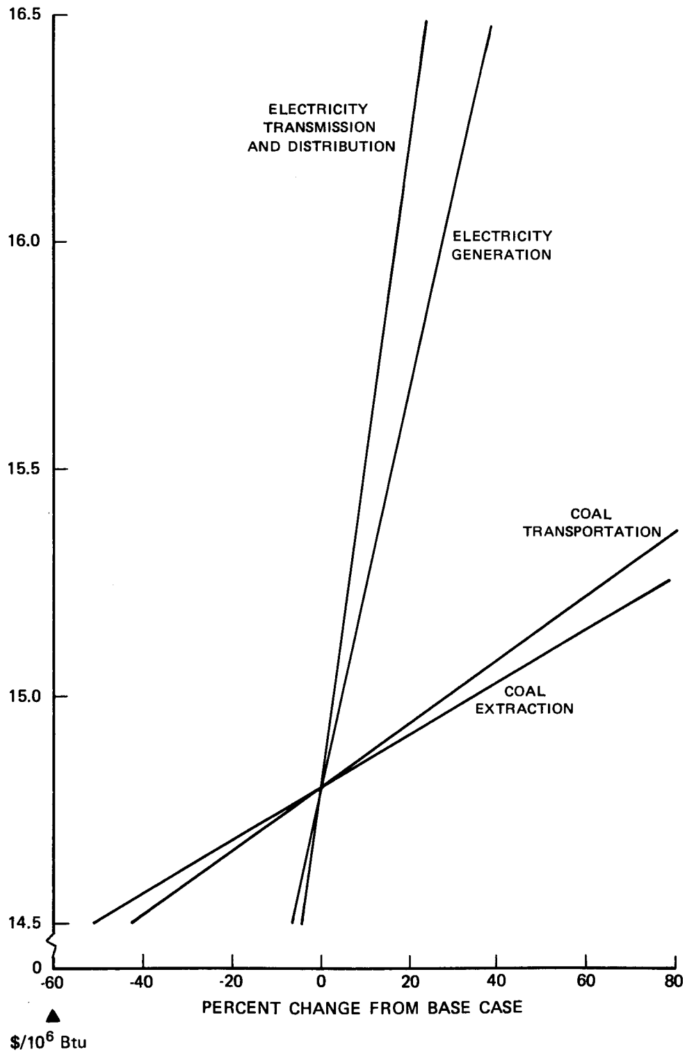
FIGURE C-6. COST SENSITIVITY: COAL FIRED POWER PLANT IN BOSTON, MASSACHUSETTS USING APPALACHIAN SURFACE COAL
