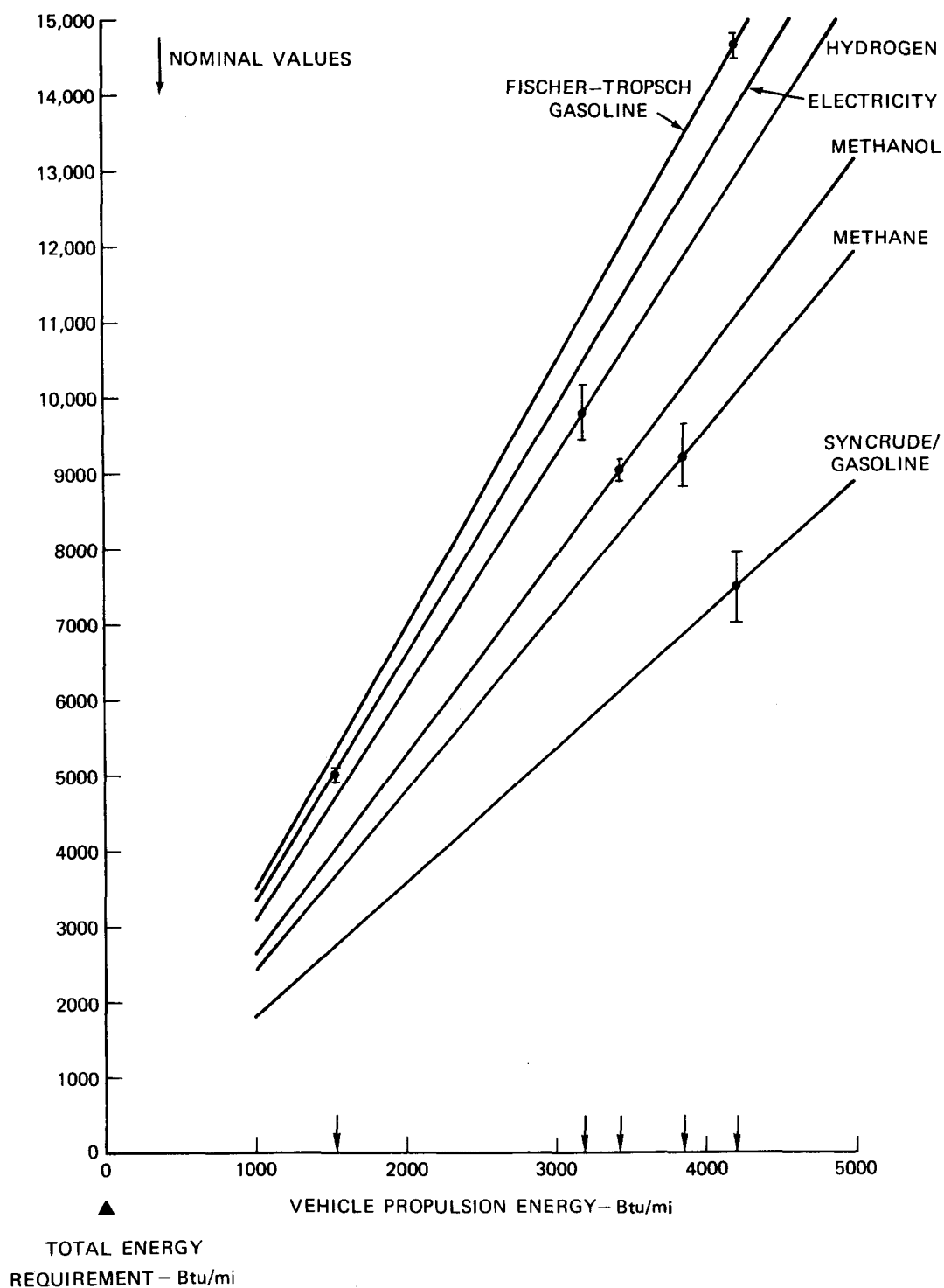
FIGURE 4-3. TOTAL ENERGY REQUIREMENTS FOR AUTOMOTIVE TRANSPORTATION
