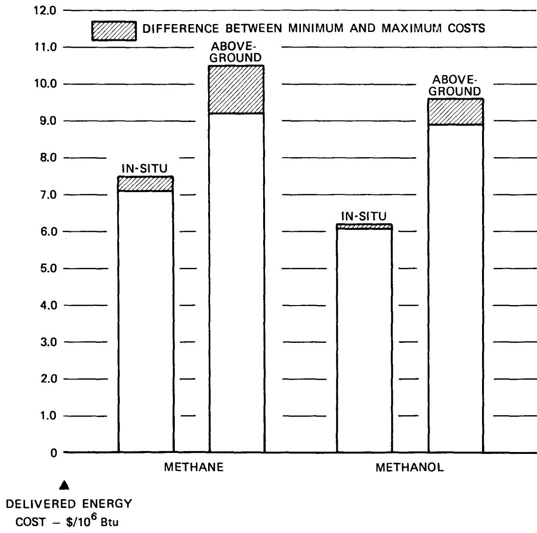
FIGURE 3-5. COMPARISON OF DELIVERED METHANE AND METHANOL COSTS USING IN-SITU AND ABOVE-GROUND COAL GASIFICATION
