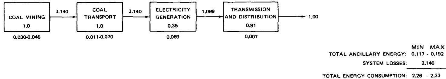
FIGURE 4-1b. ENERGY CONSUMPTION BY SYNTHETIC FUEL SYSTEMS
