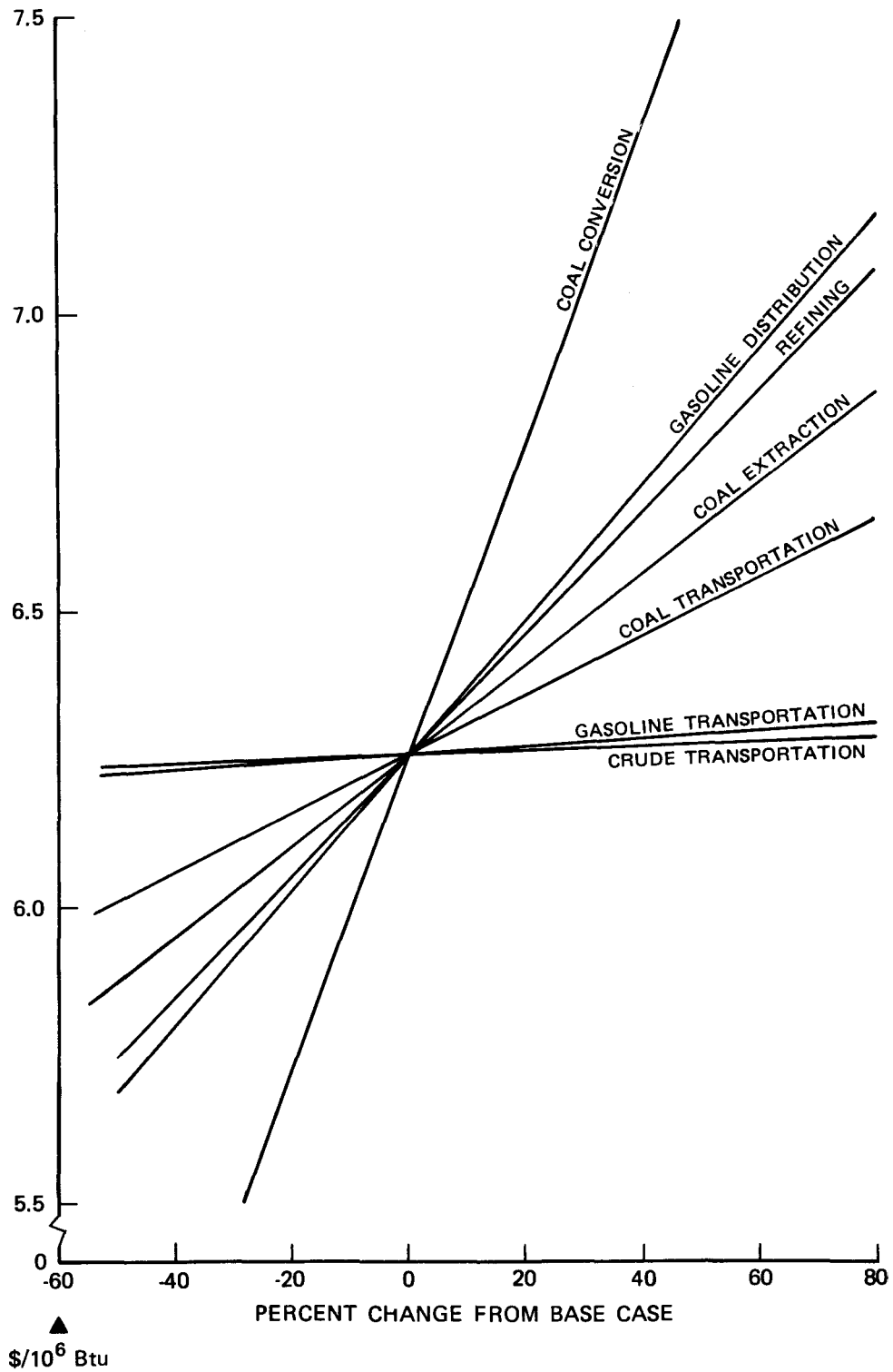
FIGURE C-1. COST SENSITIVITY: SYNCRUDE PLANT IN BEAUMONT, TEXAS USING APPALACHIAN UNDERGROUND COAL
