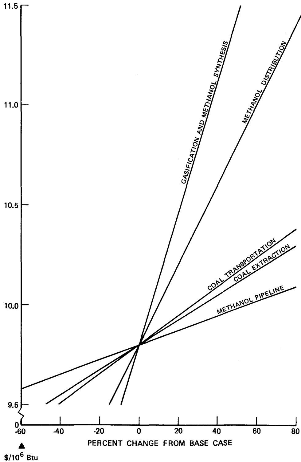
FIGURE C-3. COST SENSITIVITY: METHANOL PLANT IN GALVESTON, TEXAS USING APPALACHIAN SURFACE COAL
