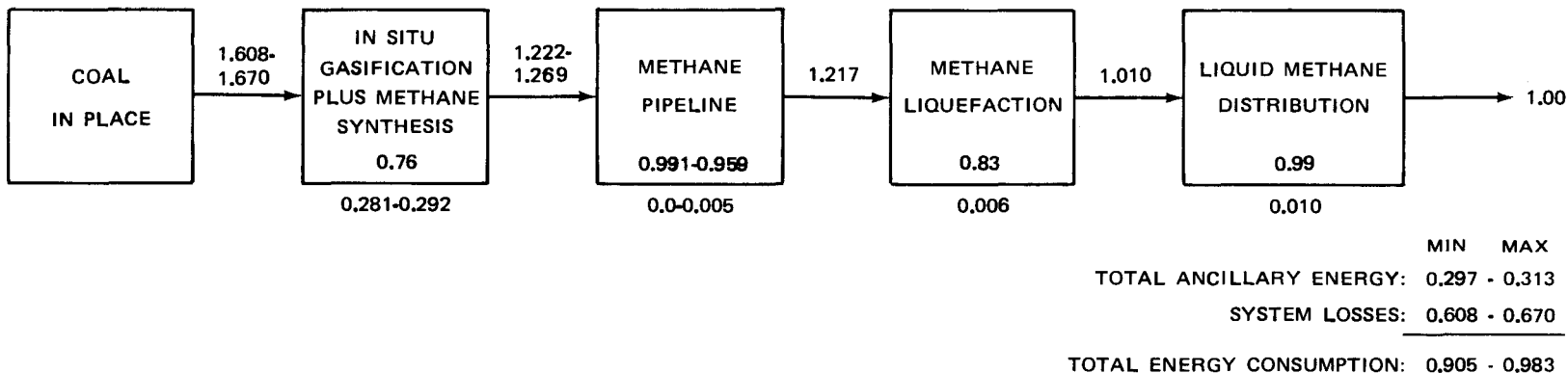
FIGURE 4-1c. ENERGY CONSUMPTION BY SYNTHETIC FUEL SYSTEMS NUMBERS ABOVE THE ARROWS ARE ENERGY FLOWS; NUMBERS BELOW THE BOXES ARE ANCILLARY ENERGY REQUIREMENTS; ALL THESE NUMBERS ARE IN UNITS OF 10^6 Btu. NUMBERS WITHIN THE BOXES ARE EFFICIENCIES OF SYSTEM ELEMENTS.
