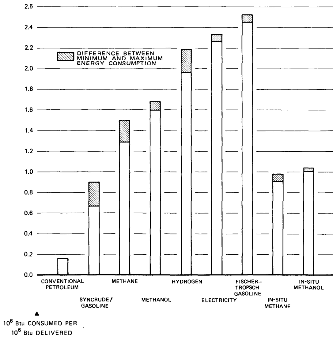
FIGURE 4-2. ENERGY CONSUMPTION BY AUTOMOTIVE ENERGY SUPPLY SYSTEMS
