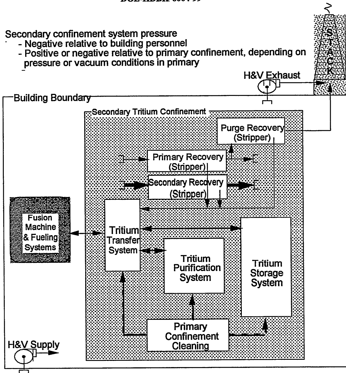
Figure II-2. Tritium processing schematic.
