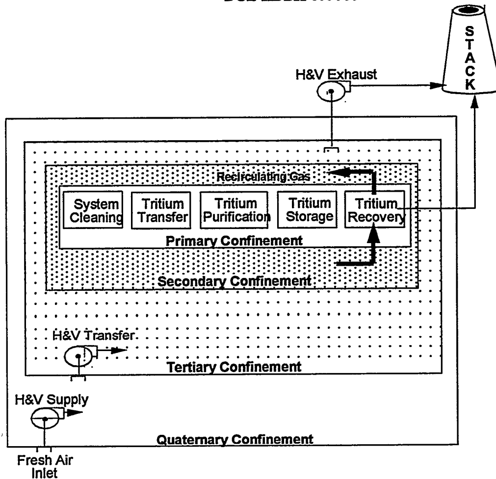
Figure II-1. Tritium confinement scheme.
