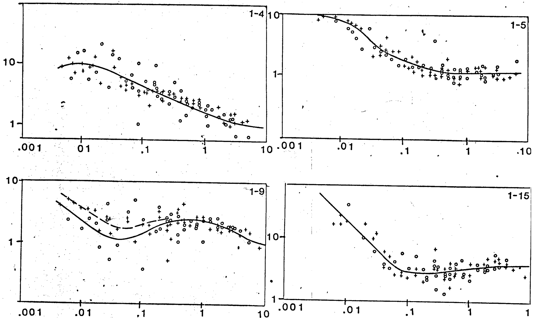
Figure 4.--Tensor resistivity amplitude curves for MT sites 1-4, 1-5, 1-9 and 1-15. Crosses are TE data, circles TM. Horizontal axes are log frequency, vertical axes are apparent resistivity in ohm-metres.
