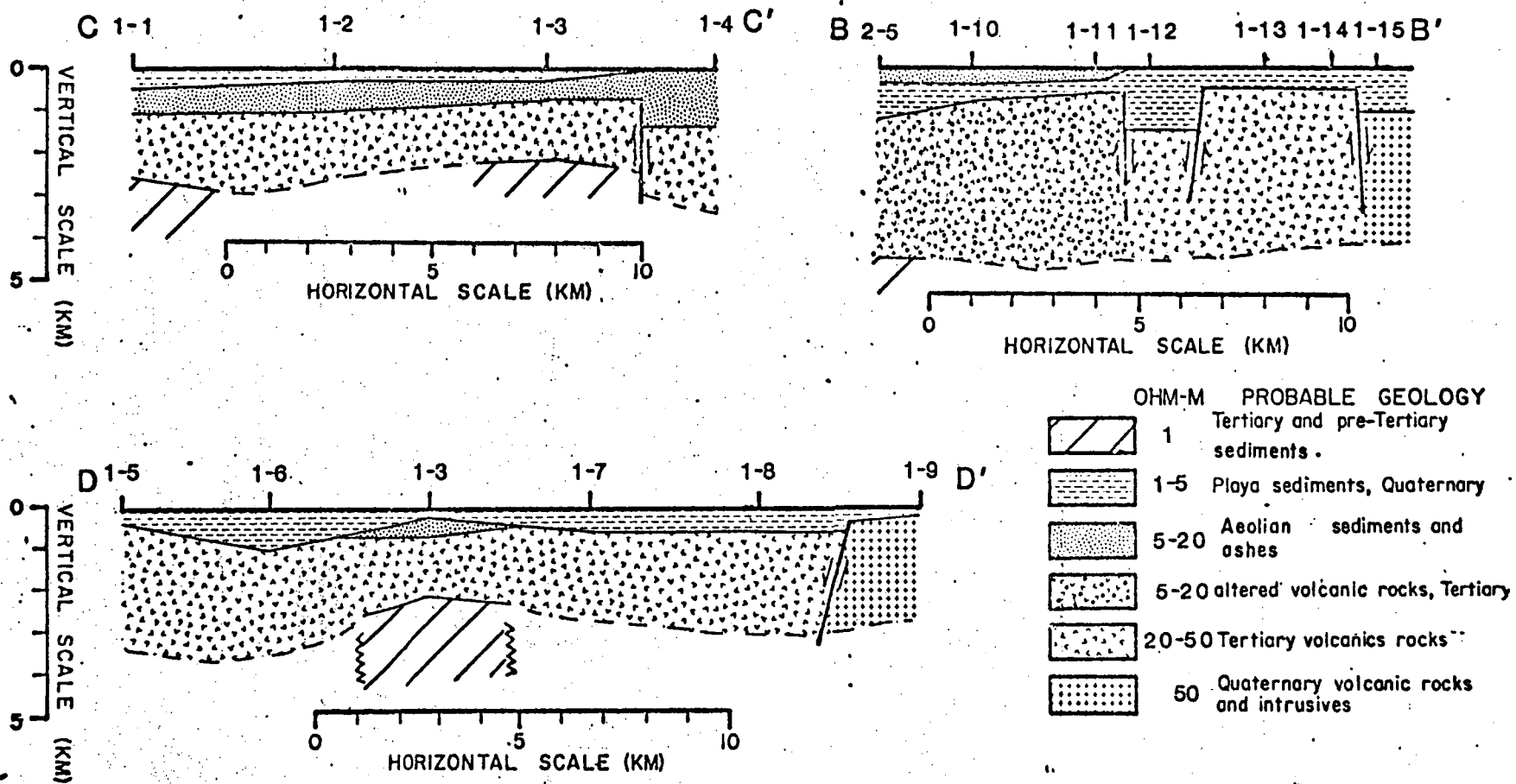
Figure 7.--MT cross-sections BB', CC', and DD'
