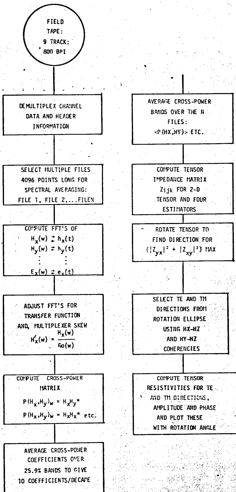
Figure 2.--Flow chart for magnetotelluric data processing.
