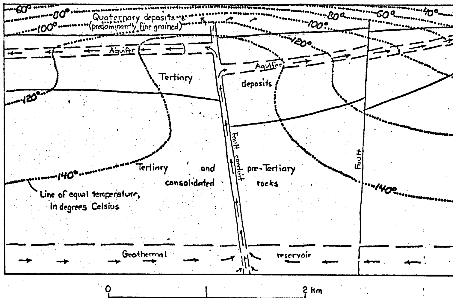
Figure 8.--Geologic cross-section through Stillwater thermal area; from
