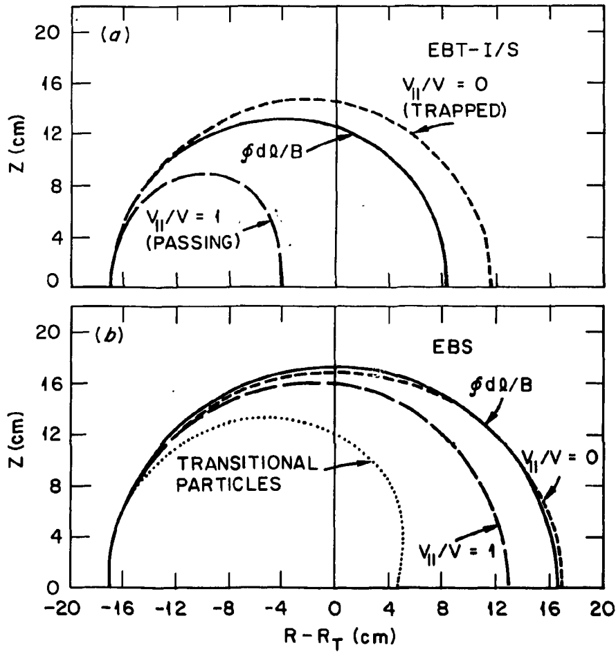
Fig. 4.7. Comparison of high-energy particle orbits for the circular (top) and square (bottom) configurations. Highly trapped particles ( v_{||} = 0 ) and extreme passing particles ( v_{||} = v; \mu = 0 ) are shown. For reference purposes, contours of \oint d\ell/B are also shown.
