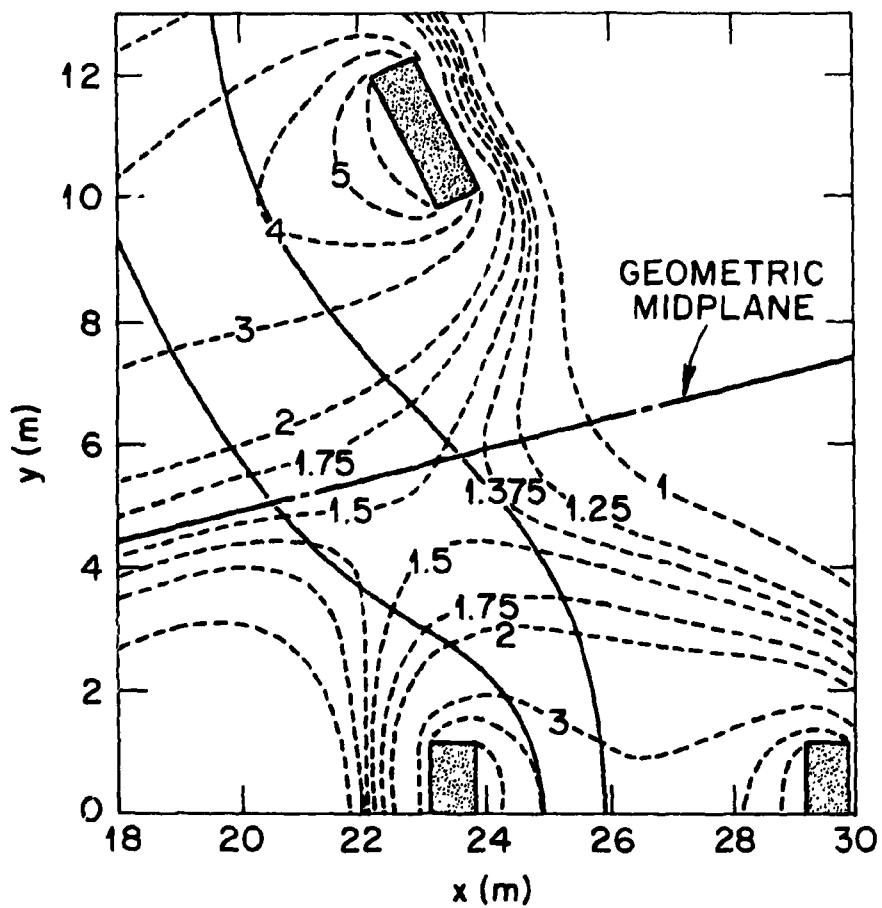
Fig. 9.8. Mod-B contours (dashed) and limiting field lines (solid) in the equatorial plane for an R_T = 23 m EBTEC.
