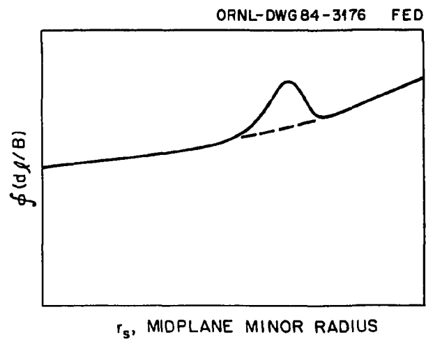
Fig. 4.3. \oint dl/B vs minor radius in the midplane when substantial ring beta occurs. The departure from the vacuum curve (dashed) occurs at radii where ring pressure exists.
