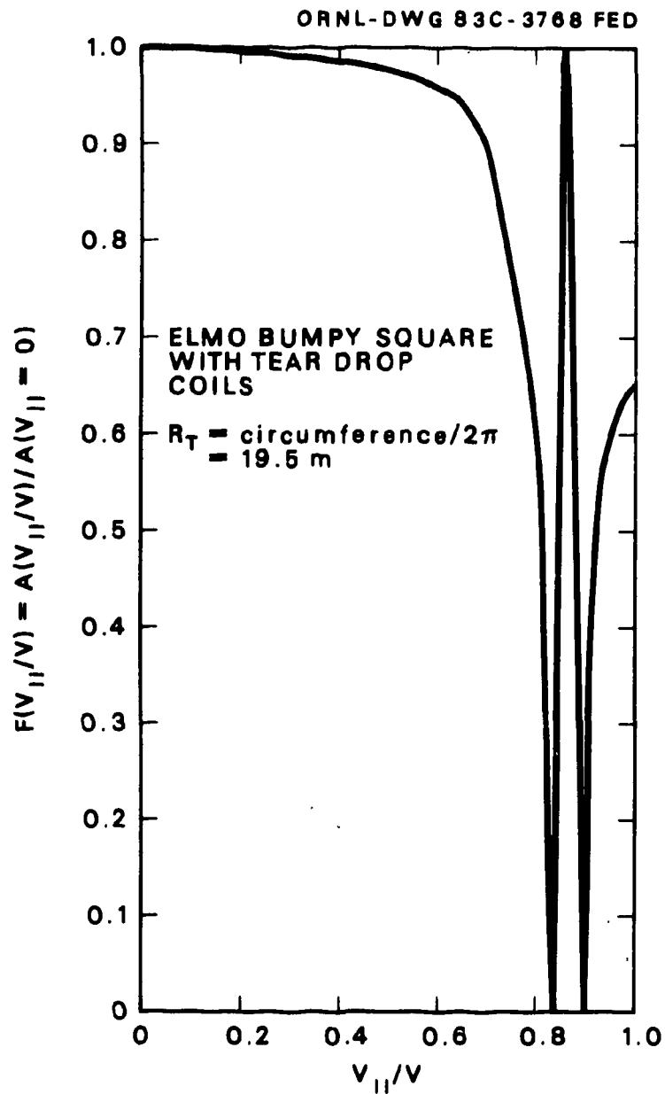
Fig. 9.14. Volumetric efficiency vs pitch angle for a bumpy square configuration shown in Fig. 9.11.
