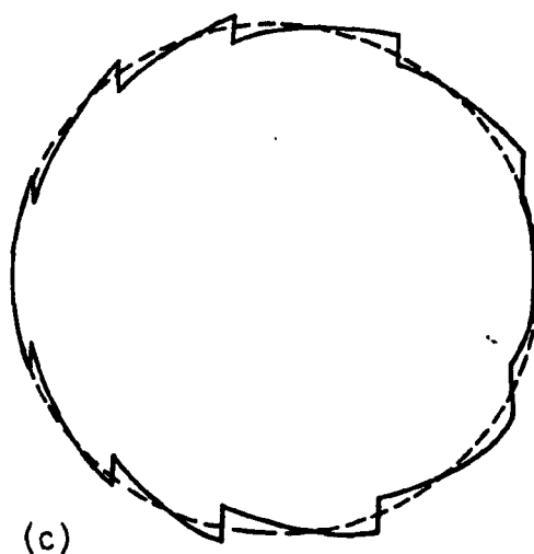
Fig. 4.5(c). The solid curve represents a more complete view of the orbit shown in 4.5(a). In order to make the detailed interaction of sides and corners visible, an exceedingly large gyro radius has been used in 4.5(a), (b), and (c). More typically, one complete toroidal circuit consists of thousands of line segments and circular arcs and is indistinguishable to the eye from the continuum limit described by the longitudinal adiabatic invariant J (dashed).
