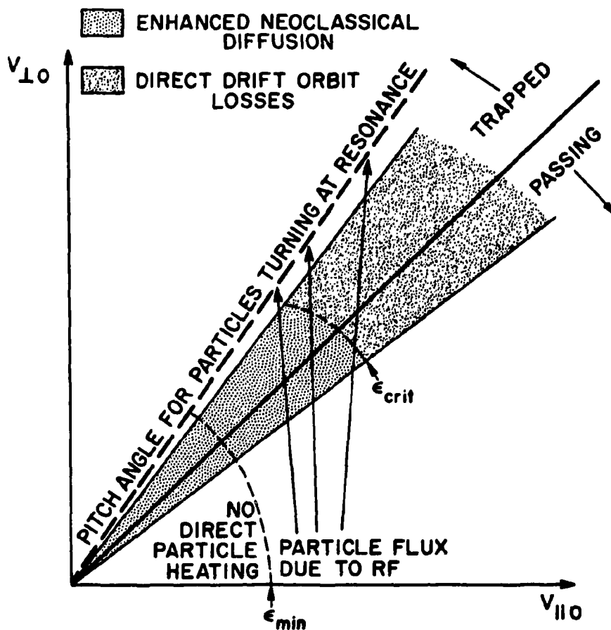
Fig. 7. Velocity space geometry for ECH-enhanced neoclassical transport and direct particle loss in EBT.
