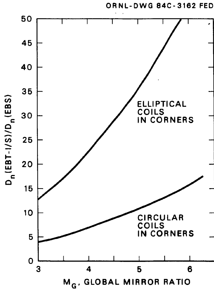
Fig. 1.12. EBS transport coefficients are seen to improve roughly as the inverse square of the global mirror ratio M_G . For the configuration with circular coils in the corners, available dc power and ECH frequencies should permit about a factor of 4 variation in the neoclassical transport rates.
