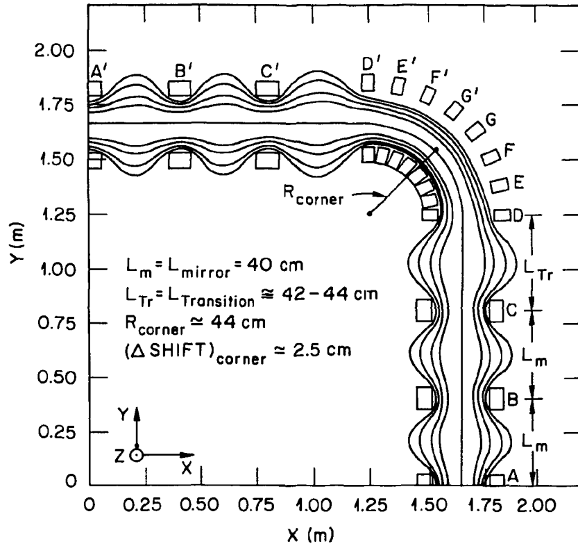
Fig. 3.2. Magnetic field lines in the equatorial plane (X-Y plane) of an EBS are shown for one quadrant. A through G coils and their mirror images G' through A' are shown along with specific dimensions used in the calculations. Here L_m = mirror sector length, L_{Tr} = transition sector length, R_{\text{corner}} = radius of the corner, and (\Delta \text{shift})_{\text{corner}} = (\text{center of coil D} - \text{center of coil A}) = X_{D0} - X_{A0} .
