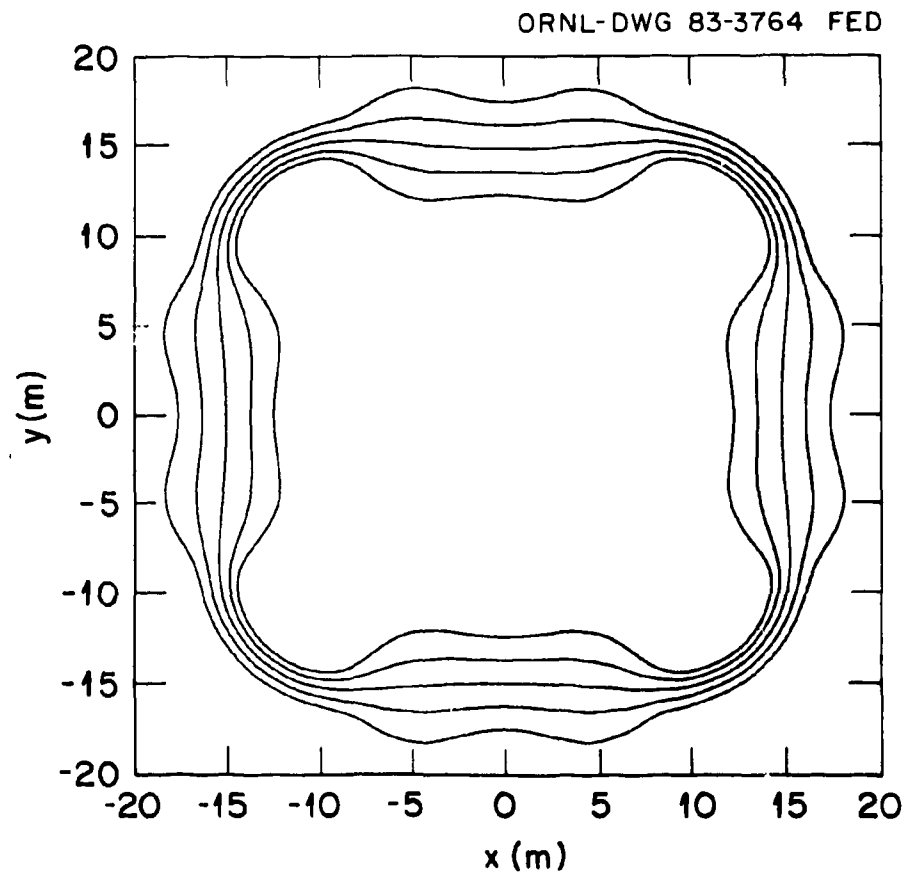
Fig. 9.9. Equatorial plane, field line drawing of an R_T = 17.5 m bumpy square with horizontal Andreoletti coils in straight sections.
