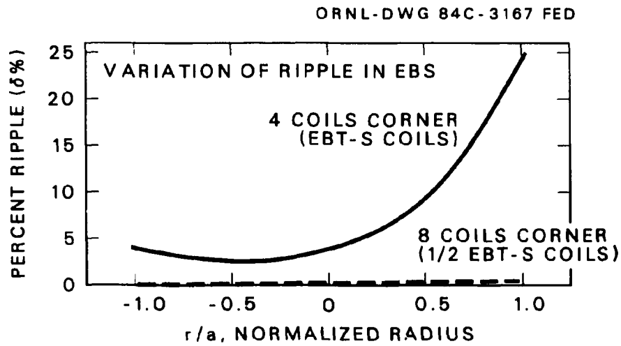
Fig. 2.6. Variation of ripple amplitude \delta as a function of radius for (a) four coils per corner (solid line) and (b) eight coils per corner (dashed line).
