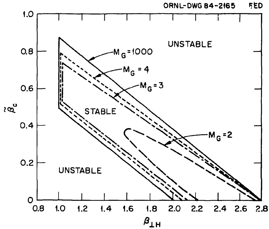
Fig. 5.1. Stability boundaries in the ELMO Bumpy Square vs \tilde{\beta}_{\perp H} and for several values of M_G ( = B_{\text{corner}}/B_{\text{midplane}} ).
