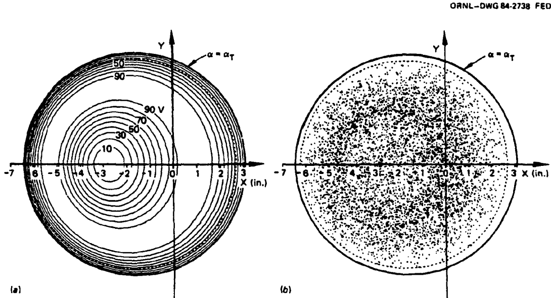
FIG. 6. Potential contours (with contour values shown in volts) and the associated long-time particle motion in EBT for the case of closed symmetric potential contours having no island structure.
