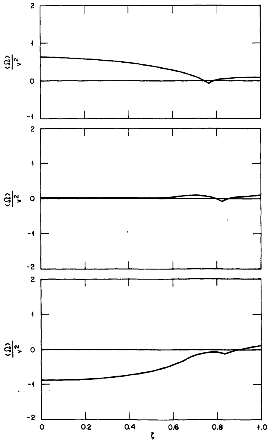
Fig. 7.1. Bounce-averaged drift frequency vs pitch angle ( \zeta = \cos V_{\parallel}/V ) for three different values of ring beta, \beta_{\text{Hot}} . \beta_{\text{Hot}} = 0 (top), small \beta_{\text{Hot}} (middle), and large \beta_{\text{Hot}} (bottom).
