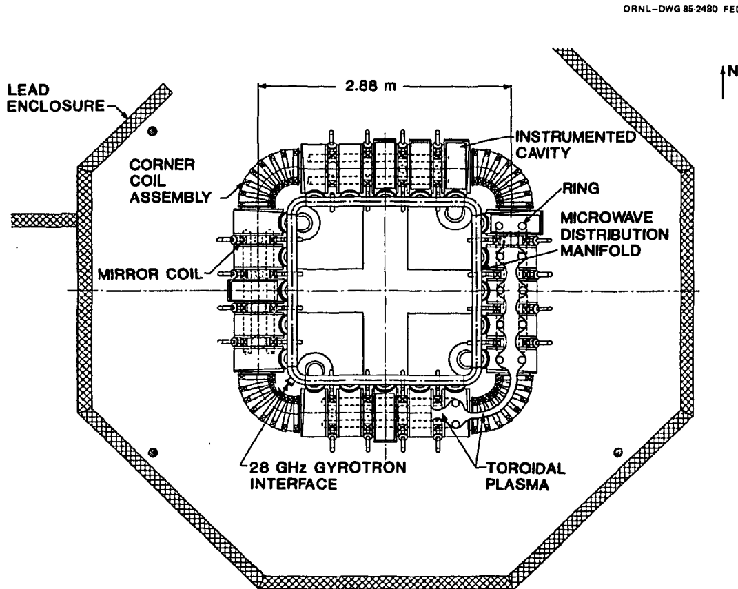
Fig. 2. Plan view of an EBS device within the lead-walled biological shield enclosure originally used for EBT.
