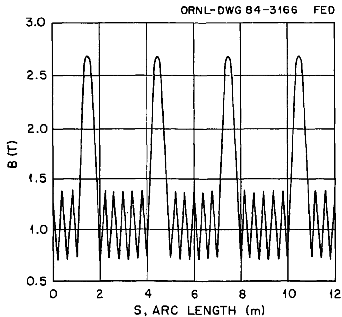
Fig. 2.5. Magnetic field strength as a function of arc length along the magnetic axis for an eight-coil per corner EBS (Fig. 2.3.).
