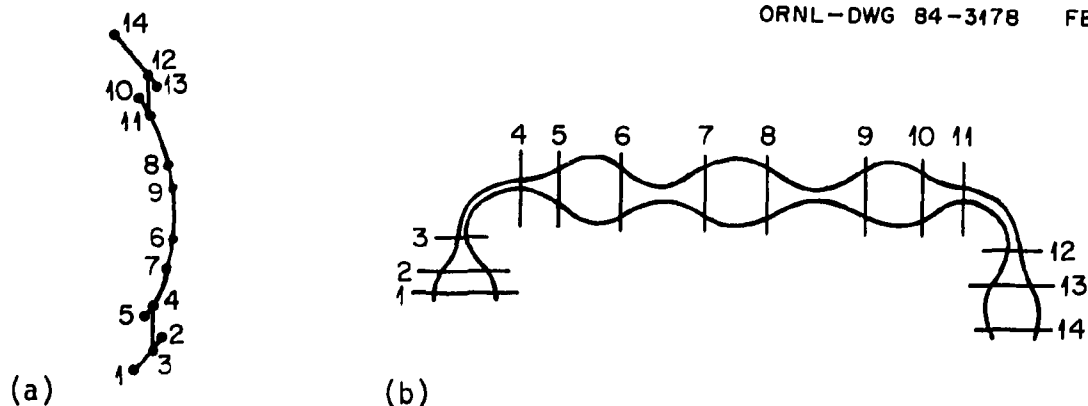
Fig. 4.5. (a) To depict the drift motion of a high energy passing particle, it is convenient to project the orbit into a single plane via field lines. (b) It is also helpful to simultaneously follow the motion parallel to the field lines. The numbers in (a) and (b) refer to times ( t_1 < t_2 < \dots < t_{14} ). At the spatial points corresponding to these times the character of the curvature (b) and curvature drift changes. Between 3 and 4 the particle drifts vertically in a corner (and again between 11 and 12). Along the sides a passing particle rotates in opposite directions as it experiences different signs of curvature - indicated on the circular arcs in (a).
