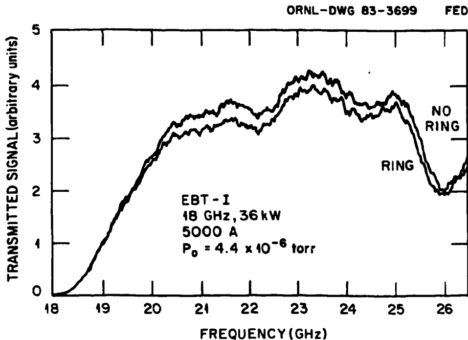
Fig. 3. Microwave transmission through a cavity midplane with and without a ring present.
