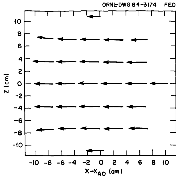
Fig. 3.5. Arrow plot showing the direction and relative magnitude of field line displacements in the plane of A coil for \Delta\phi = 1^\circ . The largest magnitude is 2.81 mm at the coil center (0,0).
