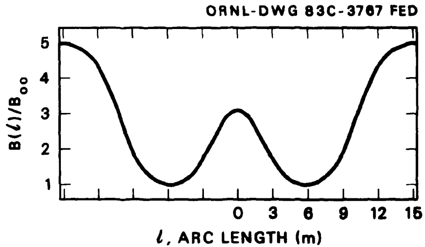
Fig. 9.13. Variation of the magnetic field as a function of arc length along the magnetic axis for one quadrant of a bumpy square configuration shown in Fig. 9.11.
