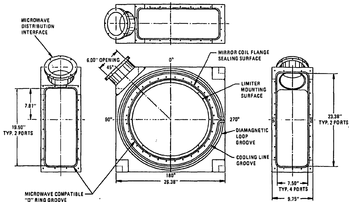
Fig. 20. Detail of instrumented diagnostic microwave cavity.
