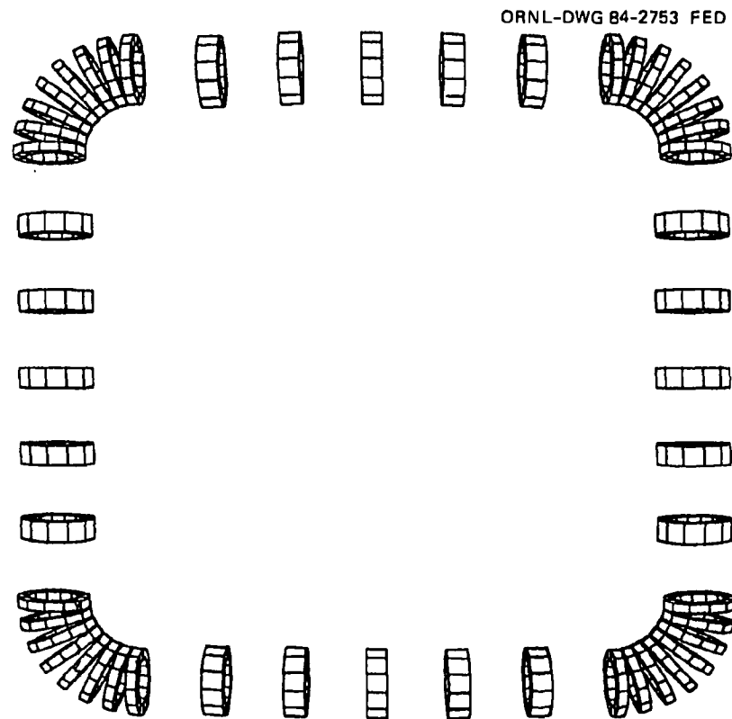
Fig. 2.1. Geometry of an EBS configuration (top view of coil arrangement).
