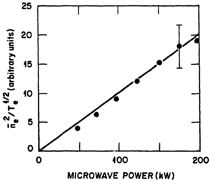
Fig. 2. \bar{n}_e^2/T_e^{1/2} as determined from midplane soft X-ray vs microwave power.
