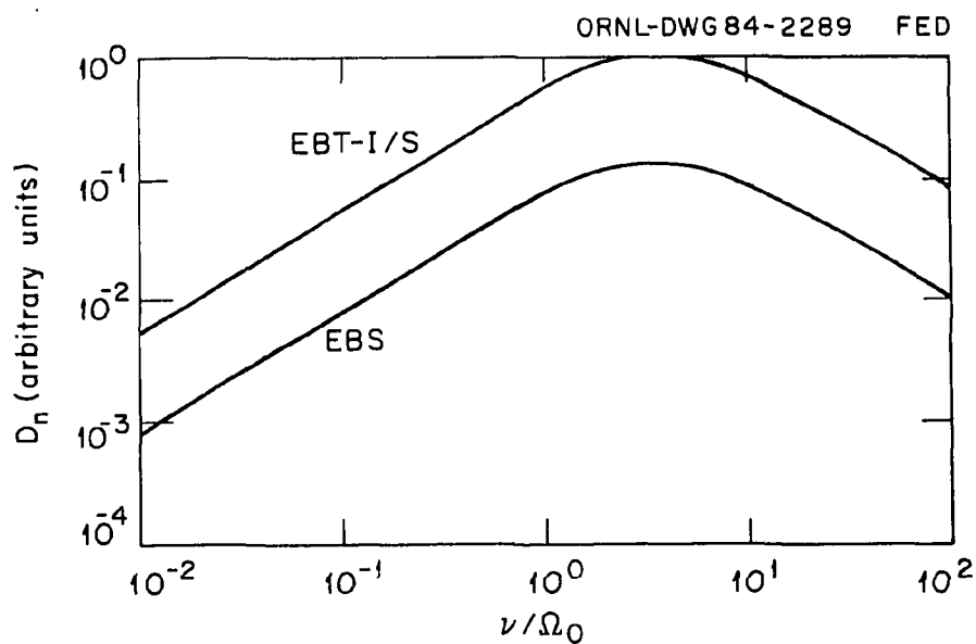
Fig. 1.11. The particle transport coefficient D_n is plotted as a function of collisionality \nu/\Omega_0 for EBT-I/S and for the EBS configuration with circular coils in the corners and M_G \approx 4 . Similar curves are obtained for D_T , K_n , and K_T , with the ratio of the transport coefficient for EBS to that for EBT-I/S approximately the same in each case.
