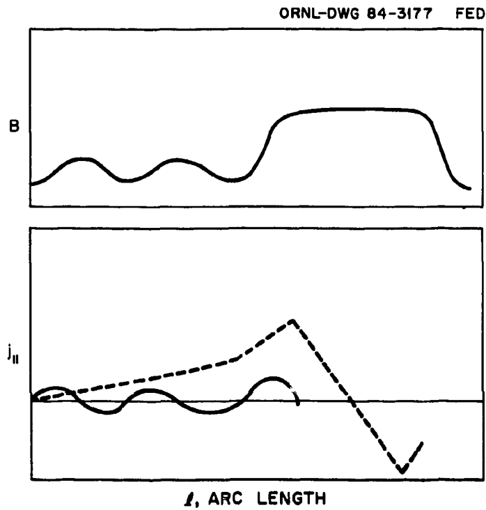
Fig. 4.4. Variation of B and j_{\parallel} vs arc length l . The oscillatory part of j_{\parallel} (solid curve) also occurs for the circular configuration. The other part of j_{\parallel} occurs in polygonal configurations such as the square. The zeros in j_{\parallel} occur at symmetry planes.
