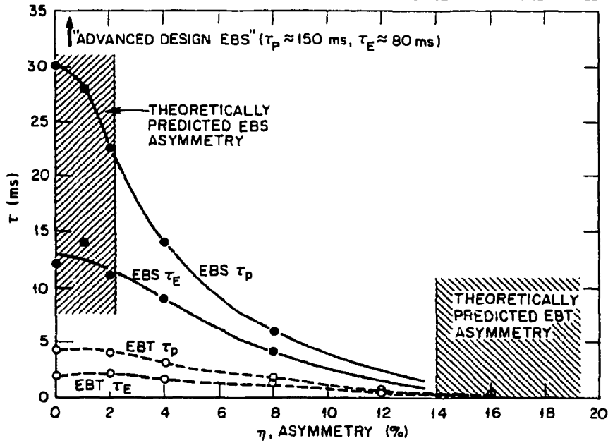
FIG. 8. Particle and energy confinement times for electrons in EBT and a minimal EBS design as functions of the asymmetry parameter \eta . The confinement times for an "advanced design EBS" are off the scale of this plot.
