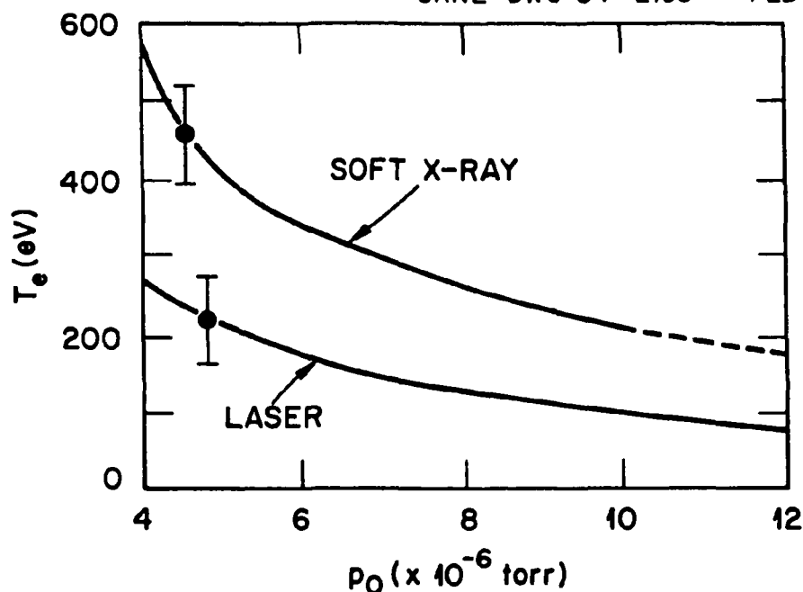
Fig. 5. Core electron temperature as determined by midplane soft X-ray and laser Thomson scattering vs torus field pressure.
