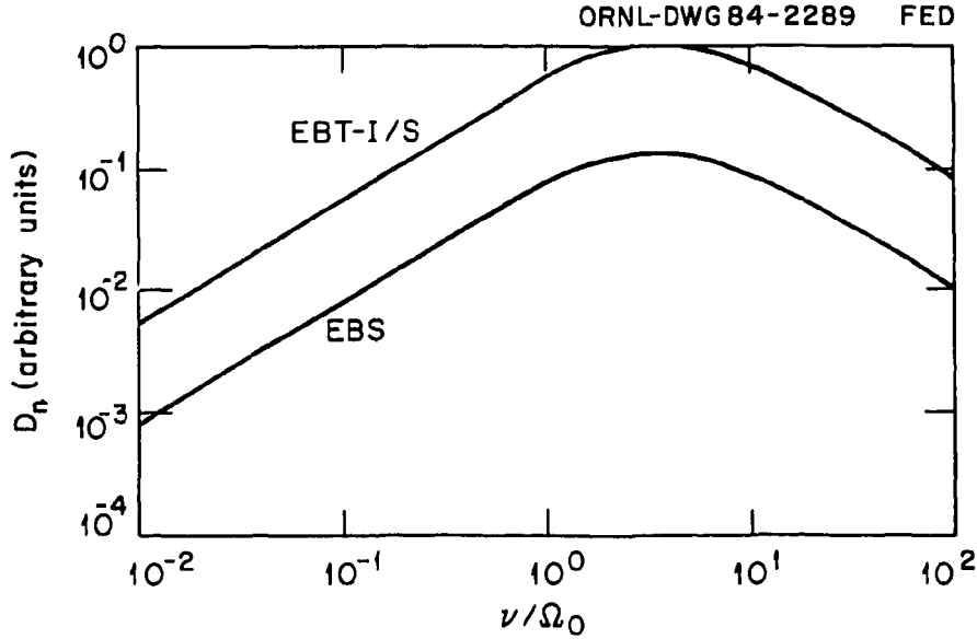
Fig. 5. Particle transport coefficient D_n as a function of collisionality \nu/\Omega_0 for EBT and EBS. Similar curves are obtained for D_T , K_n , and K_T with the same ratio of improvement in EBS over that in EBT. [Note that \tau(\text{EBS})/\tau(\text{EBT}) \sim D(\text{EBT})/D(\text{EBS}) \sim 5\text{--}15 .]
