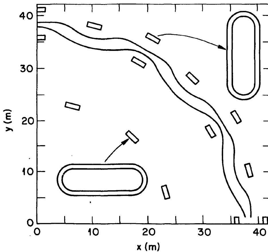
Fig. 9.2. One quadrant of an R_T = 35 m EBTEC projected onto the equatorial plane, with two magnetic lines of force and orientation of coils shown.
