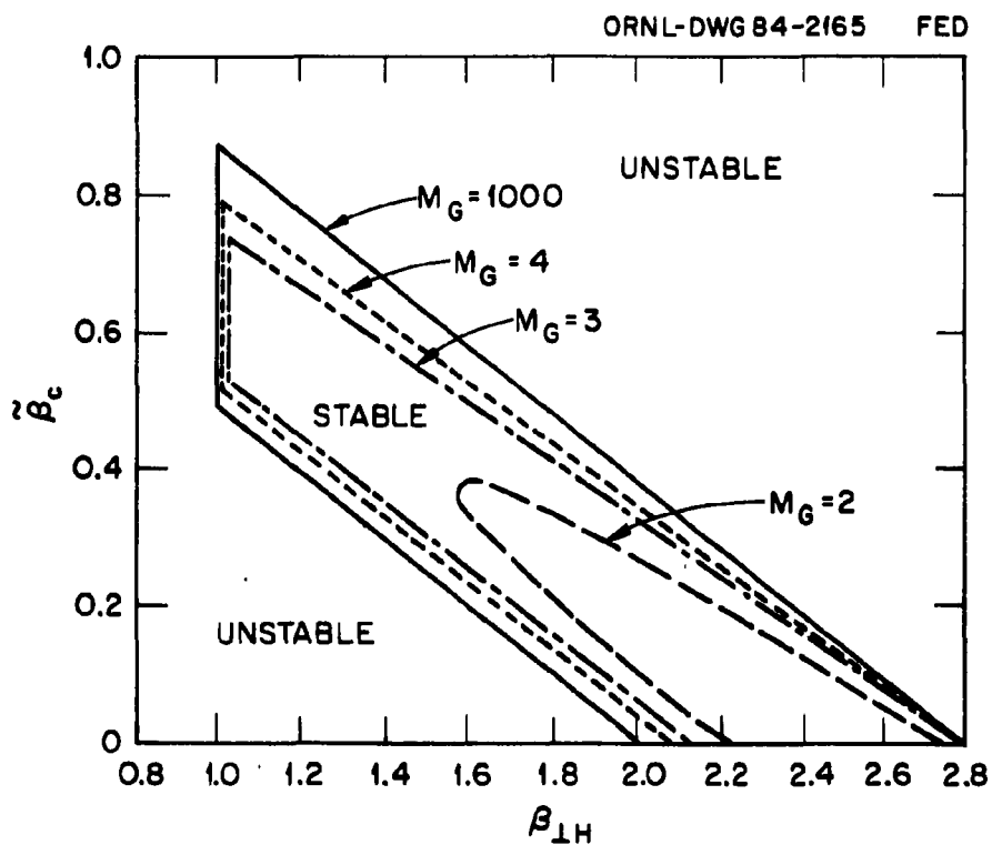
Fig. 7.4. Stability boundaries in the \tilde{\beta}_c vs \tilde{\beta}_{\perp H} plane for several values of global mirror ratio M_G .
