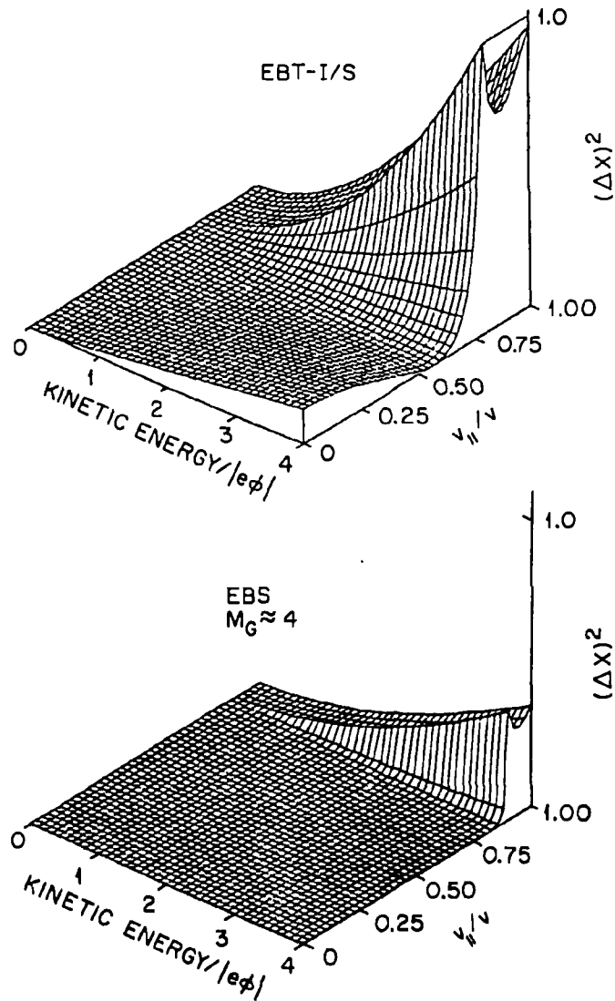
Fig. 4.10. Square of the displacement from the mean, (\Delta X)^2 , vs kinetic energy and (v_{||}/v)_{\text{midplane}} . The nonzero electrostatic potential was chosen to confine particles at low energy for both configurations. Note that the deviation from the mean is considerably suppressed by the square configuration.
