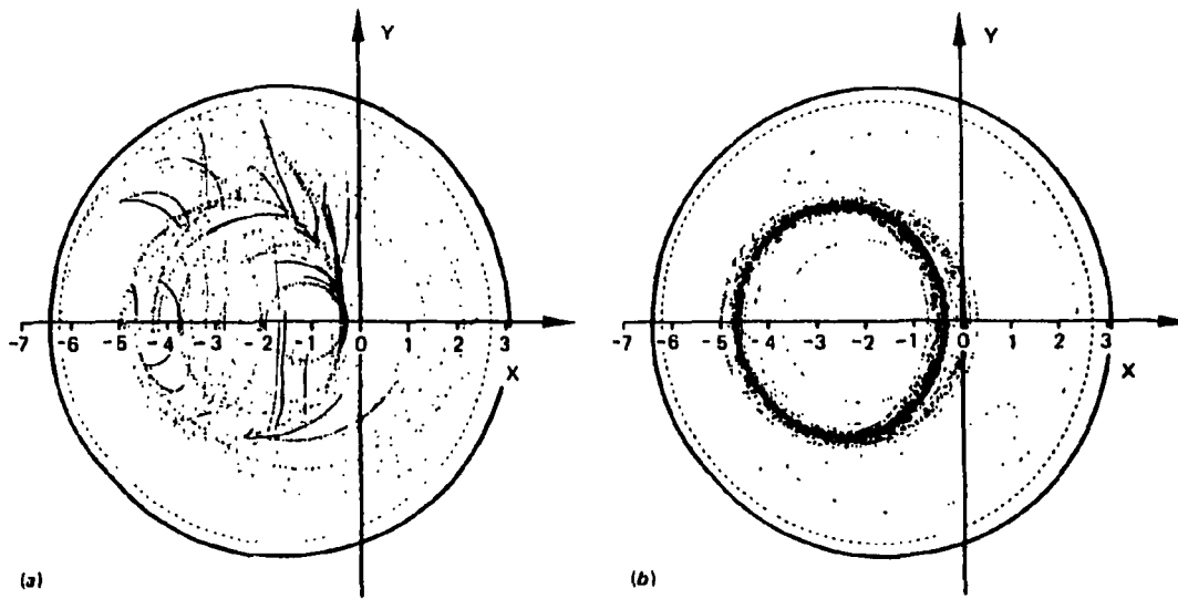
FIG. 2. Multiple exposure ( \alpha, \beta ) coordinates (projected to the midplane and transformed to real cartesian space) depicting the orbits of 64 Monte Carlo test electrons without collisions in EBT-I/S (a) with no electric field and (b) with a purely radial radial electric field (with \Delta\Phi = T_e ).
