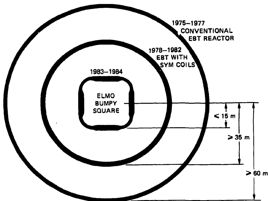
Fig. 10. Trend to smaller EBT reactor systems, which is exploited by EBS. Relative dimensions of EBT reactor configurations are shown, with corresponding years of development.
