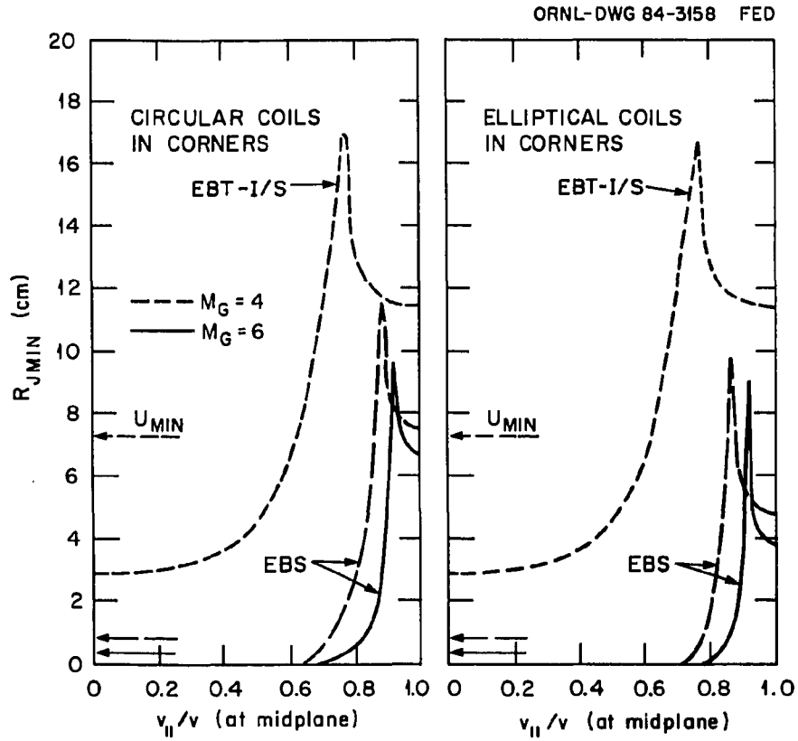
Fig. 1.8. R_{JMIN}(V_{||}/V) and the radial position of the minimum of \oint dl/B \equiv U_{MIN} for EBT-I/S and EBS with circular and elliptical coils in the corners for two values of the global mirror ratio.
