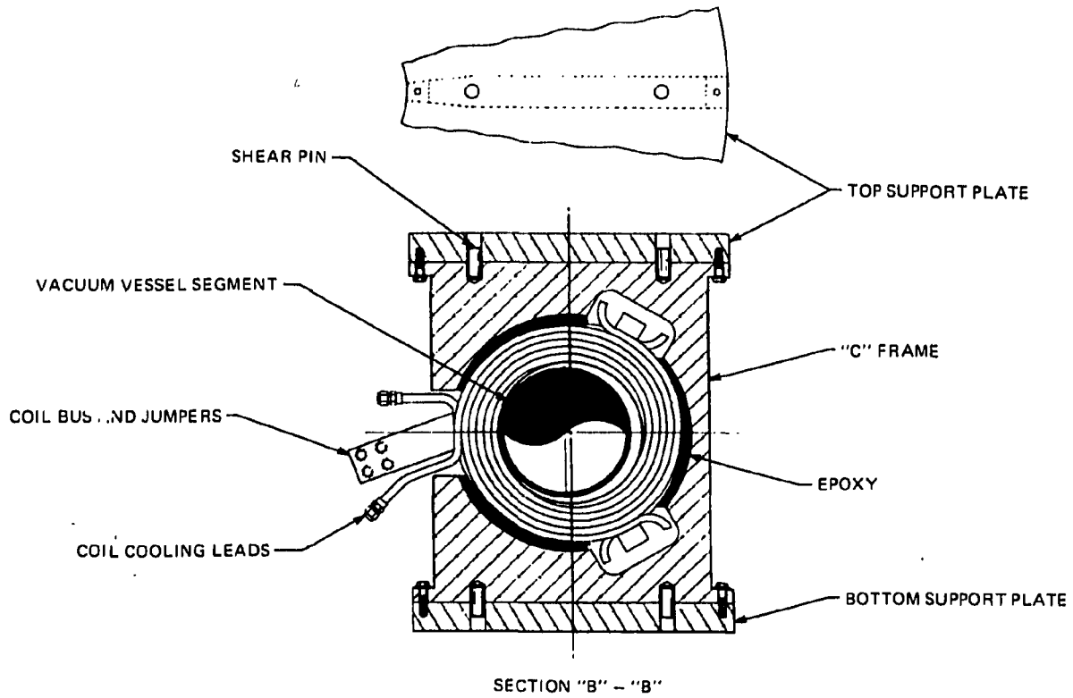
Fig. 21. Detail of support structure and cooling for standard corner coil.
