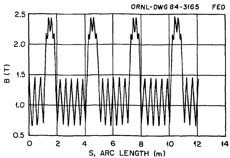
Fig. 2.4. Magnetic field strength as a function of arc length along the magnetic axis for a four-coil per corner EBS (Fig. 2.2).
