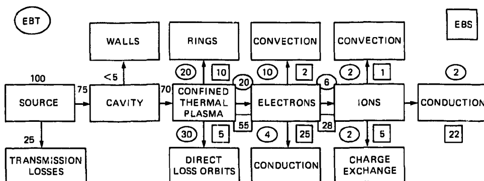
Fig. 11. Schematic power flow diagram for EBS and EBT. Parasitic side losses are substantially reduced in EBS. The numbers are percentages of the microwave source output power; EBT data are enclosed in circles and EBS data in squares.
