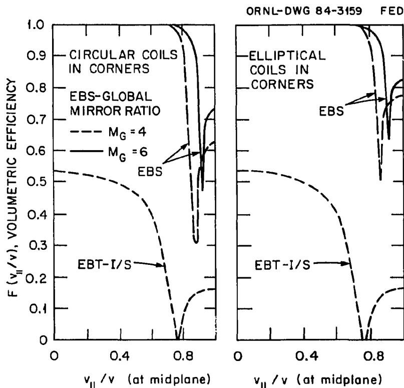
Fig. 1.7. Volumetric efficiency curves for EBT-I/S are compared to those for EBS configurations with circular and elliptical coils in the corners for two values of the global mirror ratio. The cosine of the pitch angle ( v_{\parallel}/v ) is defined at the center of the reference midplane.
