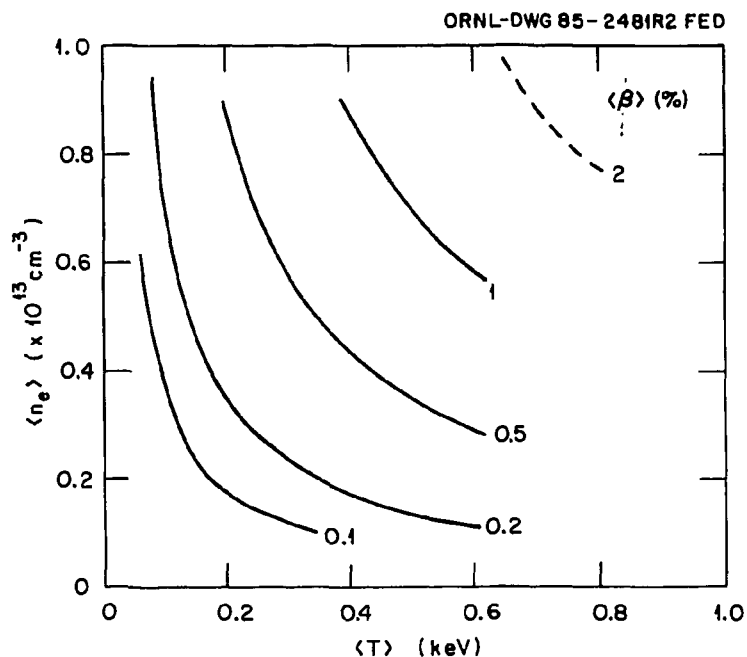
Fig. 13. WHIST code plasma operation contours, showing the beta values achieved during operation at full field.
