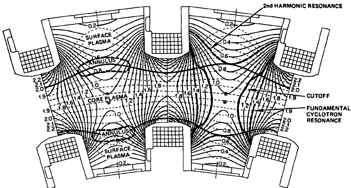
Fig. 1. Equatorial cross section of two EBT-S cavities.
