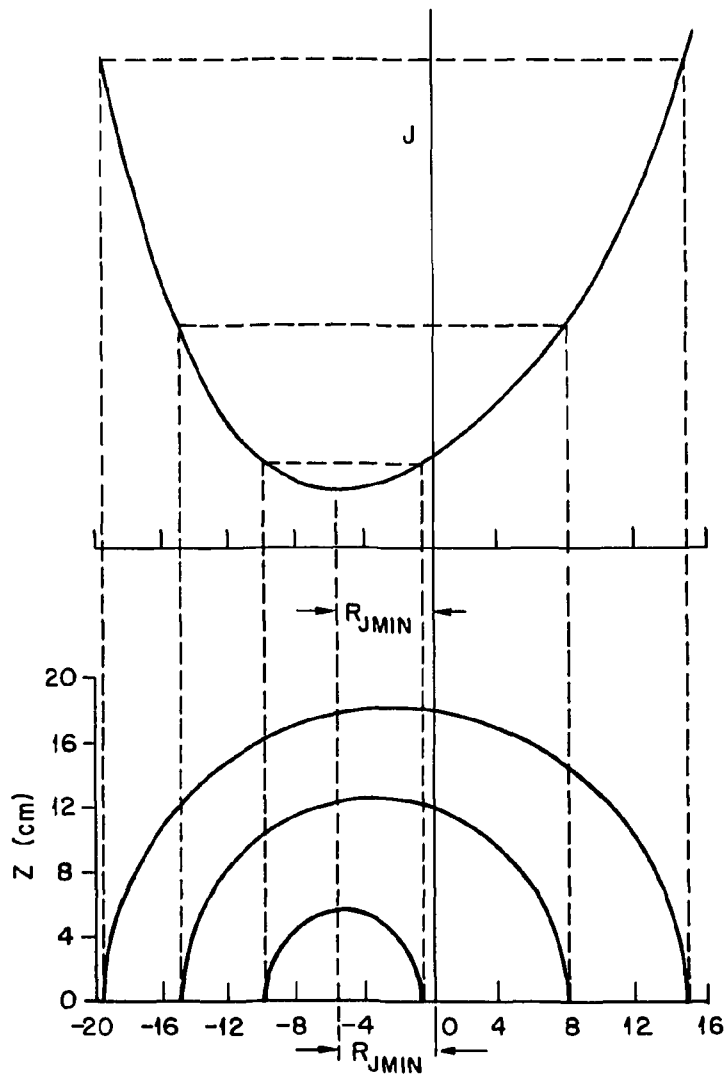
Fig. 1.5. R_{JMIN} is a useful measure of drift orbit dispersion in the plasma interior. It represents the radial distance from the minor axis of the center of that drift orbit (for a particular pitch angle) which has the largest inward shift toward the major axis of the torus.
