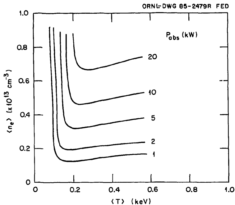
Fig. 12. WHIST code plasma operation contours. The contours show the amount of power that must be delivered to a confined plasma in order to achieve operation at any point in the plane of average density vs temperature. The entire area is predicted to be accessible with the available power, subject to limitation by cutoff at a density of 10^{13} \text{ cm}^{-3} .
