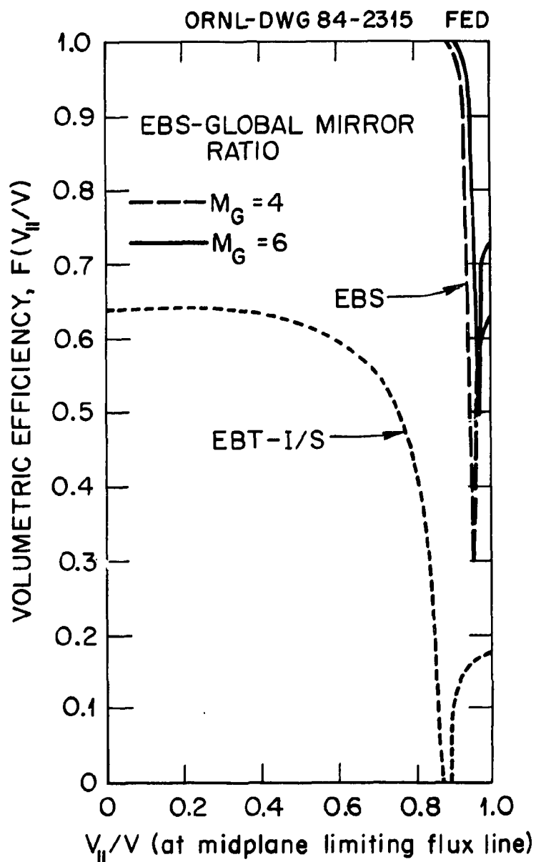
Fig. 4. Volumetric efficiency curves for EBT and EBS as a function of pitch angle at the limiting flux line in the midplane. These show containment of more than 95% of the particle in EBS, compared with \sim 50\% in EBT. (That is, the direct loss fraction is less than 5% in EBS and \sim 50\% in EBT for vacuum fields.)
