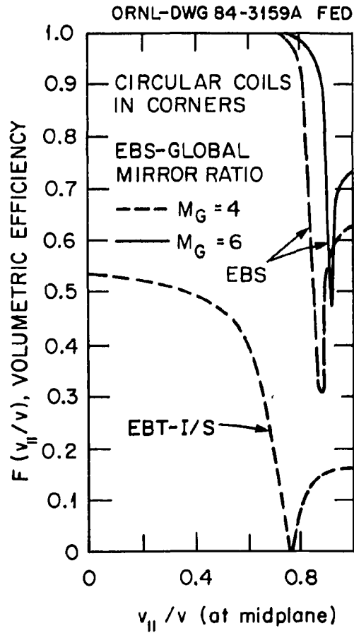
Fig. 4.9. Volumetric efficiency vs (v_{||}/v)_{\text{midplane}} for circular EBT-I/S (short dashes) and square configuration (solid curve is for M \approx 6 and long dashes for M_G \approx 4 ). The normalization chosen is F = (\text{drift orbit area})/(\pi r_{\text{limiter}}^2) . In all cases r_{\text{limiter}} = 19.5 \text{ cm} .
