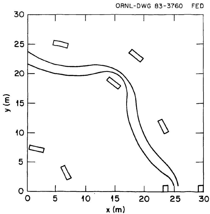
Fig. 9.5. One quadrant of a 14-sector EBTEC reactor.
