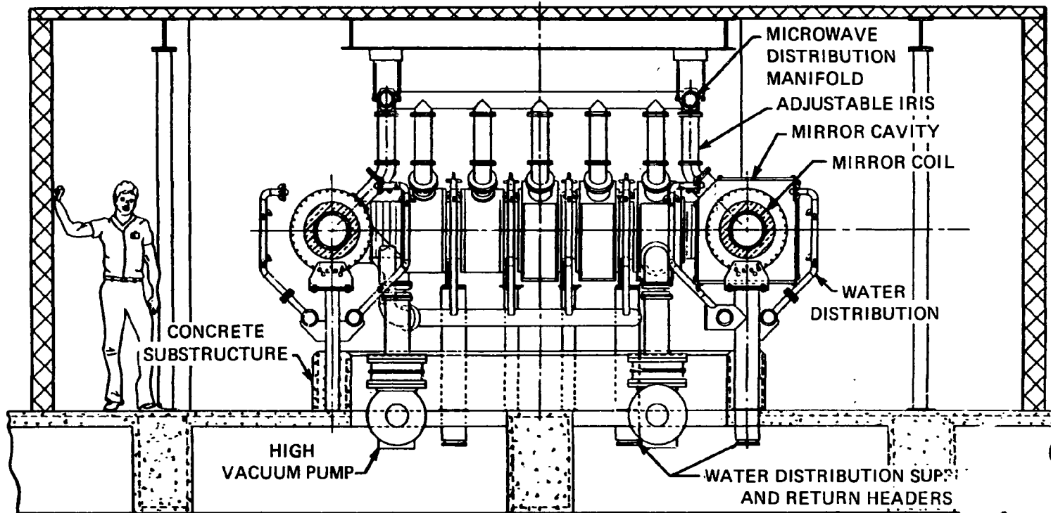
Fig. 16. Elevation view of EBS.
