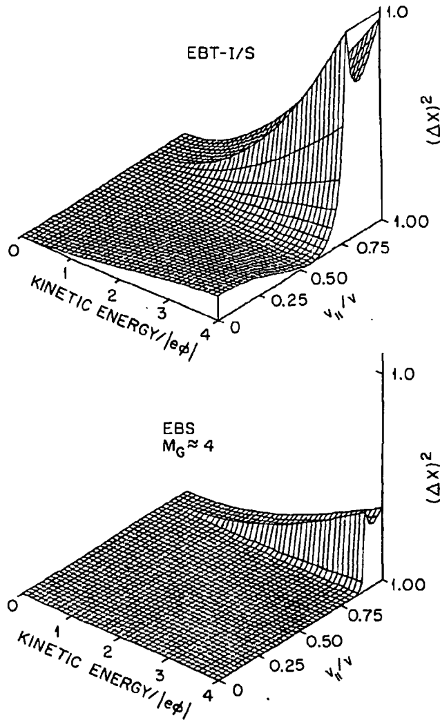
Fig. 1.9. Isometric plots of the square of the diffusion step-size for EBT-I/S and the EBS configuration with circular coils in the corners are displayed as a function of v_{||}/v and the ratio of particle kinetic energy to ambipolar potential well depth. |e\phi|/kT \approx 1 is assumed.
