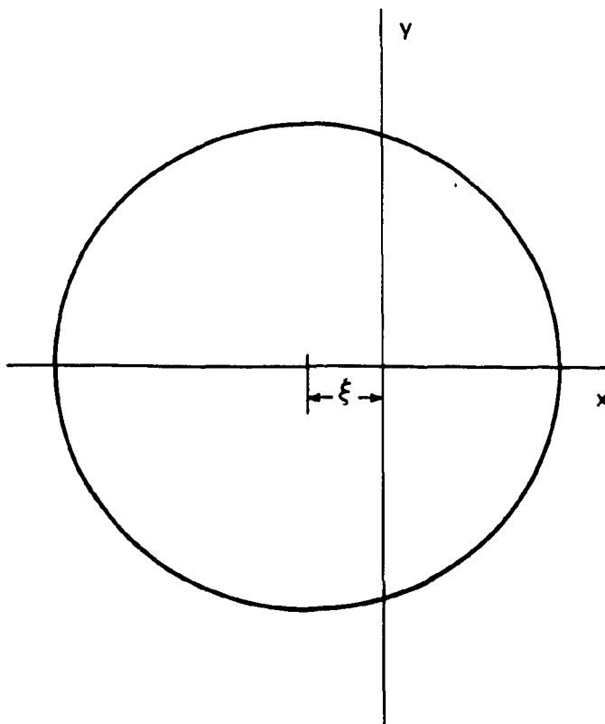
Fig. 4.2. Pressure surface in the midplane of one of the mirror cells composing the sides of the square configuration. Since pressure is constant along field lines, the pressure surface follows field lines, contracting in cross-sectional area in regions of higher magnetic field. For both circular and square configurations \xi is reduced with increasing local mirror ratio (bumpiness) and number of mirror cell. The additional dependence of \xi on global mirror ratio for the square configuration is exploited to reduce the inward shift of the pressure surface.
