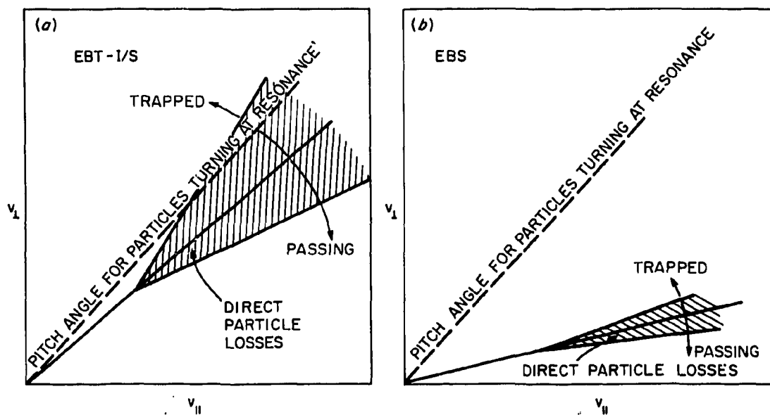
Fig. 9. Heating zone (pitch angle for particles turning at resonance) for (a) EBT and (b) EBS.
