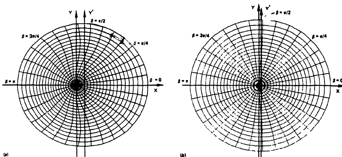
FIG. 4. Contours of constant \alpha and \beta for (a) a "minimal" EBS design with 4 coils per side and a global mirror ratio of 3.7 and (b) an improved EBS with 6 coils per side and a global mirror ratio of 6.4.
