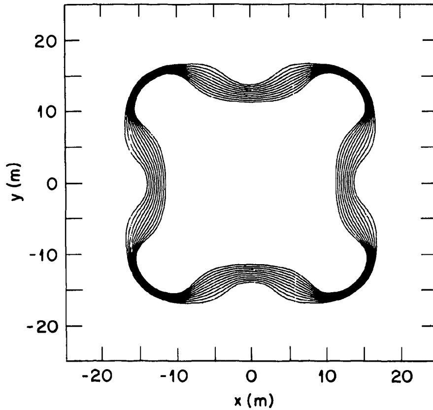
Fig. 9.11. A field line drawing of a bumpy square with horizontal "teardrop" coils in straight sections. Equivalent major radius R_T \simeq 19.5 m.
