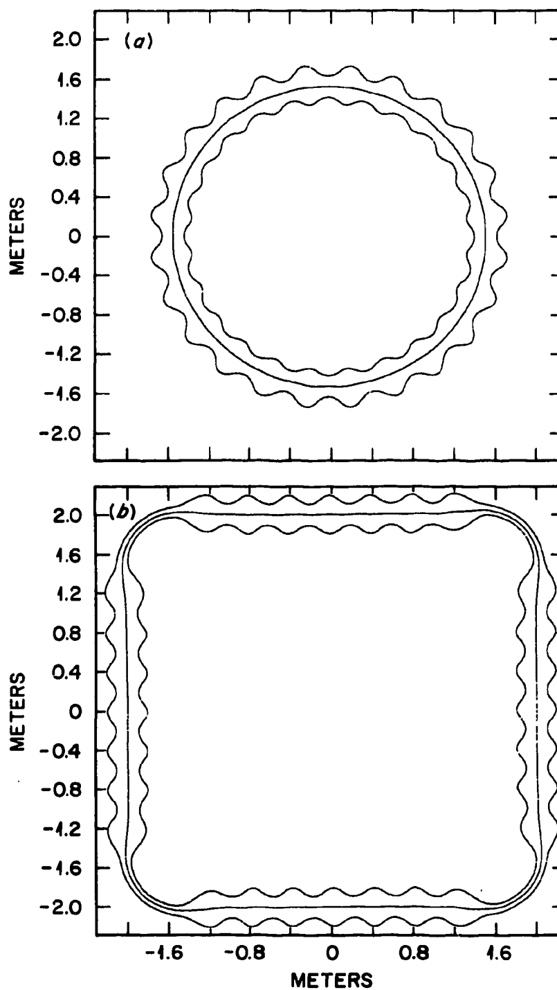
Fig. 4.1. Circular (EBT-I/S) and square (EBS) configurations of EBT.
