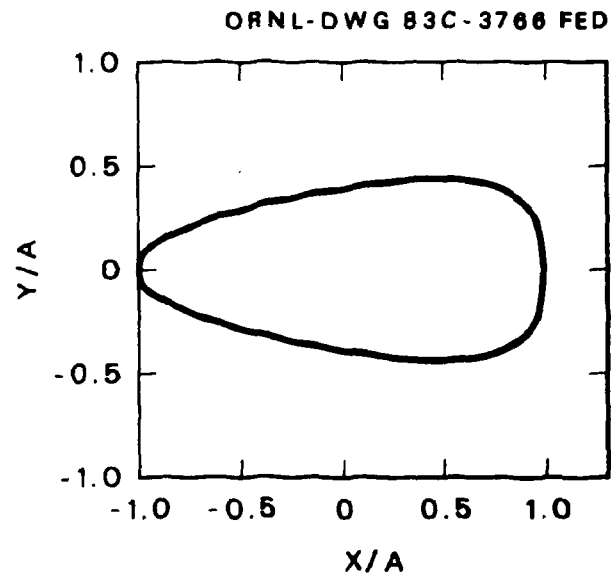
Fig. 9.12. Shape of the "teardrop" coil.
