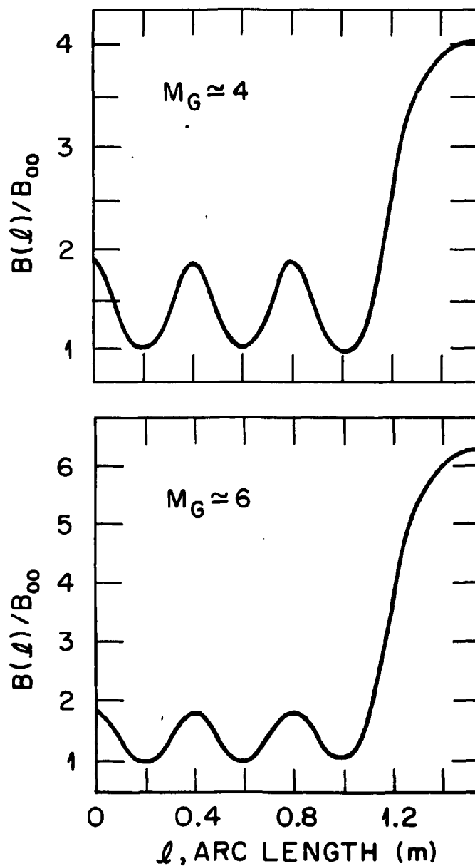
Fig. 1.3. The normalized magnetic field strength is plotted along the central field line in EBS for two values of the global mirror ratio M_G ; M_G = 4 (top) and M_G = 6 (bottom).
