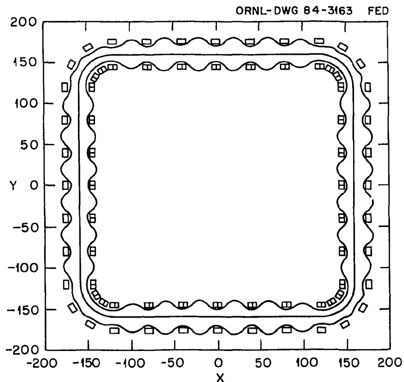
Fig. 2.2. Magnetic field lines in the equatorial plane of an EBS with a four-coil corner. Each side of the EBS configuration consists of a linear array of five EBT-I/S mirror coils, and the corners are formed by 90° sections of toroidal solenoids in which the field is produced by four EBT-I/S mirror coils. Current in straight section coils is 7.25 kA and in the corner coils 9 kA.
