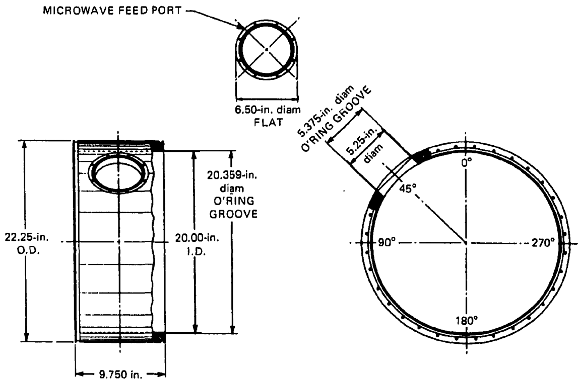
Fig. 19. Detail of standard microwave cavity.
