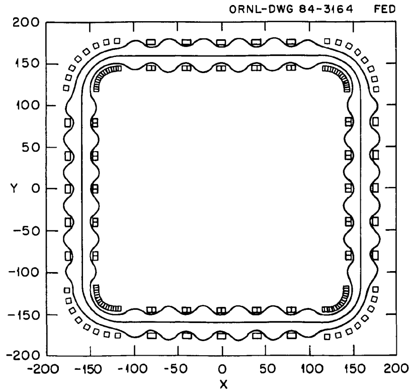
Fig. 2.3. Magnetic field lines in the equatorial plane of an EBS with eight coils per corner. The corner field is produced by eight half-size (ampere-turns) EBT-I/S coils. Total ampere-turns are the same as in Fig. 2.2.
