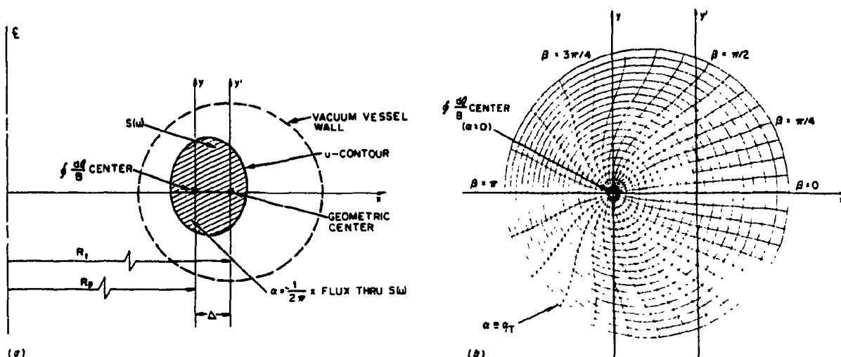
FIG. 1. (a) Schematic geometry of a u = \oint dl/B pressure surface in an EBT midplane and its relation to the geometric center of the magnetic field coils. The major radius of the torus, R_t , measures the distance from the torus centerline to the geometric center, and R_p is the distance from the centerline to the \oint dl/B center. S(u) is the surface enclosed by the u = \text{constant} contour, and 2\pi\alpha is the magnetic flux through S(u) . (b) Contours of constant \alpha and \beta for EBT-I/S. In both (a) and (b), the cartesian (x, y) axes have their origin at the \oint dl/B center, and the y' -axis passes through the geometric center.
