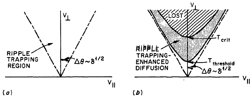
Fig. 2.8. (a) Ripple loss region and (b) critical energies.
