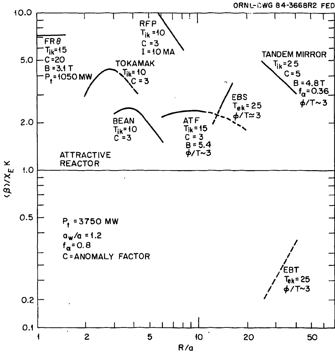
Fig. 14. Neoclassical predictions for attractive reactors. The EBS margin of safety for achieving attractive reactor performance is of the same order as that of other fusion reactor candidates.
