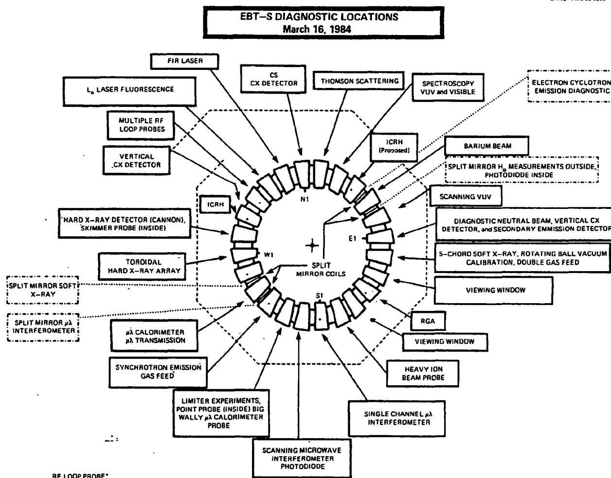
Fig. 15. Schematic diagram of diagnostic devices installed on EBT. A similar array is eventually planned for EBS, although operation will begin with the minimum diagnostic set needed to demonstrate ring stabilization and improved confinement.
