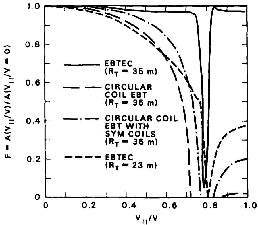
Fig. 9.3. Volumetric efficiency vs pitch angle for an EBTEC reactor ( R_T = 35 m and 23 m) and for a circular coil EBT reactor ( R_T = 35 m) with and without SYM coils.
