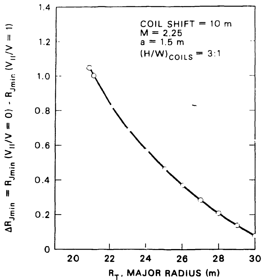
Fig. 9.4. Dispersion in drift orbit centers vs major radius for an EBTEC.
