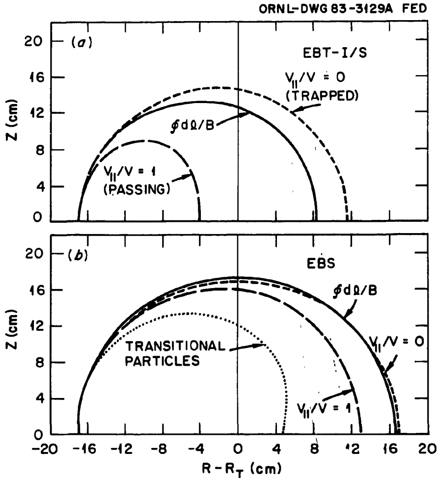
Fig. 3. Drift orbits (dashed lines) and \oint d\Omega/B contours (solid lines) in the reference midplane of EBT (top) and EBS (bottom). Deeply trapped ( v_{||}/v = 0 ), extreme passing ( v_{||}/v = 1 ), and transitional particles near the boundary between the trapped and passing zones (most poorly confined drift orbit) are shown. Transitional particle orbits were absent from EBT (i.e., the worst orbit did not close within the volume) but are reasonably well contained in EBS.
