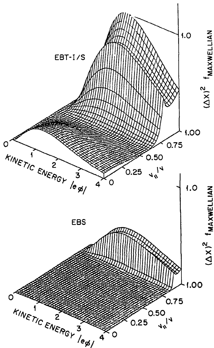
Fig. 4.11. Square of the displacement multiplied by a Maxwellian distribution. The figure indicates the importance of weighting the displacement by the number of particles having that displacement.
