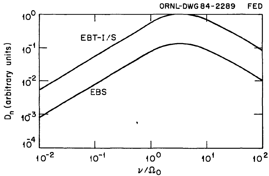
Fig. 4.12. Diffusion coefficient vs collisionality for circular and square configurations. Note that the diffusion is roughly an order of magnitude less for the square configuration. Thus, for similar assumptions for the ambipolar potential, the lifetime is an order of magnitude larger for the square configuration.
