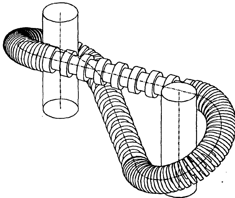
Fig. 9.15. Twisted racetrack configuration.
