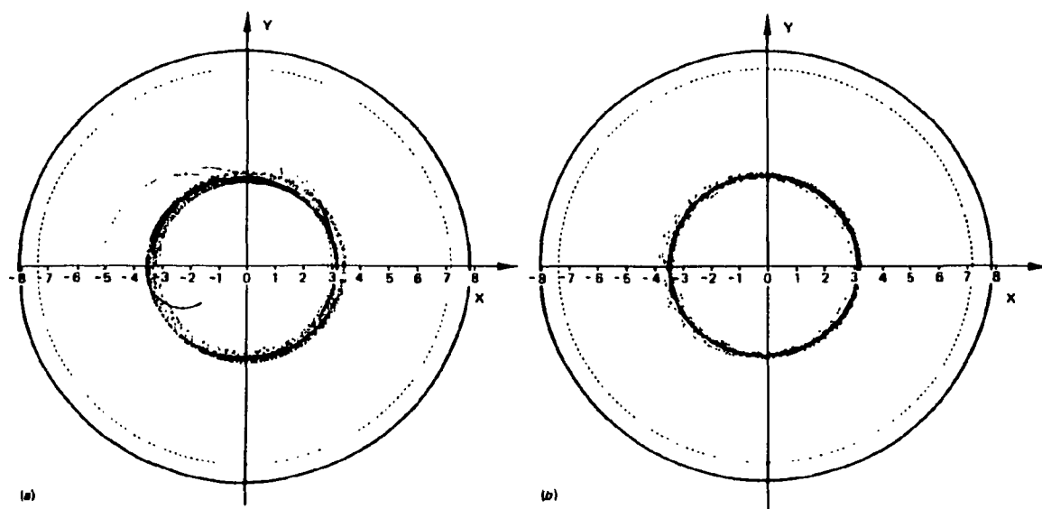
FIG. 5. Multiple exposure positions of 64 collisionless electrons in an EBS (a) with no electric field and (b) with a radial electric field.
