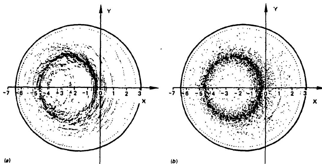
FIG. 3. Multiple exposure positions of 64 test electrons in EBT undergoing e-e and e-i collisions appropriate to about 9 \times 10^{11} \text{ cm}^{-3} background plasma density (a) with no electric field and (b) with a radial electric field.
