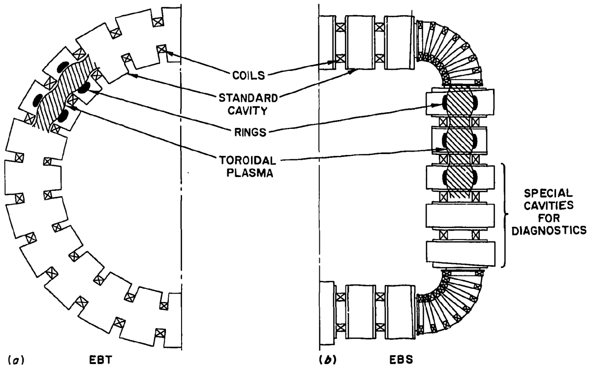
Fig. 1. Top view of the EBT configuration (left) and the EBS reference configuration (right). The diagram shows how the existing EBT mirror coils will be used in the sides of EBS, which will require new corner coils and microwave cavities. There will be 14 standard cavities and 6 instrumented cavities for diagnostics.
