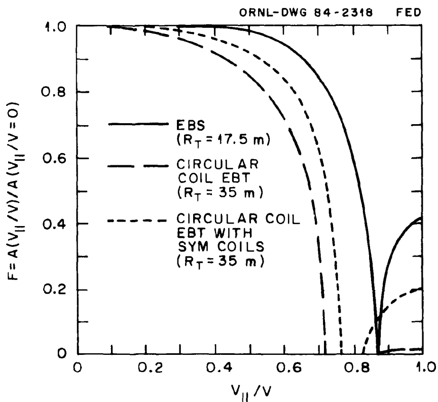
Fig. 9.10. Volumetric efficiency vs pitch angle for an EBS reactor ( R_T = 17.5 m) and for a circular coil EBT reactor ( R_T = 35 m) with and without SYM coils.
