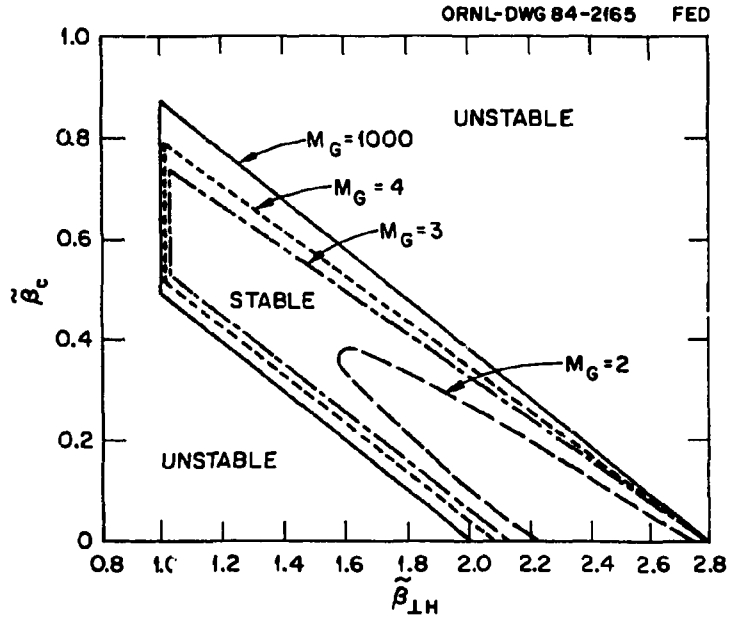
Fig. 8. Stability boundaries in EBS for several values of M_G . Beta values here are scaled to the Lee-Van Dam threshold \beta_0 = 2\Delta r/R_c , where \Delta r is the ring radial width and R_c is the field line radius of curvature in the ring region. Here, \tilde{\beta}_c = \beta_c/\beta_0 and \tilde{\beta}_{\perp H} = \beta_{\perp H}/\beta_0 .
