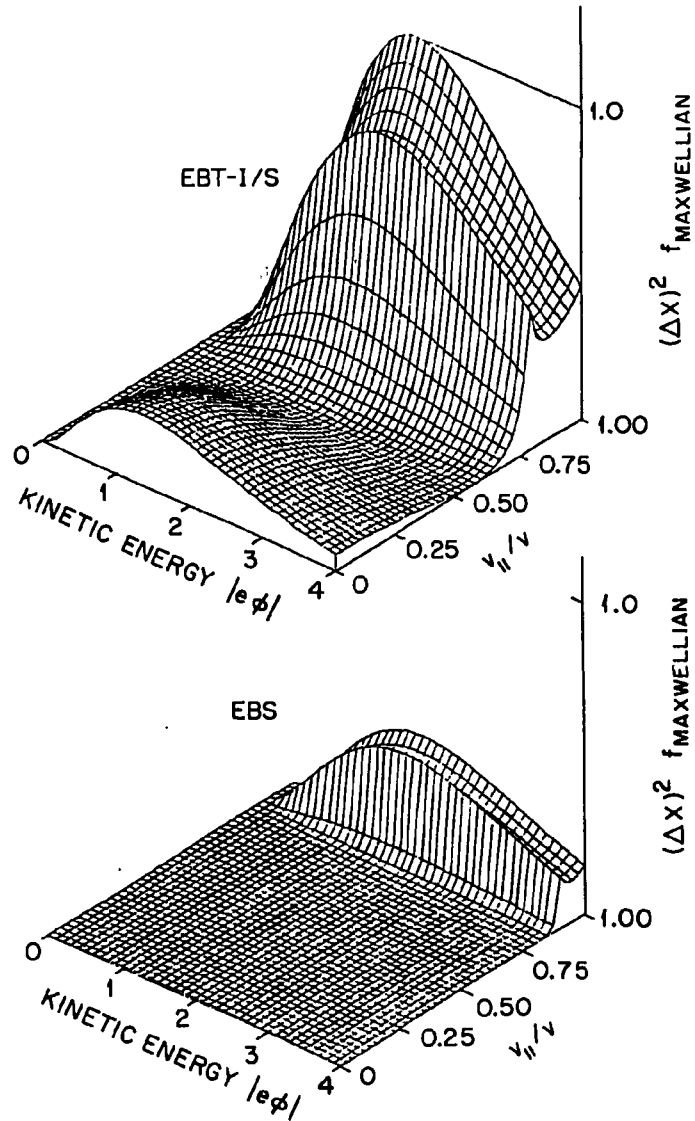
Fig. 1.10. The square of the diffusion step-size, shown in Fig. 1.9, is multiplied by a Maxwellian distribution function.
