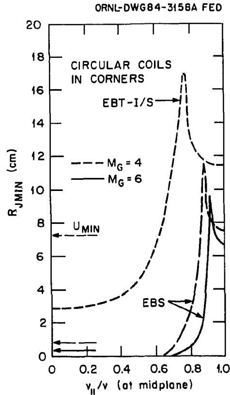
Fig. 4.8. Shift of small radius orbits, R_{JMIN} , vs (v_{||}/v)_{midplane} for high-energy particles. The solid curve represents a square configuration with global mirror ratio M_G \approx 6 , whereas the long dashes indicate the same coils with less current in the corners ( M_G \approx 4 ). The higher curve (short dashes) is for EBT-I/S.
