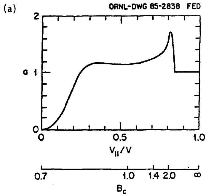
Fig. 2. Anisotropy factor, a , for (a) EBT and (b) EBS. Two scales are used: B_c (normalized to the value of B in the midplane on the magnetic axis) and v_{||}/v = (1 - B_2/B_c)^{1/2} , where B_2 (here equal to 0.7) is the value of B at the second harmonic electron cyclotron resonance. The fundamental resonance of the electron cyclotron resonance occurs at B_c = 1.4 . For EBT the boundary between trapped and passing occurs near B_c = 2 , while for EBS it occurs near B_c = 5 .
