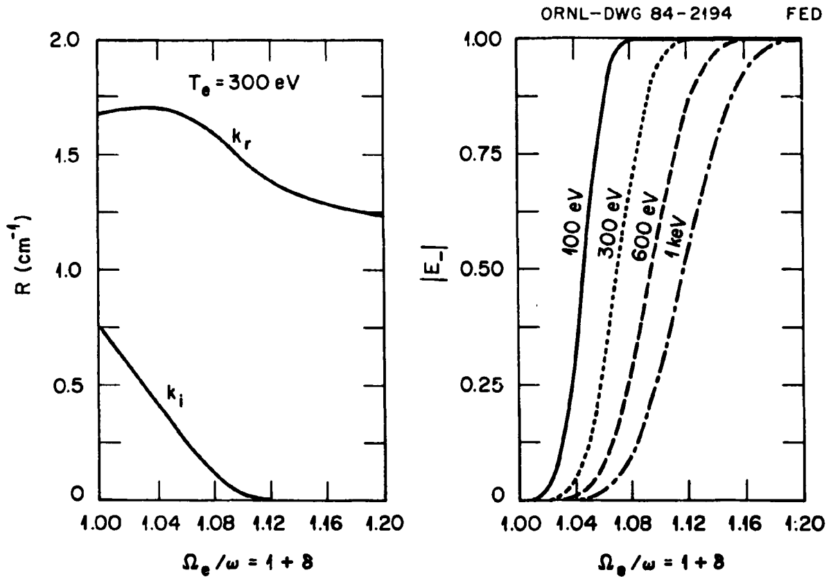
Fig. 6. (a) k -real and k -imaginary vs \Omega_e/\omega for parallel propagating extraordinary mode waves in a 300-eV Maxwellian plasma. (b) Wave power density profiles \propto |E_-|^2 for various plasma temperatures.
