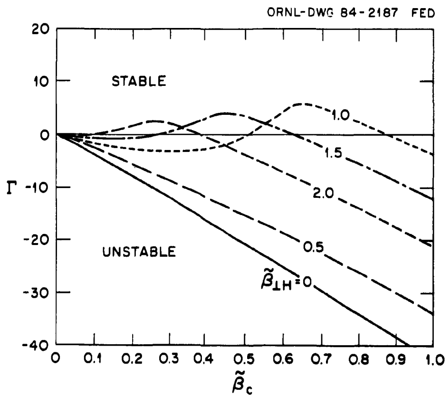
Fig. 7.3. \Gamma vs normalized core beta \tilde{\beta}_c = \beta_c/\beta_{LVDN} for several different values of ring beta \beta_{\perp H} . Note \tilde{\beta}_{\perp H} = \beta_{\perp H}/\beta_{LVDN} .
