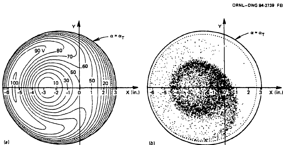
FIG. 7. Asymmetric potential contours in EBT with asymmetry parameter \eta = 16\% producing crescent-shaped potential islands and the associated particle motion.
