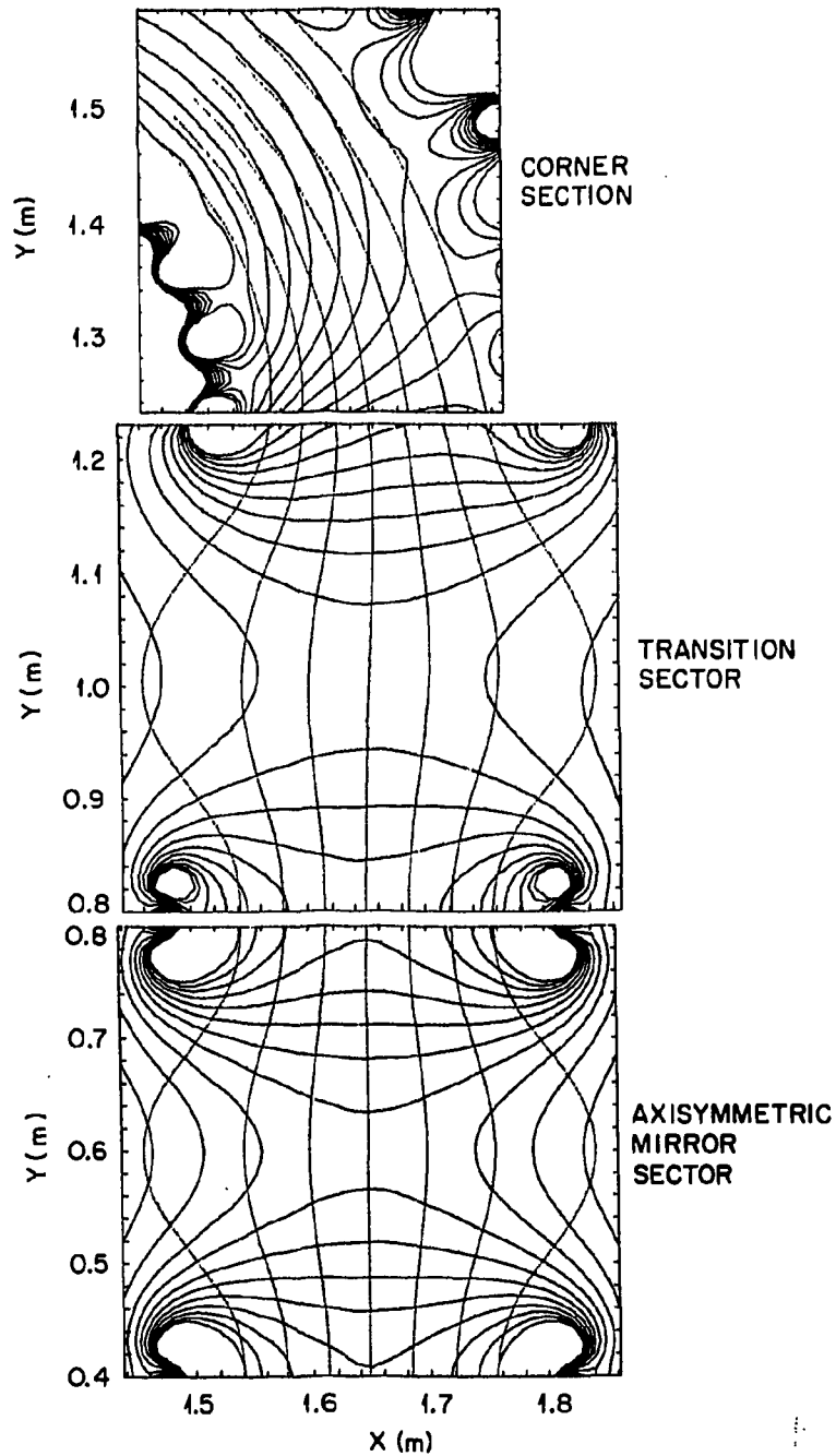
Fig. 1.2. Mod-B contours (solid) and magnetic field lines (dotted) in the equatorial plane of an EBS configuration with circular coils in the corners. Small outward displacement of the corners' (top) symmetrize the mod-B in the transition sector (middle). This allows rings to form on the same flux lines on which they are formed in the axisymmetric sectors (bottom).
