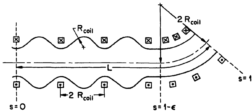
Fig. 7.2. Schematic diagram of a one-eighth sector of an EBS with some typical dimensions.
