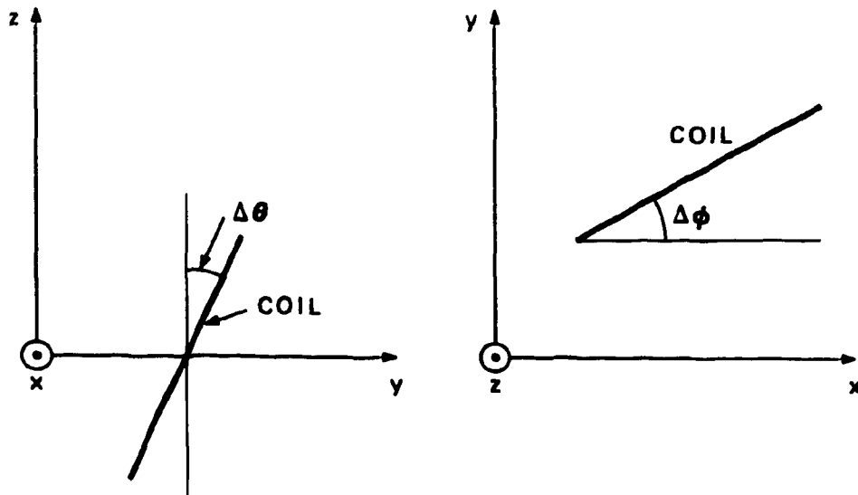
Fig. 3.3. Two angles of the coil plane. Orientation of X , Y , and Z coordinates are shown, with the same orientation as in Figs. 3.1 and 3.2.
