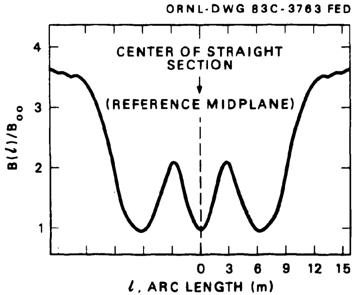
Fig. 9.8. Variation of the magnetic field as a function of arc length along the magnetic axis for one quadrant (straight section plus two half-corners) of an R_T = 20.5 m EBS.
