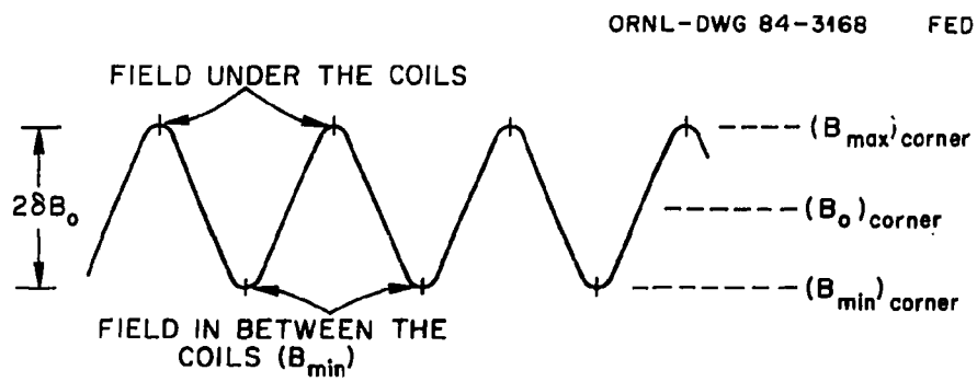
Fig. 2.7. Definitions of field maxima and minima in the corner.
