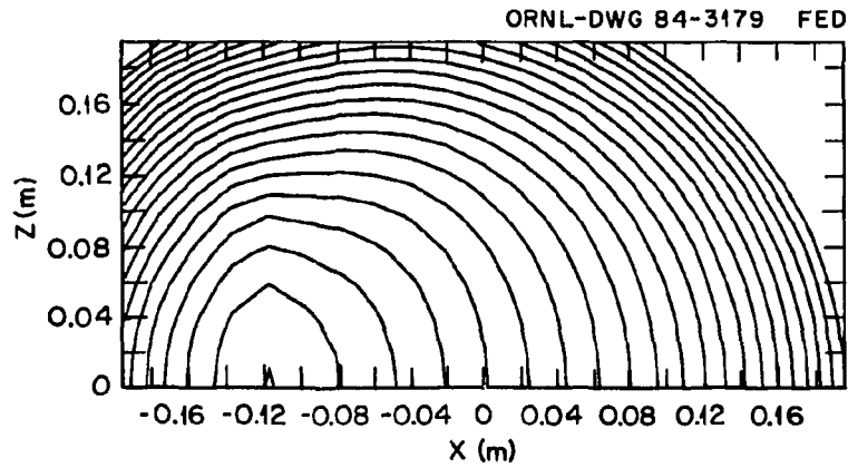
Fig. 4.8. Drift surfaces in a midplane for a high-energy transitional particle in a square configuration. The last closed contour within the volume passes close to the axis of the side. This is in contrast to the circular EBT-I/S configuration, which does not contain any high-energy transitional particles.
