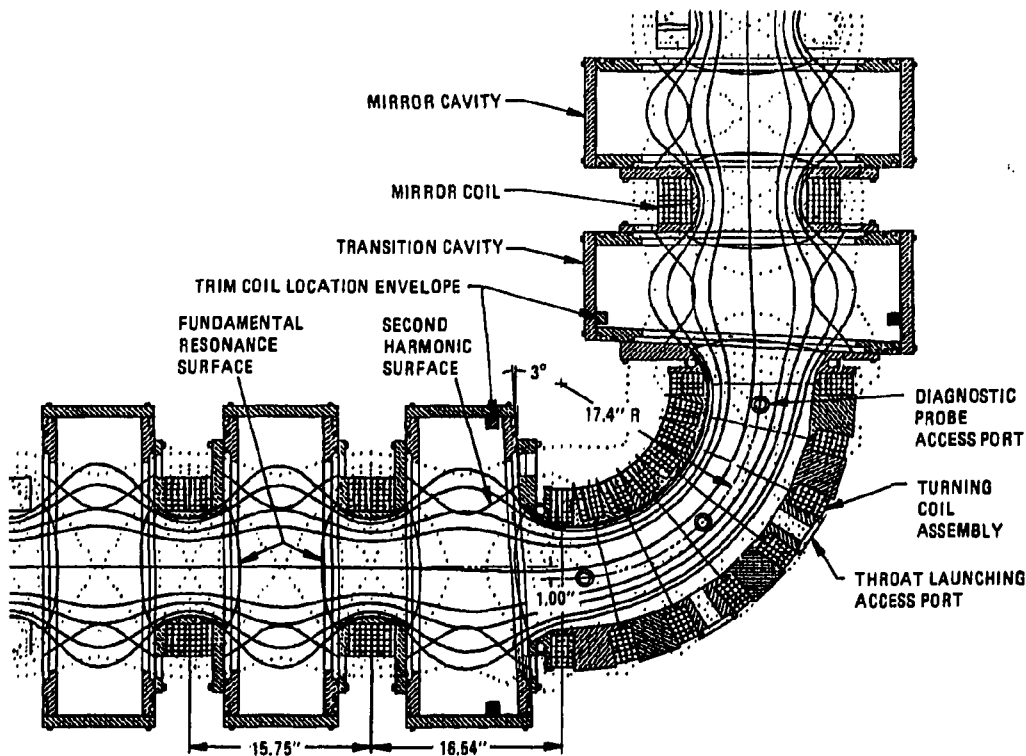
Fig. 18. Relation of microwave cavities and field coils to magnetic field lines.
