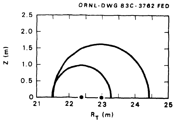
Fig. 9.7. Shape of the trapped (outer curve) and passing (inner curve) particle drift orbits in the "geometric midplane" (only upper half portions are shown).
