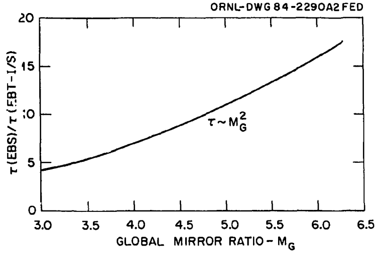
Fig. 7. Variation of confinement time \tau with global mirror ratio M_G = B_{\text{corner}}/B_{\text{mid}} .
