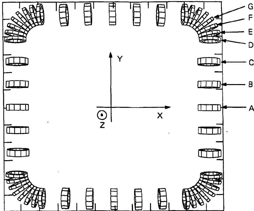
Fig. 3.1. Geometry of an EBS configuration indicating the coil arrangements (top view). Coordinate system used is shown (X and Y axes are indicated; Z-axis points out of the paper — right-hand coordinate system). Specific coils involved in the calculations A through G are indicated, which represent the coils in one field period. In an EBS there are four symmetry planes and eight field periods.
