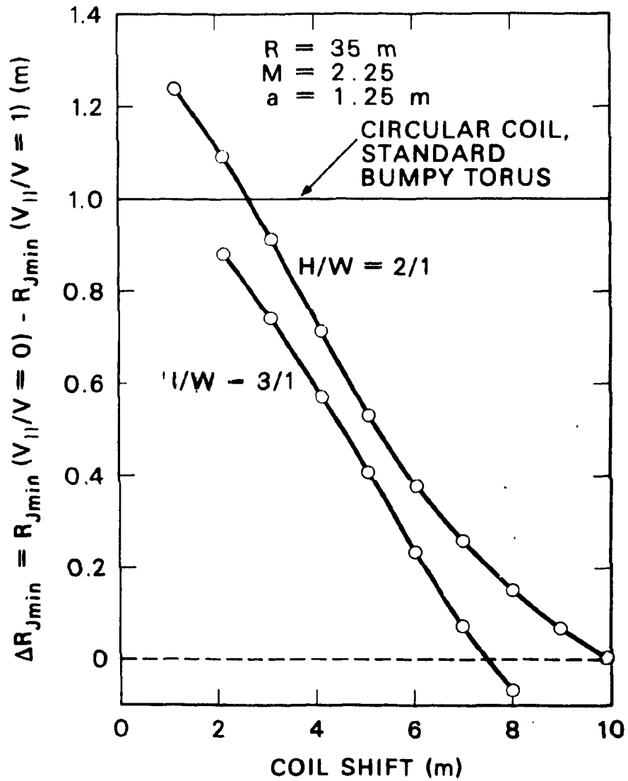
Fig. 9.1. Dispersion in drift orbit centers of trapped and passing particles, \Delta R_{JMIN} , vs coil shift for an R_T = 35 m EBTEC.
