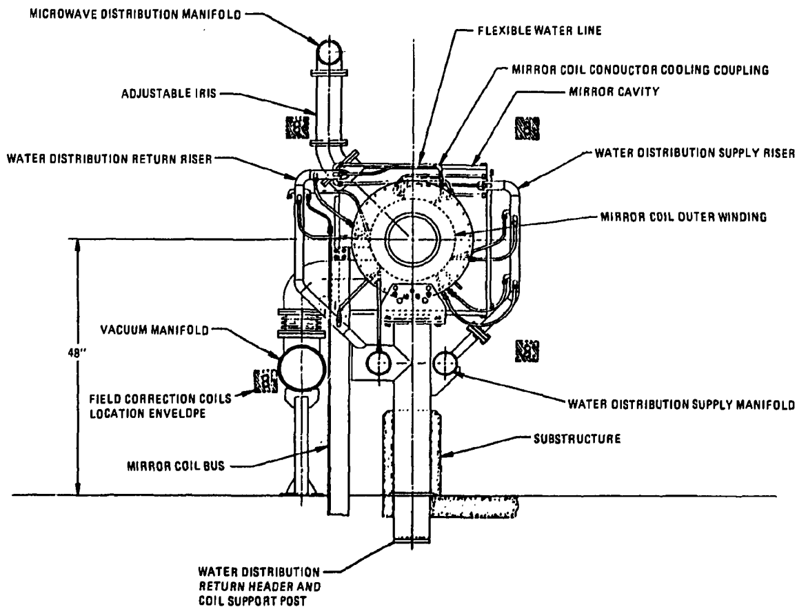
Fig. 17. Cross section of typical elevation of EBS.
