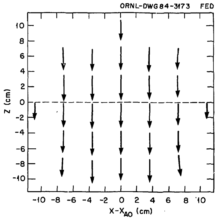
Fig. 3.4. Arrow plot showing the direction and relative magnitude of field line displacements in the plane of A coil for \Delta\theta = 1^\circ . The largest magnitude is 2.82 mm at the coil center (0,0).
