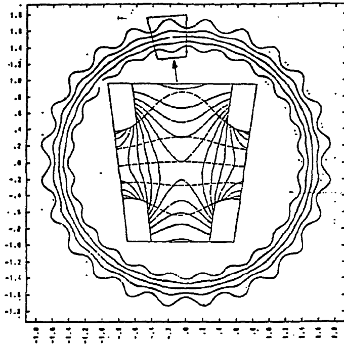
Fig. 1. Field lines in the equatorial plane for (a) EBT and (b) EBS magnetic configurations. The inset drawings show contours of mod-B for an EBT mirror cell and for a central mirror cell of the EBS magnetic configuration. Notice that the mirror cell of an EBS is very nearly axisymmetric and that all toroidal effects are concentrated in the corners.
