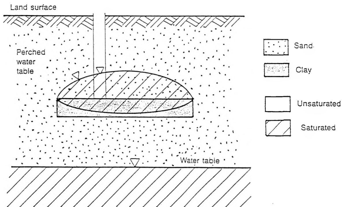
Figure 3. Schematic of perched water table with well (after Freeze and Cherry, 1979).
