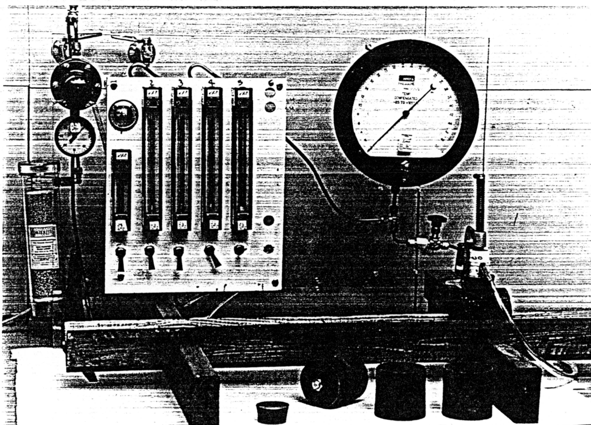
Figure 3. Permeameter used in the laboratory and core measurements. The sample holder here is set up to run core samples.
