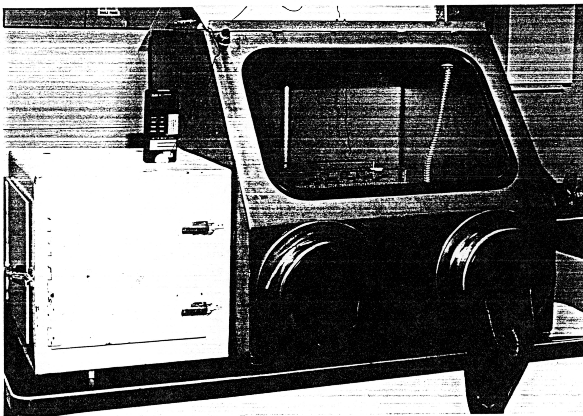
Figure 5. This is the stainless steel glove box used for the equilibrium water saturation experiment. In the window, the top tier of basalt plugs can be seen.
