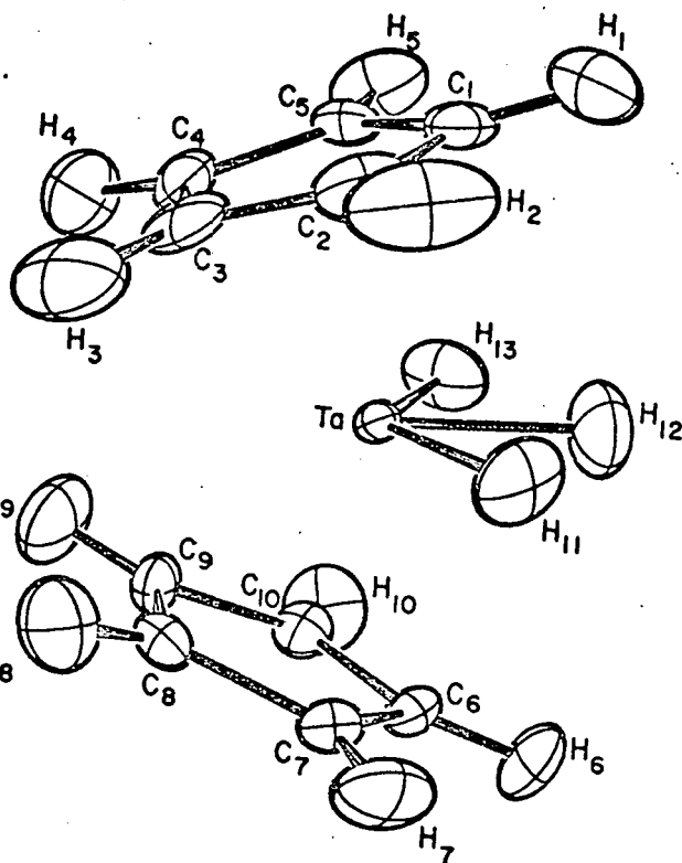
Fig. 5. The structure of \text{H}_3\text{TaCp}_2 .
