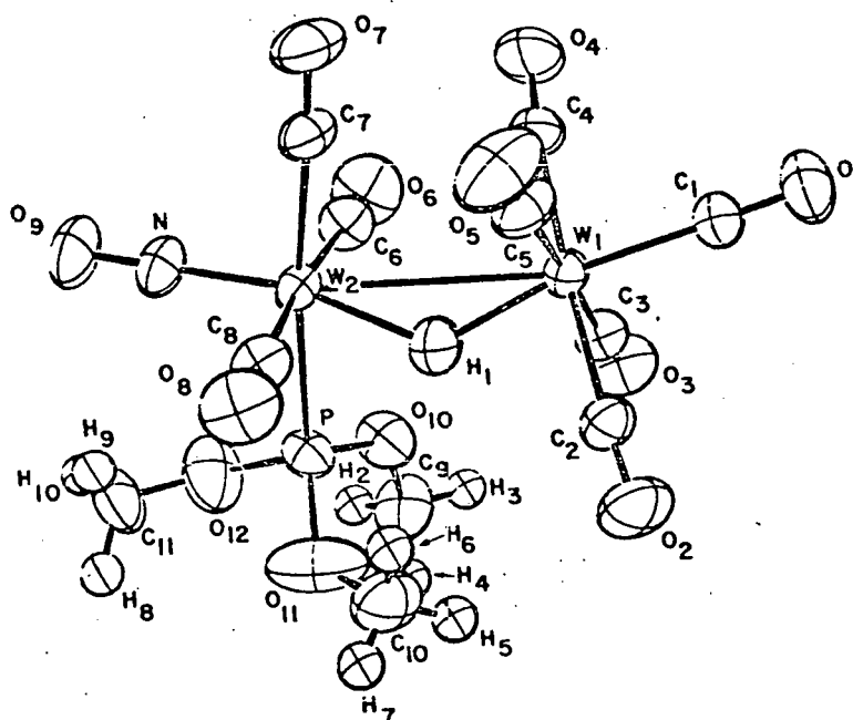
Fig. 7. The structure of \text{HW}_2(\text{CO})_8(\text{NO})(\text{P}(\text{OMe})_3) .
