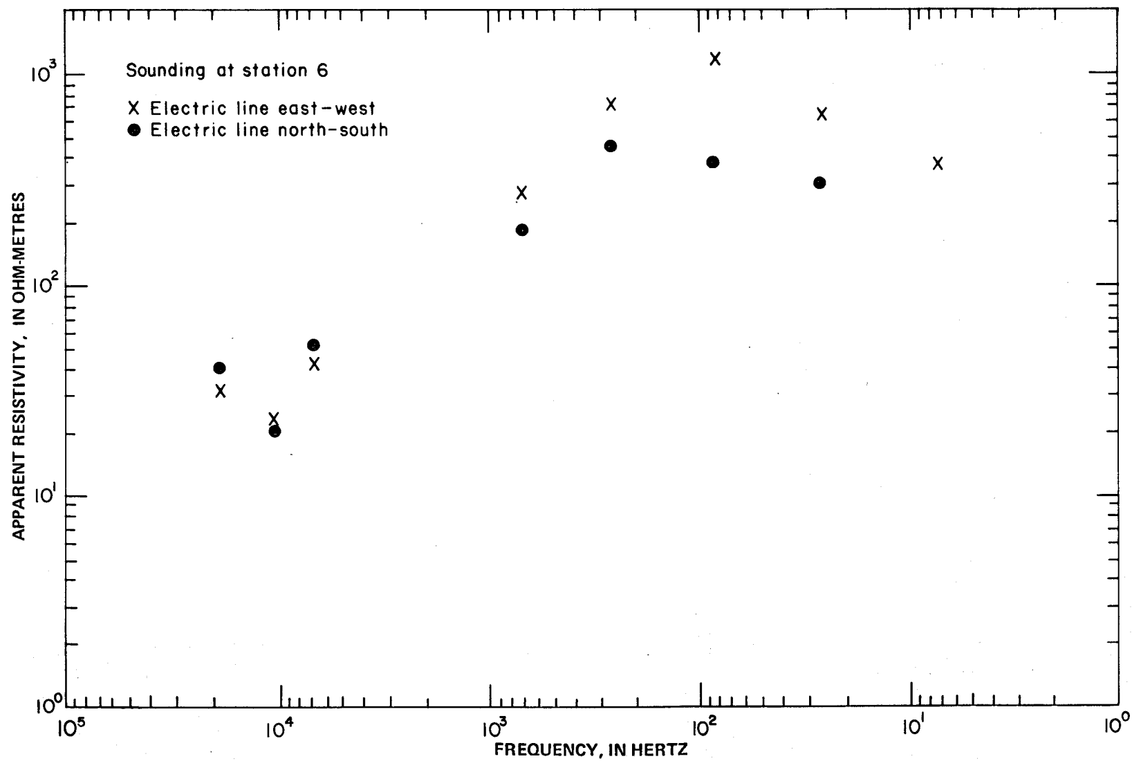
FIGURE 17. Apparent resistivities at station 6.
