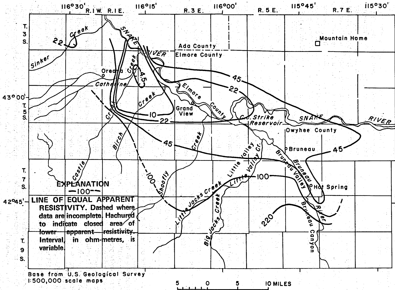
FIGURE 14. Apparent resistivity map at 8 hertz.
