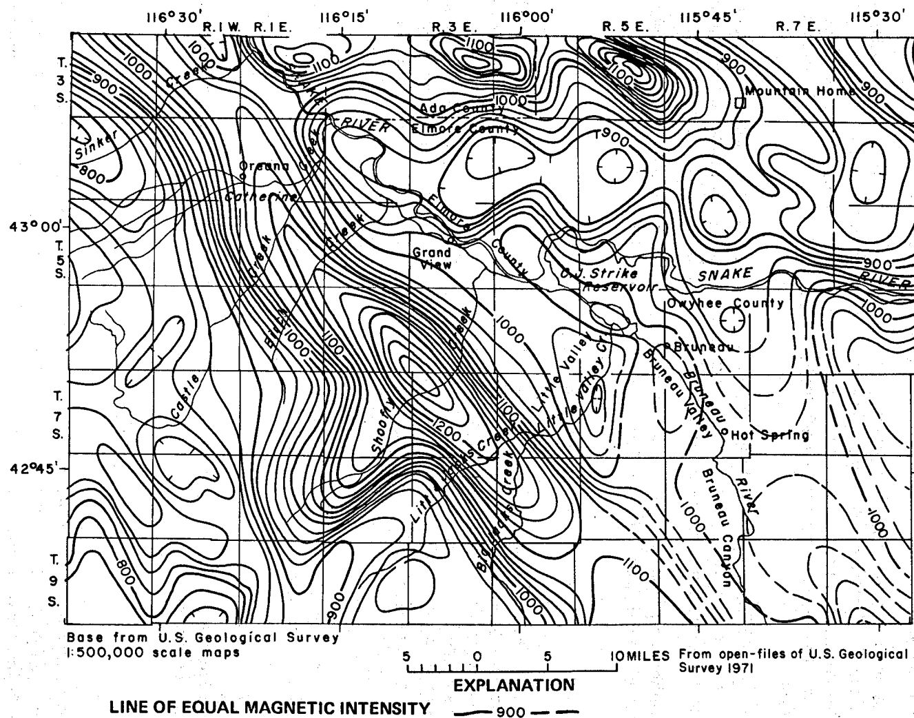
FIGURE 8. Aeromagnetic map.
