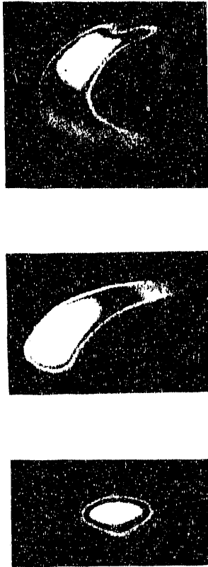
Fig. 9 Profiles (x-y) of a 2 \times 10^{10} e - bunch at 47 GeV with a 0.2 mm oscillation (left), with a 0.5 mm oscillation (center), and with a 1 mm oscillation (right) in both planes. The initial core sizes in both planes are about 120 \mu m.
