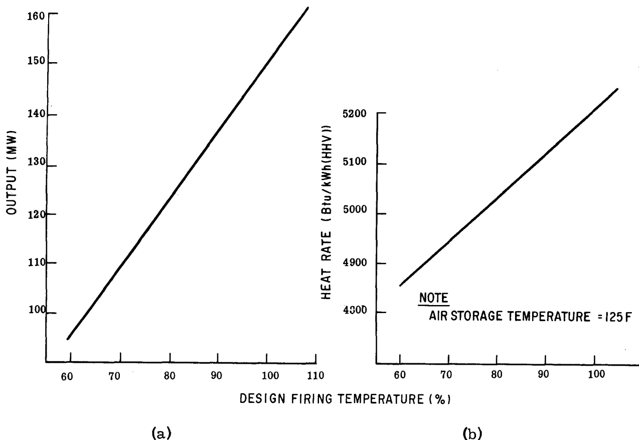
Figure 7-8. Brookville CAES Plant Performance
