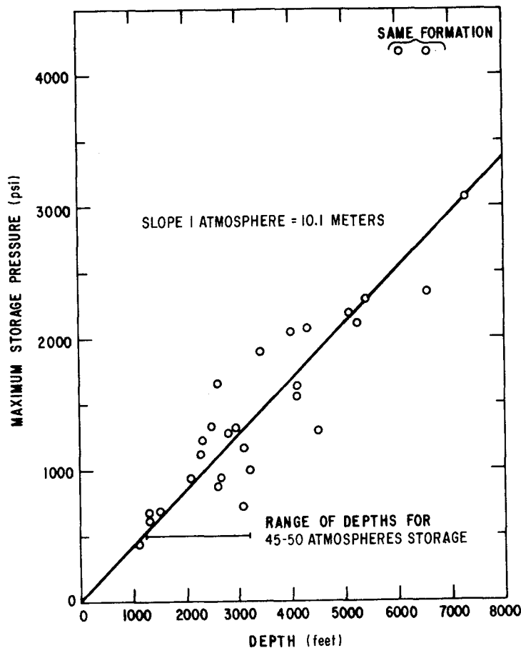
Figure 2-1. Maximum Storage Pressure vs Depth for 33 Giant Gas Storage Reservoirs in the United States (Ref. 31)
