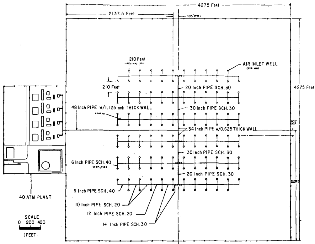
Figure 3-10. 600 MWe, 40 Atmosphere Aquifer Storage Plant
