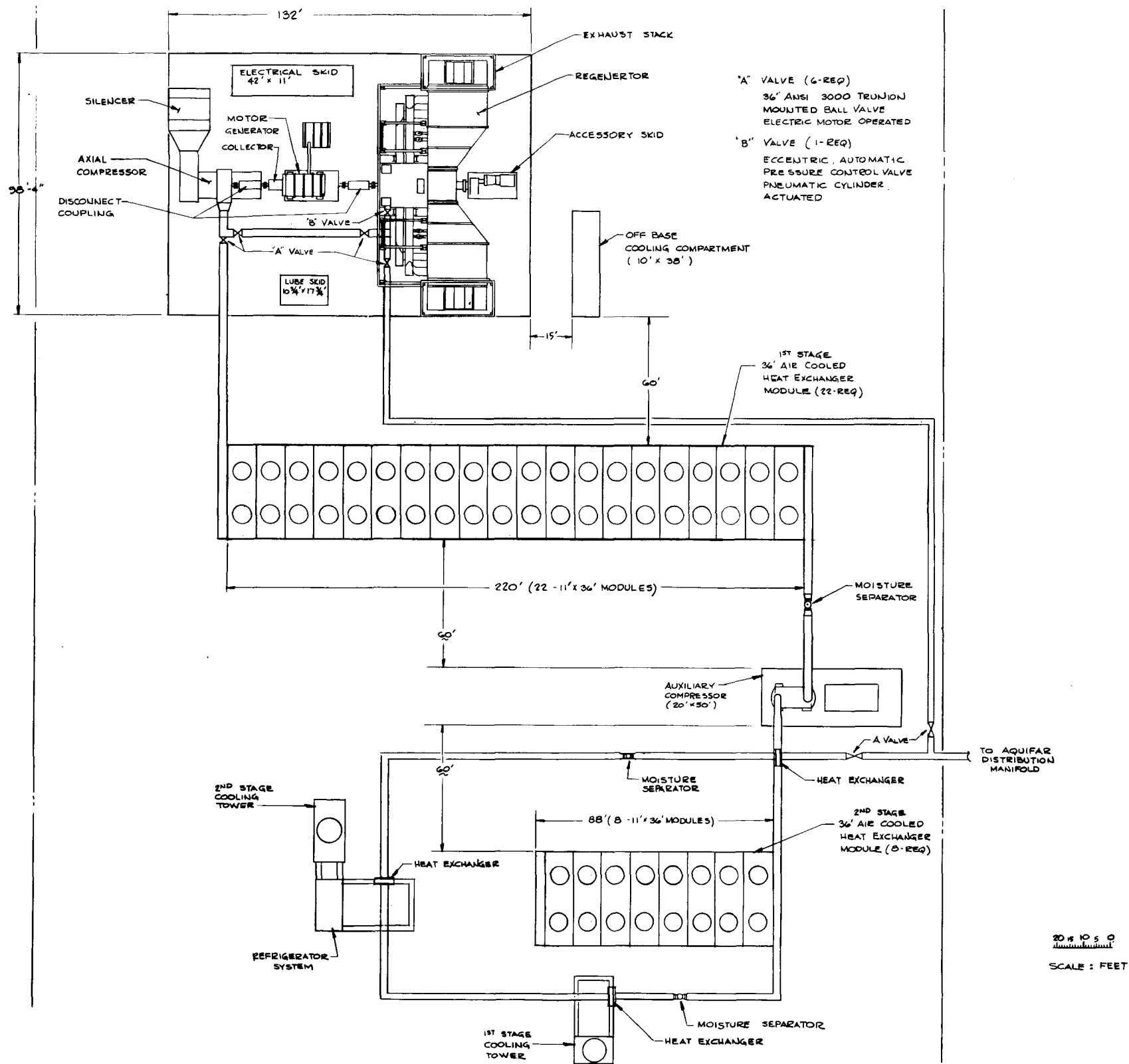
Figure J-1. Equipment Arrangement for Initial Plant
