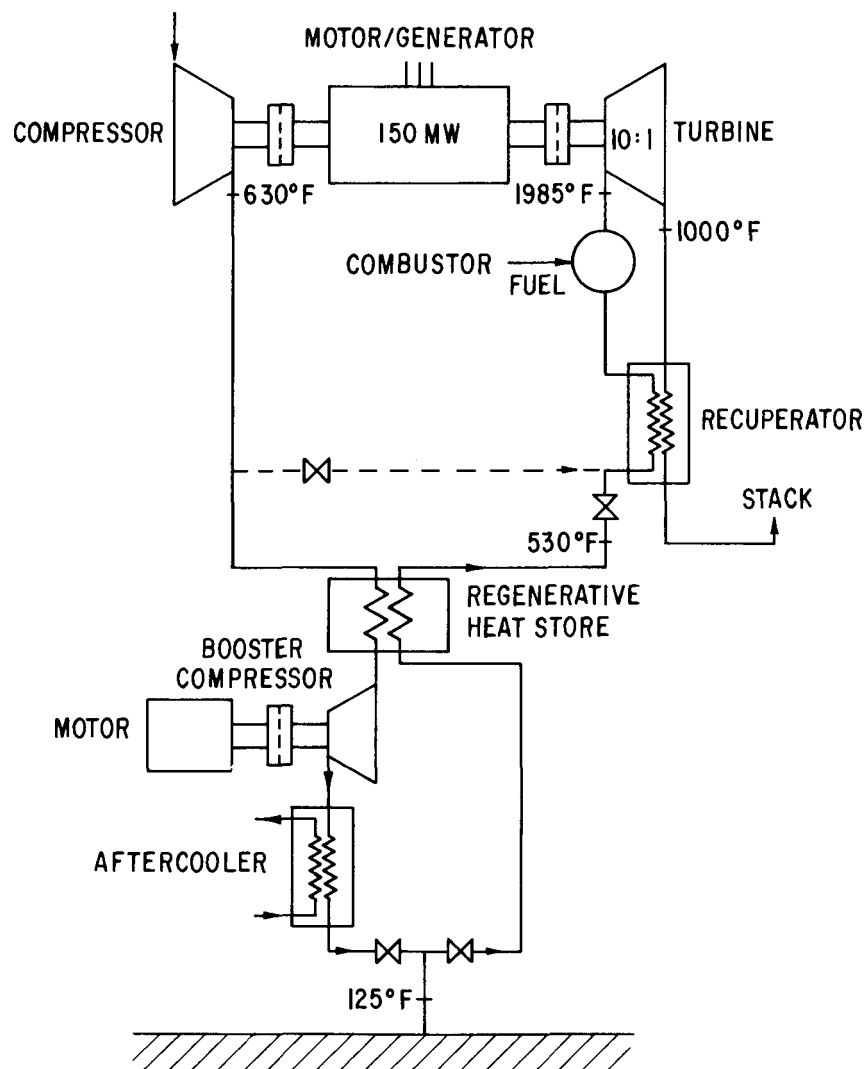
Figure 3-6. Third Generation Base System with Heat Storage
