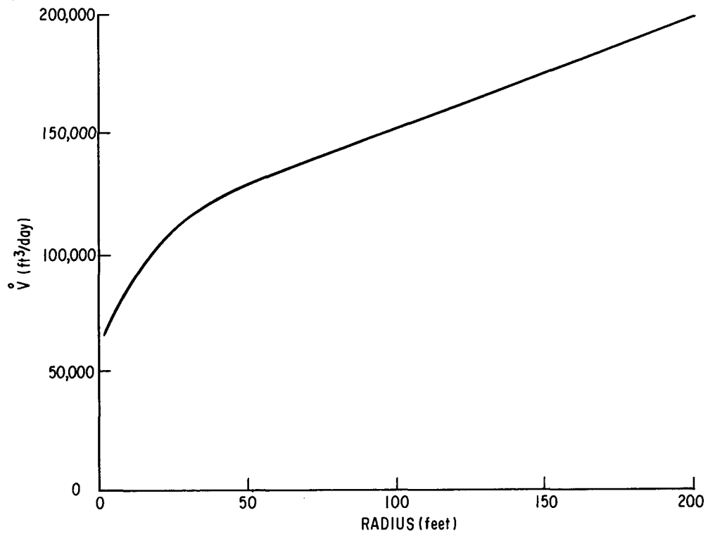
Figure G-1. Volumetric Displacement of Water as a Function of Radius for a Single Well in the Brookville Aquifer for \Delta P = 163 Psia
