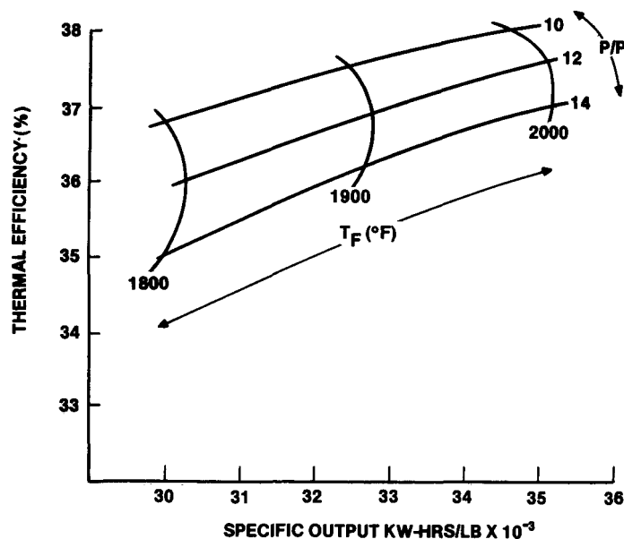
Figure 9-1. Typical Regenerative Cycle Gas Turbine Performance Characteristic
