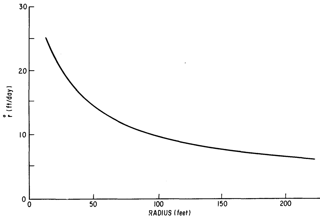
Figure G-2. Radial Rate of Reservoir Growth as a Function of Radius in the Brookville Aquifer for P = 163 Psia
