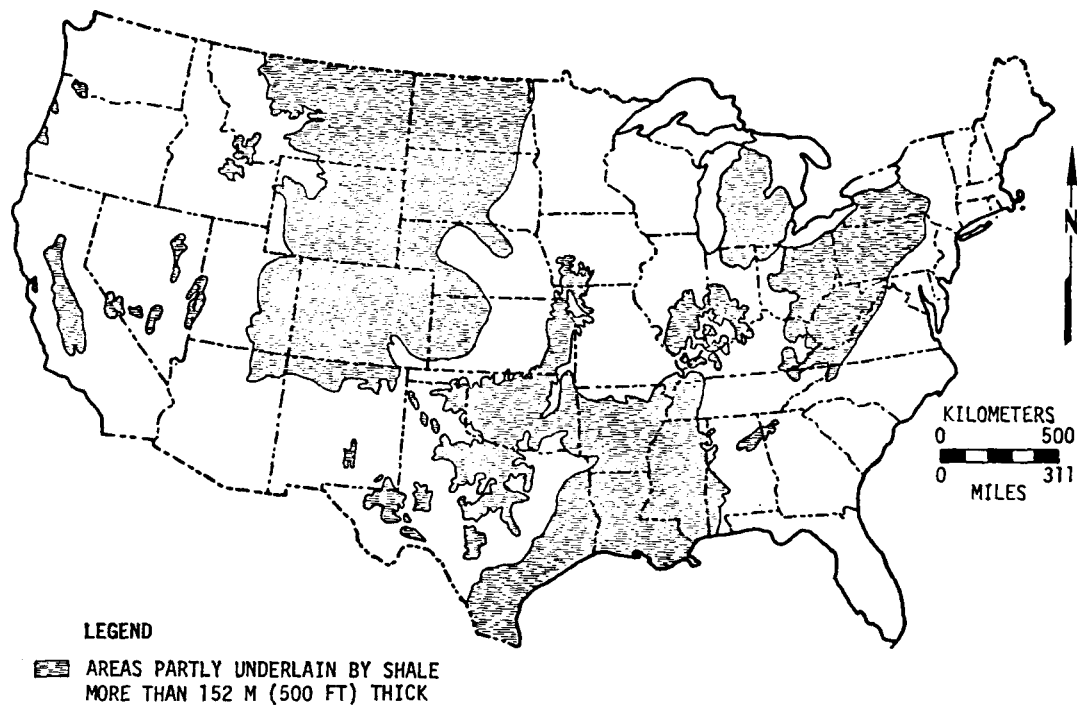
Figure 3-18. Thick Shale Deposits in the United States
