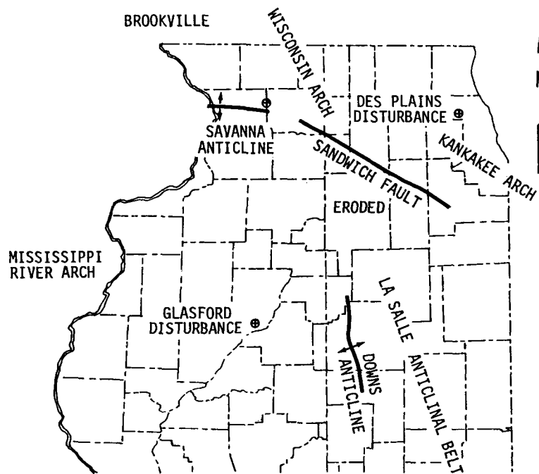
Figure F-1. Structure on Top of Galena Group in Northern Illinois
