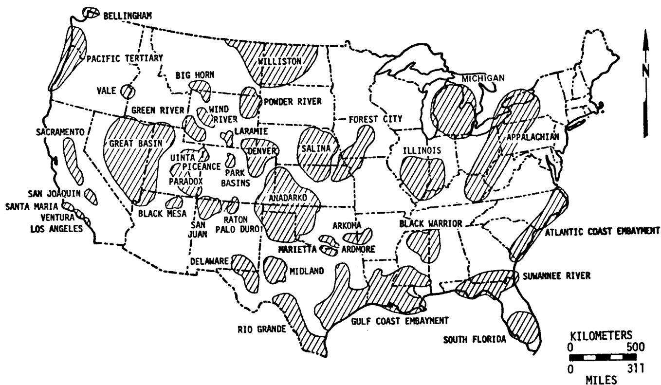
Figure 3-20. Major Depositional Basins in the United States
