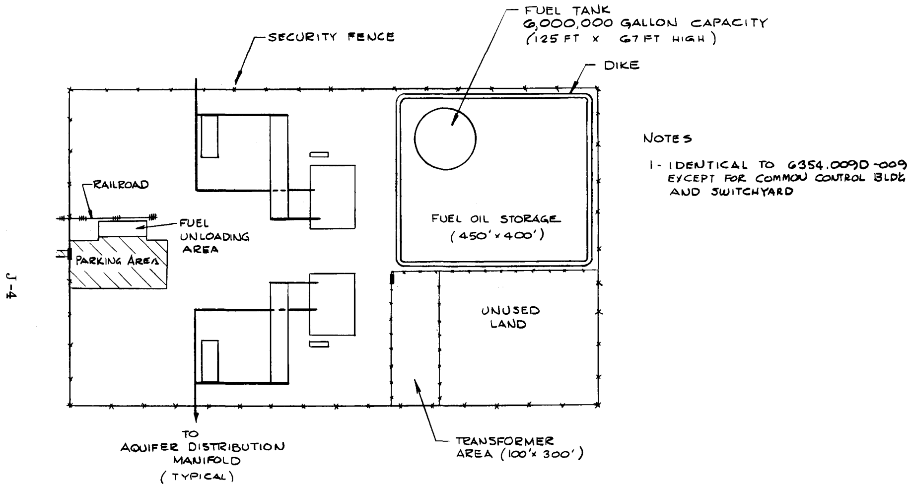
Figure J-3. Partial Plot Plan -- 300 MW e Cluster without Control Building
