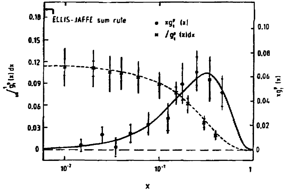
Fig. 1. EMC results for xg_1^p(x) (Ref. 13)
