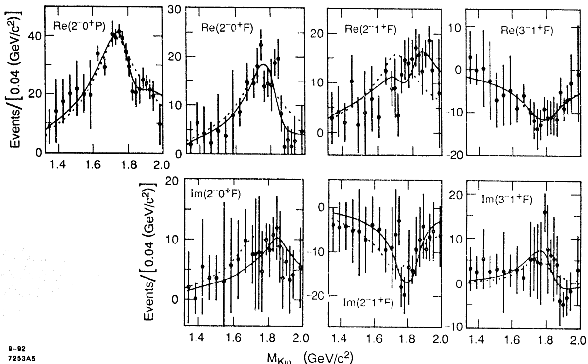
Figure 5. The real and imaginary parts of the K^-\omega 2^- and 3^- amplitudes; the lines show the results of the fits described in the text.
