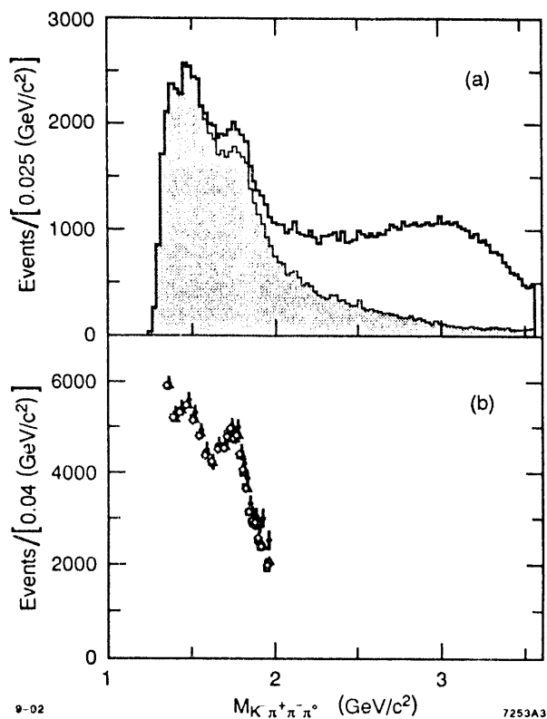
Figure 3. The K - \pi^+\pi^-\pi^0 invariant mass distribution for events with 0.1 < |t'| < 2.0 (GeV/c) 2 ; (a) the unshaded curve contains all events that satisfy 0.72 < M_{3\pi} < 0.84 GeV/c 2 while the shaded portion contains events with M_{p\omega} > 2.28 and M_{pK} > 2.0 GeV/c 2 ; (b) the background-subtracted and acceptance-corrected mass distribution; the points with error bars are the measured values and the other points are the values obtained in the PWA fit discussed in the text.
