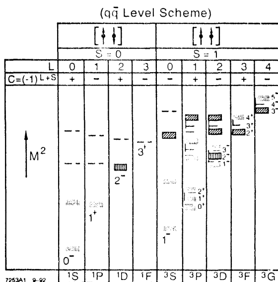
Figure 1. Level diagram (Grotrian plot) for the strange meson states known before this analysis. All of these states have been observed in the LASS/SLAC group B program. The dashed lines indicate the lowest lying states expected in the quark model. The mass levels are illustrative only. The states indicated by cross-hatching are clearly observed, and have generally been confirmed; in a few cases there are possible classification ambiguities. Only one strange 2^- meson has been confirmed. It could be either the S=0 or the S=1 state, or perhaps a mixture, as shown by the vertically lined boxes. The states indicated by diagonal lines are more speculative and require confirmation.
