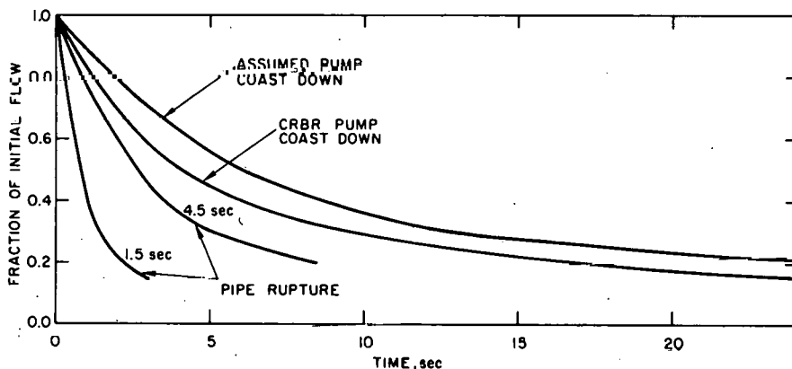
Fig. 8. Flow Reduction Rates for Pump Coastdown and for Less Extreme Pipe Rupture Cases. ANL Neg. No. 11b-76-20.
