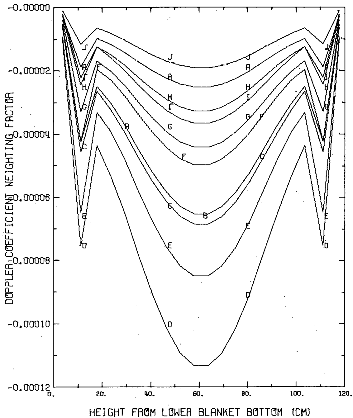
Fig. 7. Doppler Worth Distribution for CRBR, BOL State. ANL Neg. No. 116-76-16.
