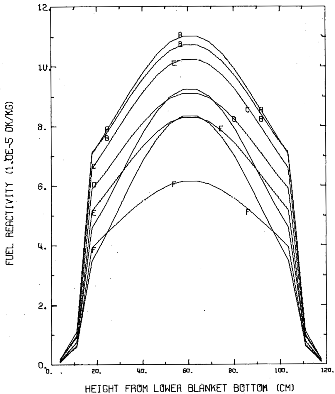
Fig. 4. Fuel Worth for CRBR, BOL State. ANL Neg. No. 116-76-11.
