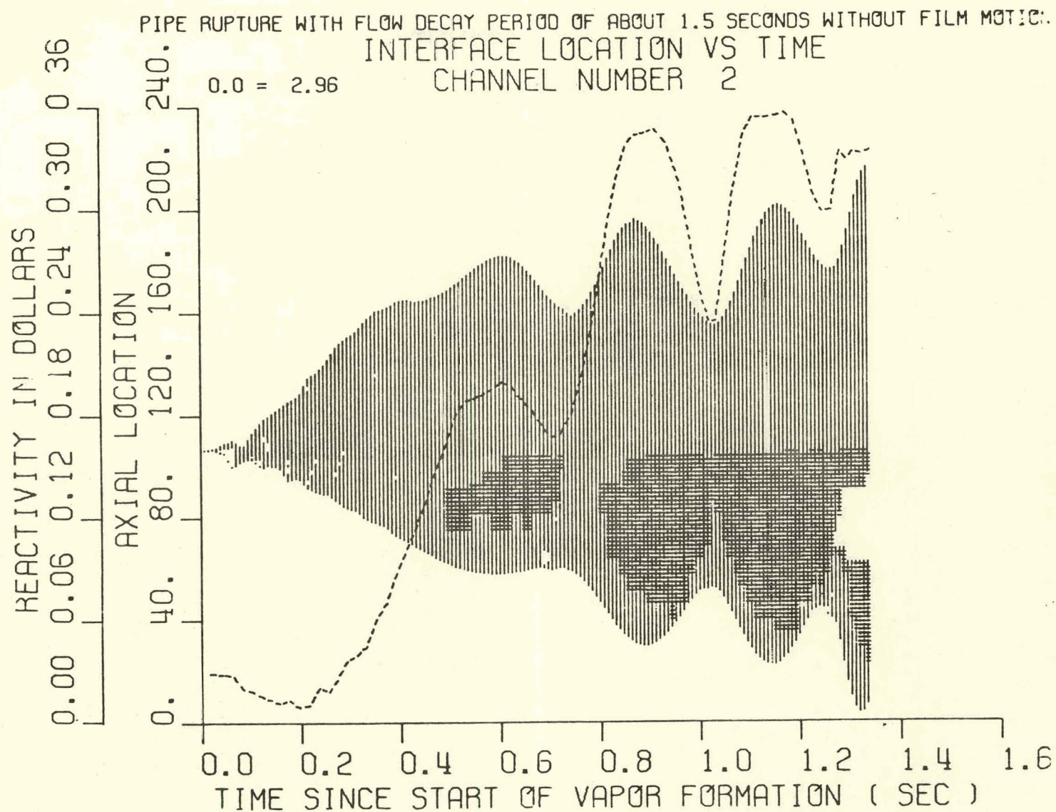
Fig. 11. Sodium Liquid-vapor Interface Location for 1.5 sec Pipe Rupture Accident, Static Film, 1-phase Friction Factor. ANL Neg. No. 116-76-13.
