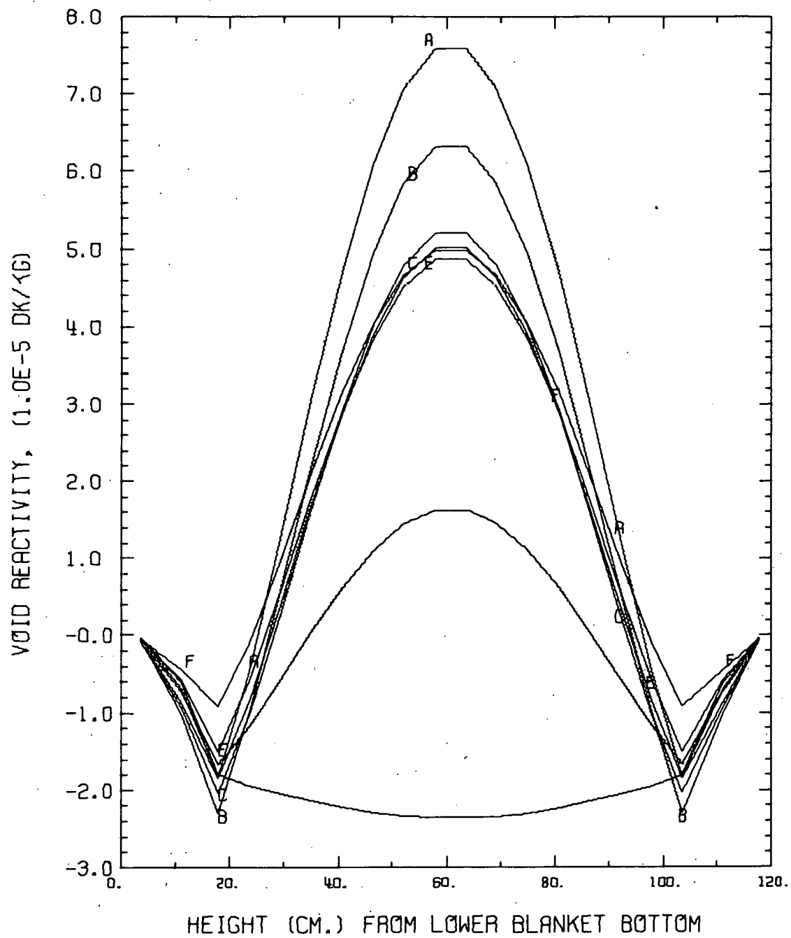
Fig. 5. Sodium Void Worth for CRBR, BOL State. ANL Neg. No. 116-76-12
