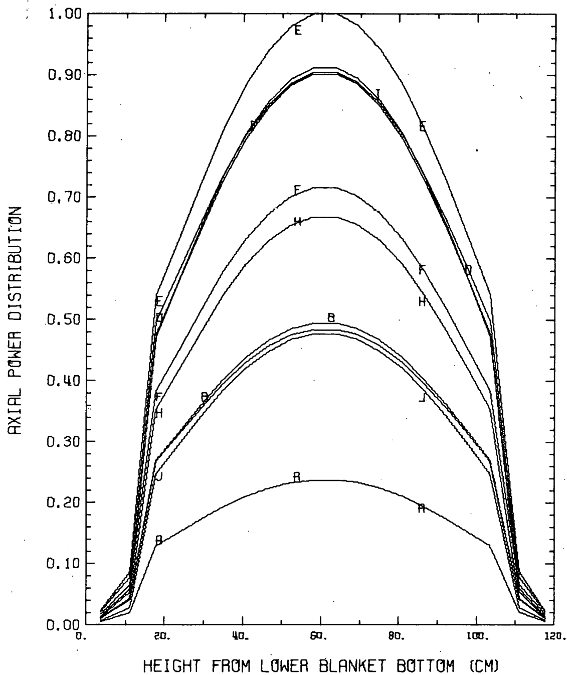
Fig. 3. Axial Power Distribution for CRBR, BOL State. Letters A, B, C, etc. refer to Channels 1, 2, 3, etc. respectively. ANL Neg. No. 116-76-18.
