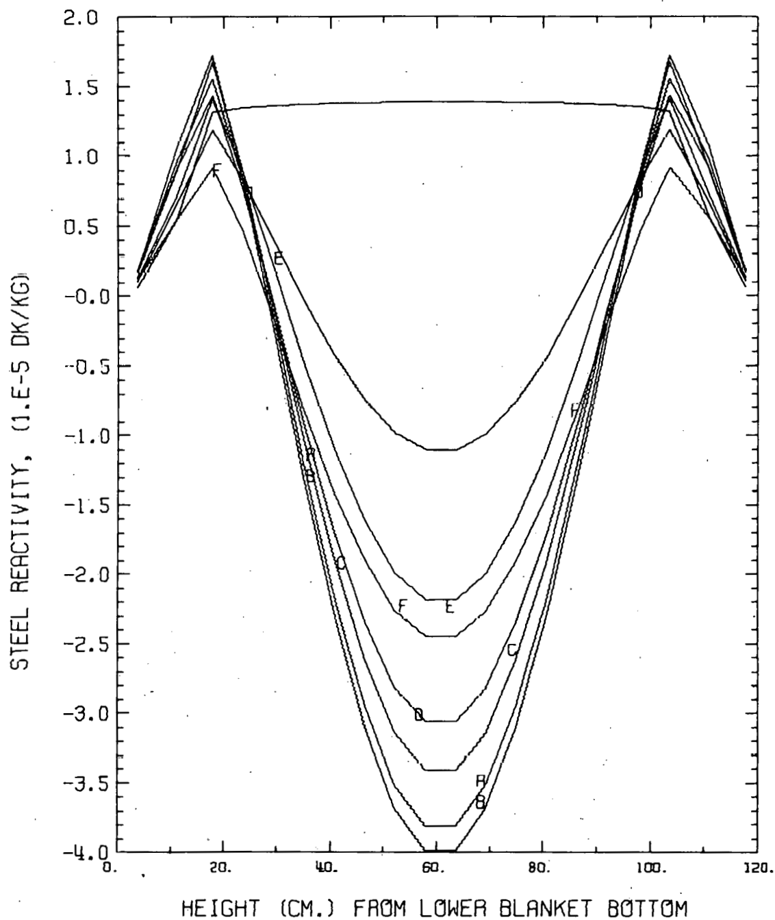
Fig. 6. Clad Worth for CRBR, BOL State. ANL Neg. No. 116-76-14.
