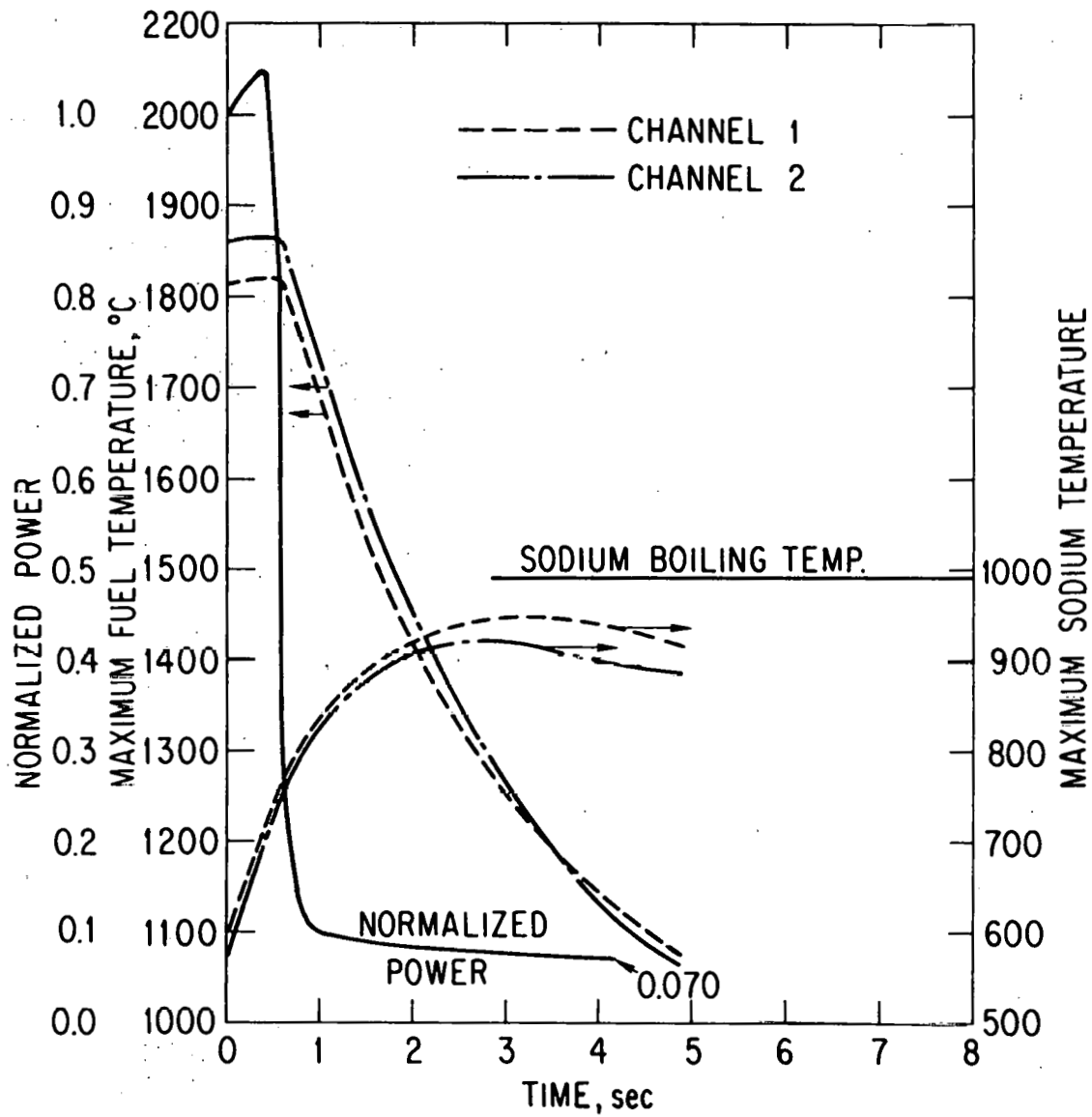
Fig. 13. Results for Extreme Pipe Rupture Accident with Scram, \Delta P = 0.02 . ANL Neg. No. 116-76-8.
