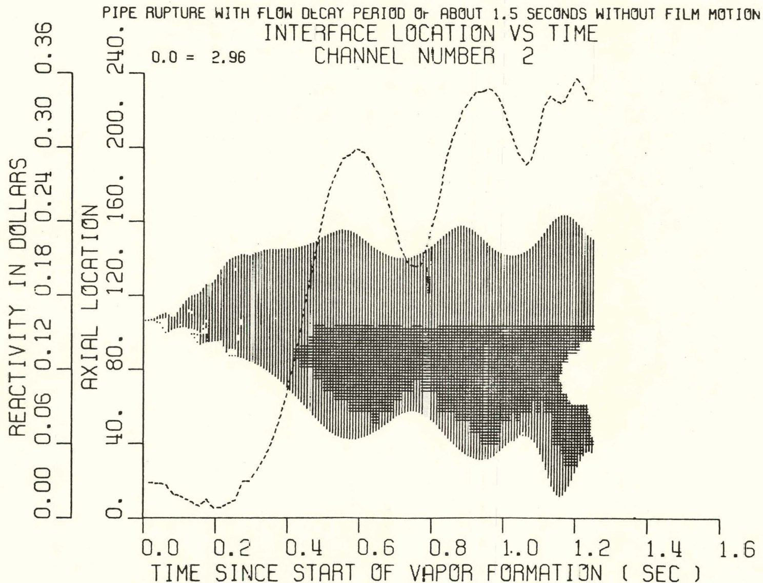
Fig. 10. Sodium Liquid-vapor Interface Location for 1.5 sec Pipe Rupture Accident, Static Film, 2-phase Friction Factor. ANL Neg. No. 116-76-15.
