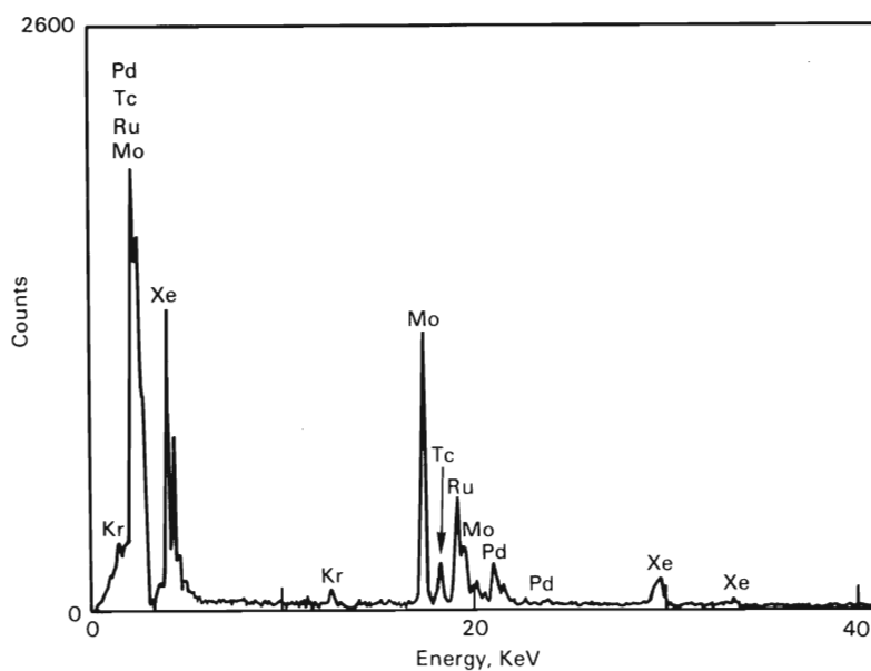
b. EDS Spectrum of Xenon-containing Particle With \text{UO}_2 Matrix Contribution Removed
