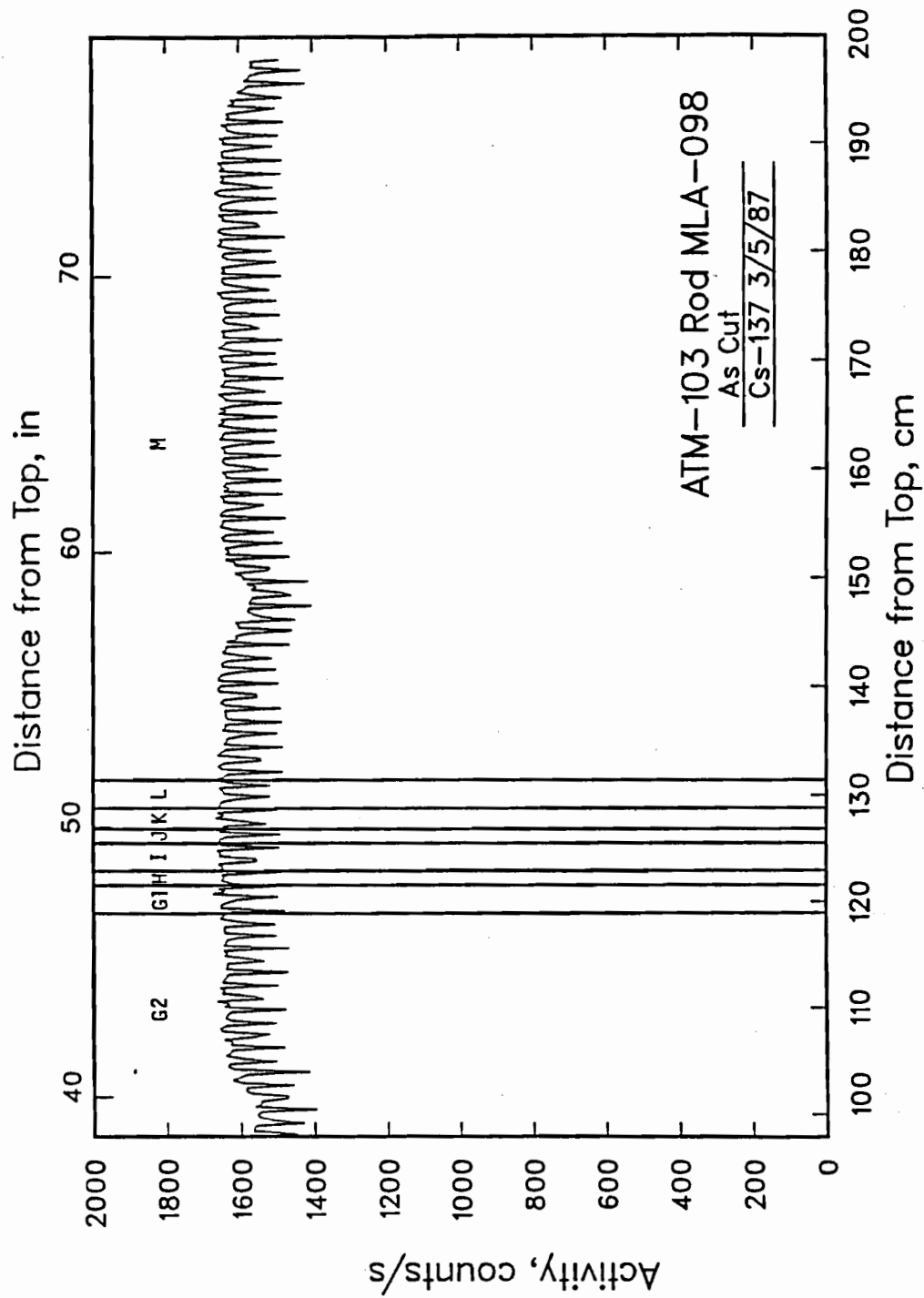
FIGURE D.1.1. As-Cut Sectioning Diagram for Rod MLA098 (contd)
