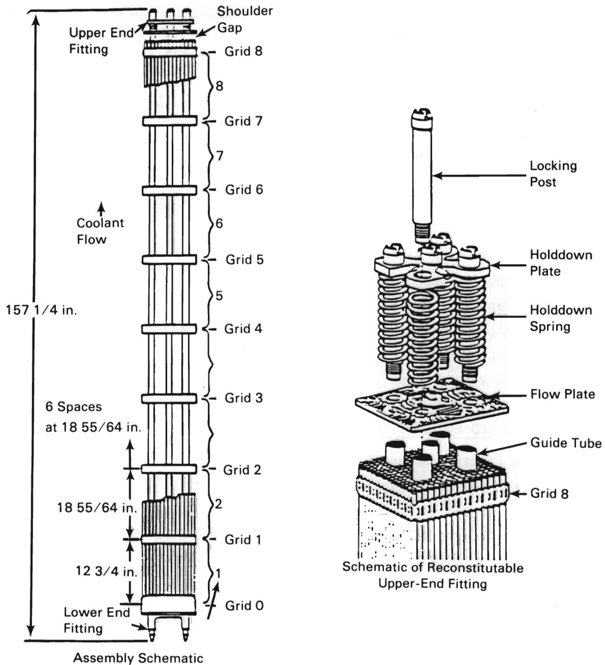
FIGURE 4.1. Fuel Assembly Schematic
