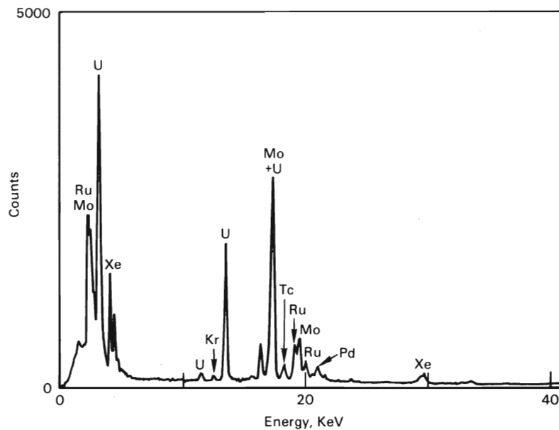
a. EDS Spectrum of Xenon-containing Particle Plus Surrounding \text{UO}_2 Matrix
