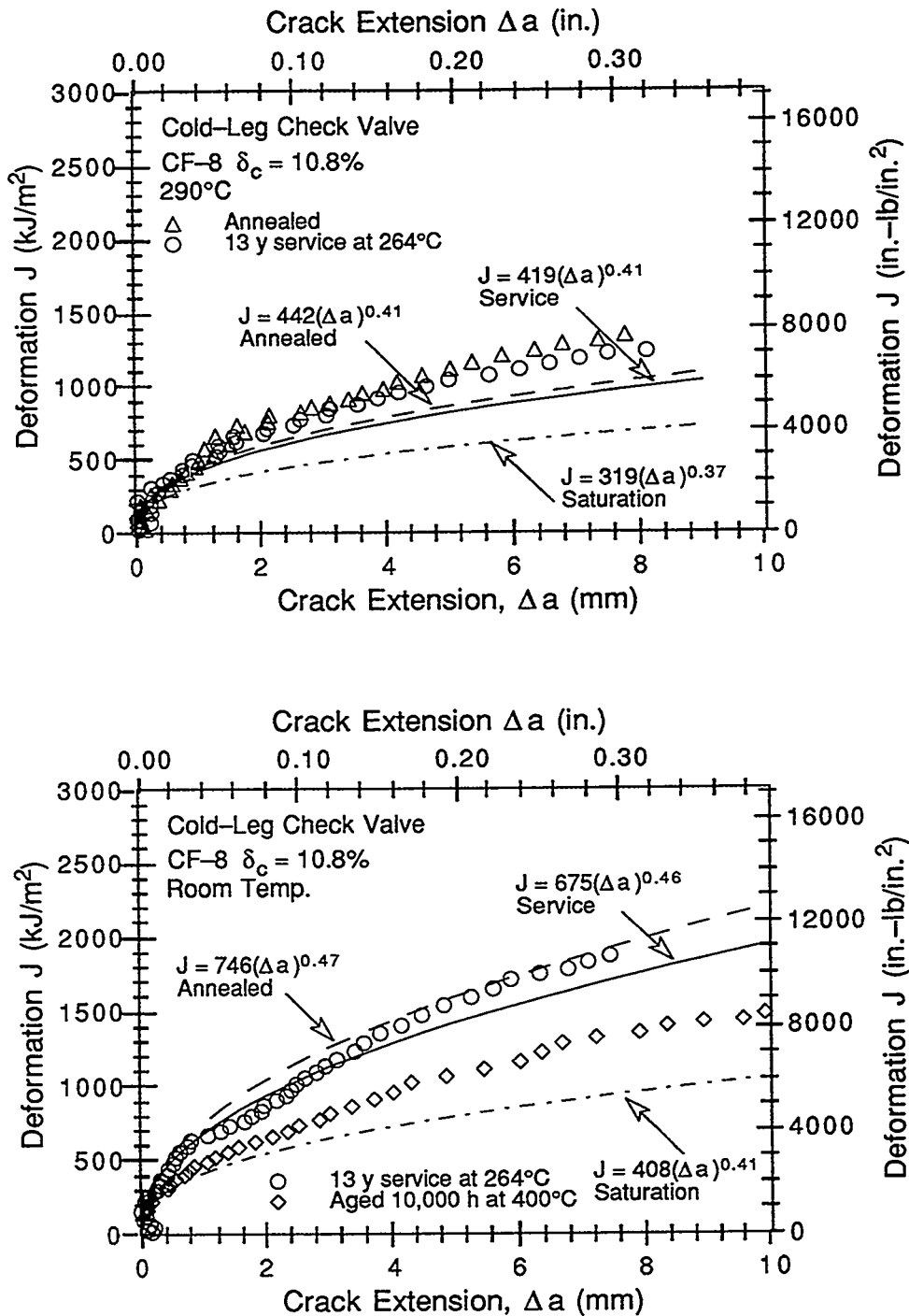
Figure 25. Estimated and measured fracture toughness J - R curves for the cold-leg check valve in the annealed, 13-y service at 264°C, and fully embrittled or saturation condition. (Dashed, solid, and chain-dot lines are the best-fit power-law J - R curves for annealed, service-aged, and laboratory-aged materials, respectively.)
