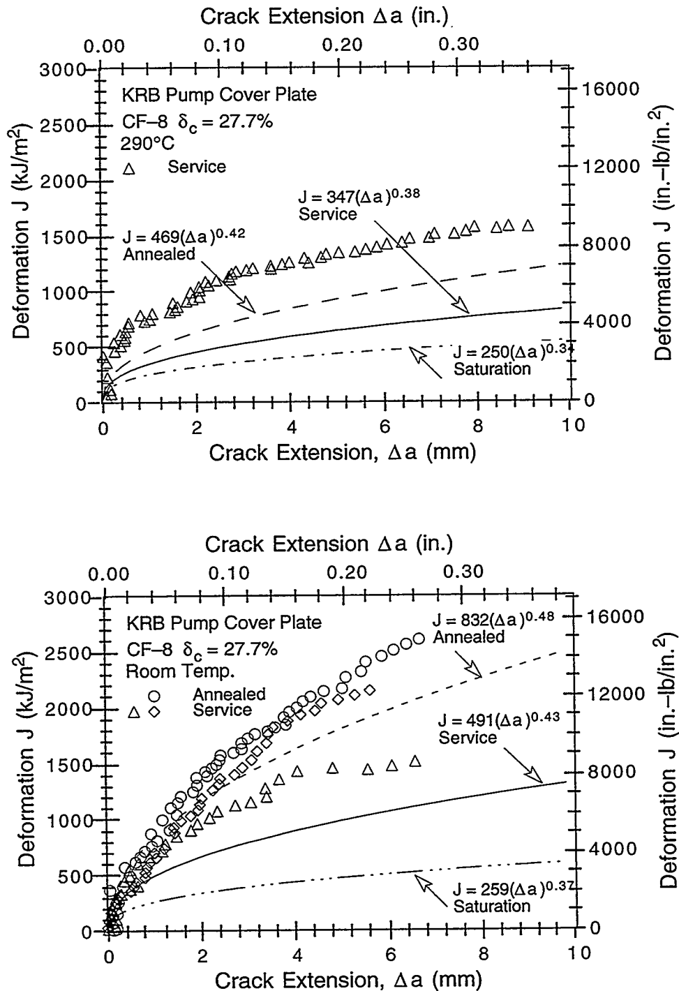
Figure 38. Estimated and measured fracture toughness J-R curve for the KRB pump cover plate in the annealed or unaged condition, after service, and at saturation. (Dashed, solid, and chain-dot lines are the estimated power-law J-R curves for annealed, service-aged, and fully embrittled or aged material, respectively.)
