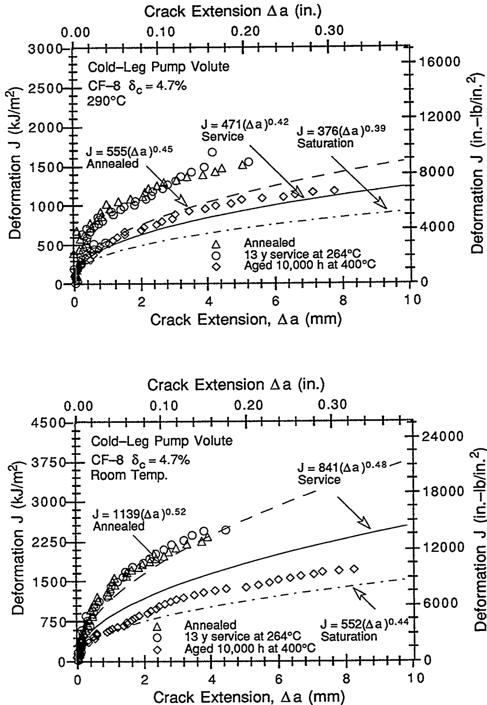
Figure 27. Estimated and measured fracture toughness J - R curves for the cold-leg pump volute in the annealed, 13-y service at 264°C, and fully embrittled or saturation condition. (Dashed, solid, and chain-dot lines are the best-fit power-law J - R curves for annealed, service-aged, and laboratory-aged materials, respectively.)
