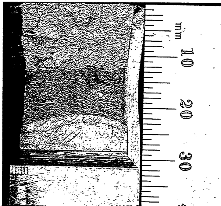
Figure C-11. Fracture surface of the cold-leg check valve CA4 tested at 290°C after 13 y of service at 264°C
