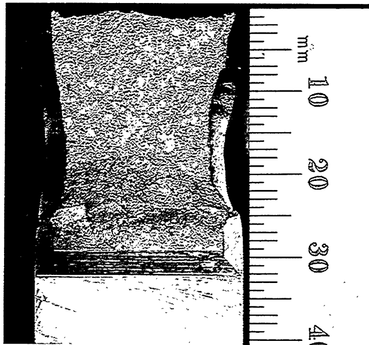
Figure C-26. Fracture surface of essentially unaged material MA9 from the hot-leg main shutoff valve tested at 290°C
