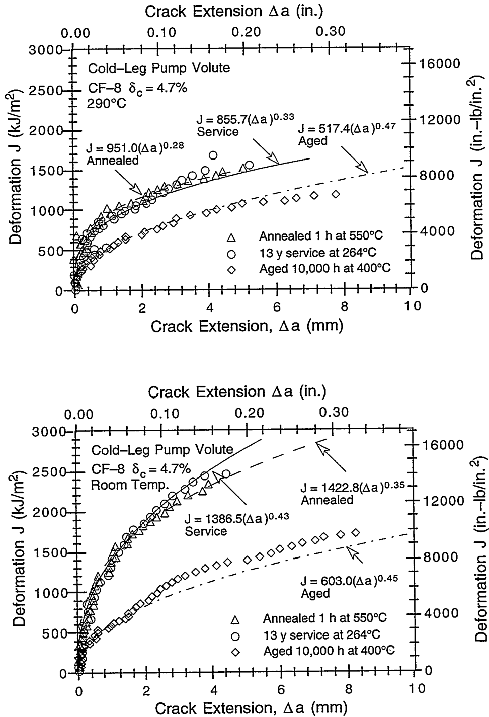
Figure 19. Fracture toughness J-R curves at room temperature and 290°C for annealed, service-aged, and laboratory-aged material from the cold-leg pump volute. (Dashed, solid, and chain-dot lines are the best-fit power-law J-R curves for the annealed, service-aged, and laboratory-aged materials, respectively.)
