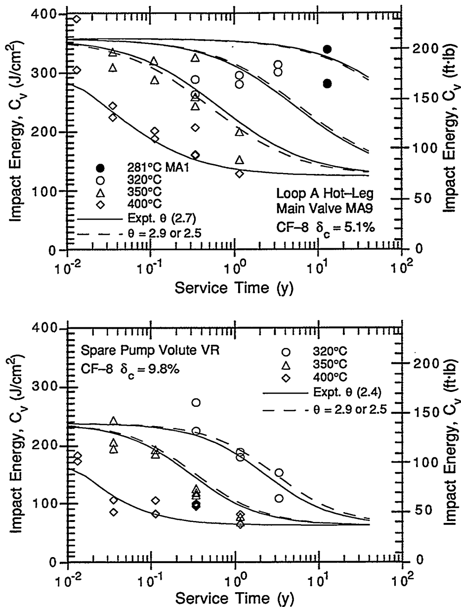
Figure 23. Variations of estimated room-temperature Charpy-impact energy with time for materials from cooler region of the hot-leg main valve MA9 and spare pump volute VR.
