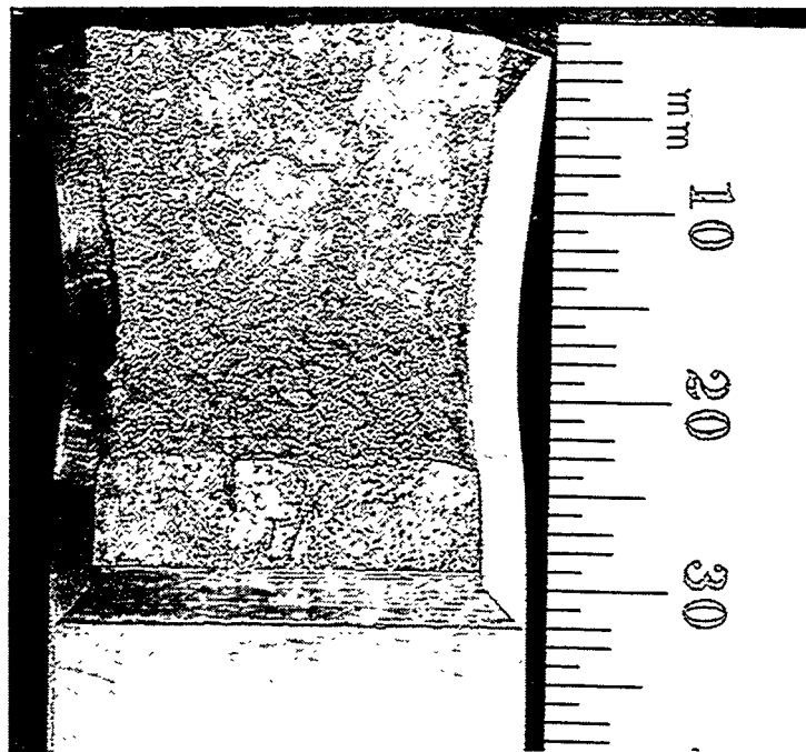
Figure C-50. Fracture surface of the unaged spare pump volute VR tested at room temperature
