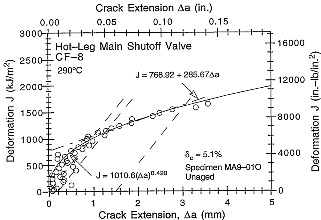
Figure C-27. Deformation J-R Curve at 290°C for essentially unaged material MA9 from the hot-leg main shutoff valve
