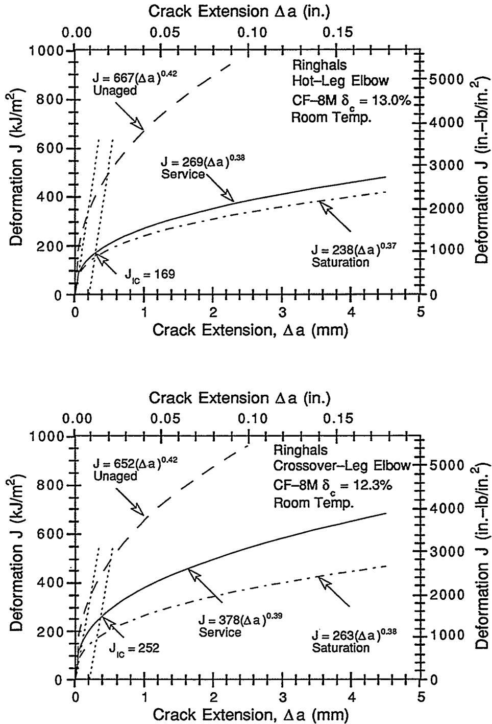
Figure 35. Estimated fracture toughness J - R curves for the Ringhals hot- and crossover-leg elbows in the unaged condition, after service, and at saturation. (Dashed, solid, and chain-dot lines are the estimated power-law J - R curves for unaged, service-aged, and fully embrittled or aged material, respectively.)
