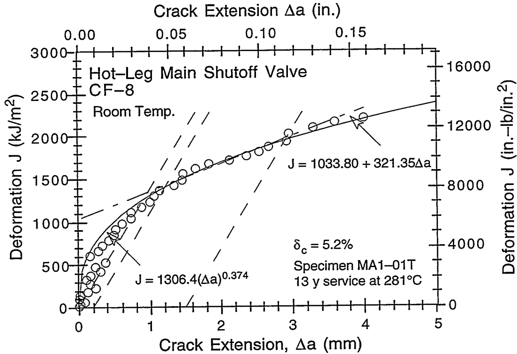
Figure C-15. Deformation J-R Curve at room temperature for hot-leg main shutoff valve MA1 after 13 y of service at 281°C
