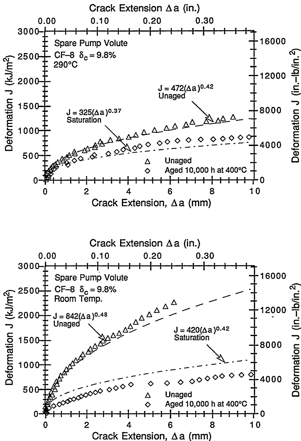
Figure 28. Estimated and measured fracture toughness J - R curves for the spare pump volute in the unaged and fully embrittled or saturation condition. (Dashed and chain-dot lines are the best-fit power-law J - R curves for unaged and laboratory-aged materials, respectively.)
