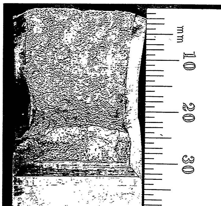
Figure C-32. Fracture surface of recovery-annealed material from the pump volute PV tested at room temperature
