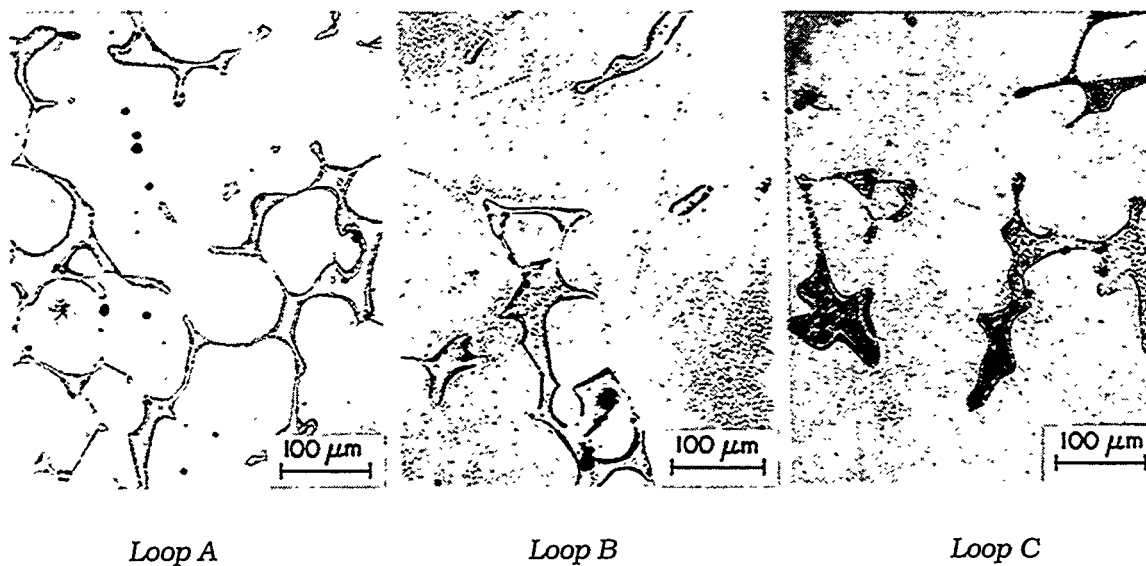
Figure 5. Ferrite morphology of cast materials from Loops A, B, and C cold-leg check valves from the Shippingport reactor
