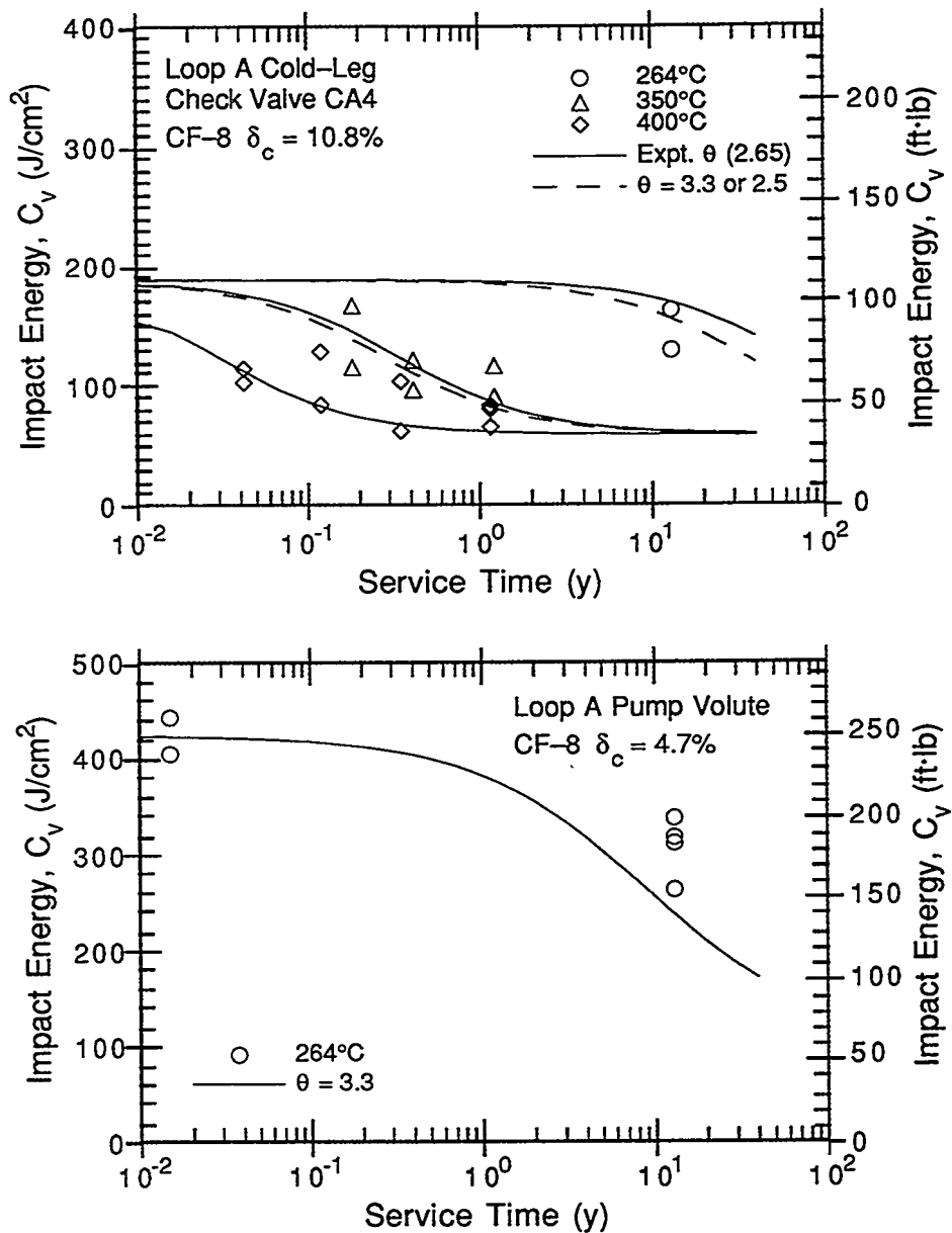
Figure 22. Variations of estimated room-temperature Charpy-impact energy with service time for Loop A cold-leg check valve CA4 and pump volute PV
