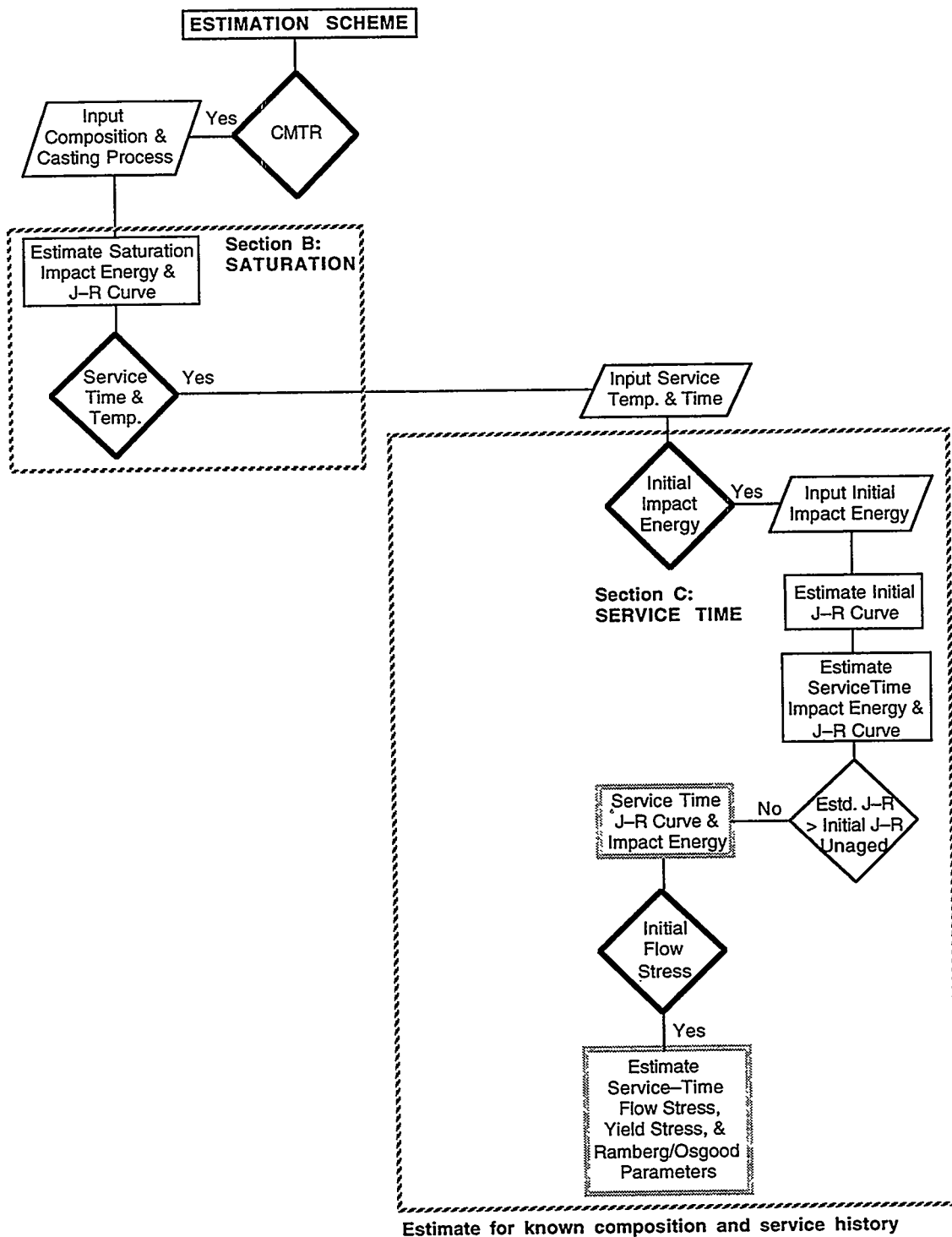
Figure 21. Flow diagram for estimating mechanical properties of cast materials obtained from the Shippingport reactor
