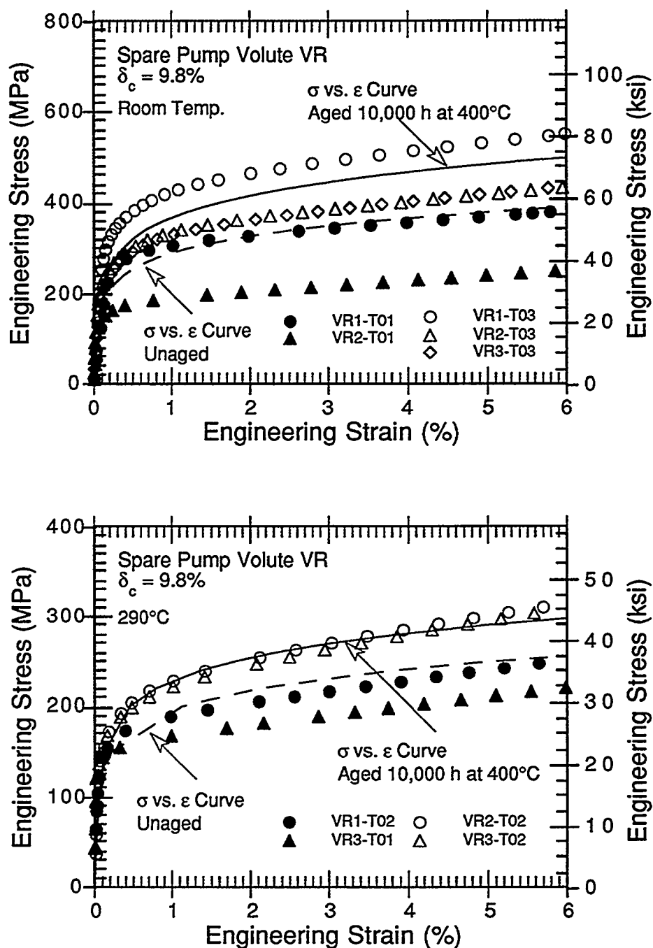
Figure 33. Estimated and measured tensile stress-vs.-strain curves at room temperature and 290°C for the spare pump volute in the unaged and fully embrittled or aged condition
