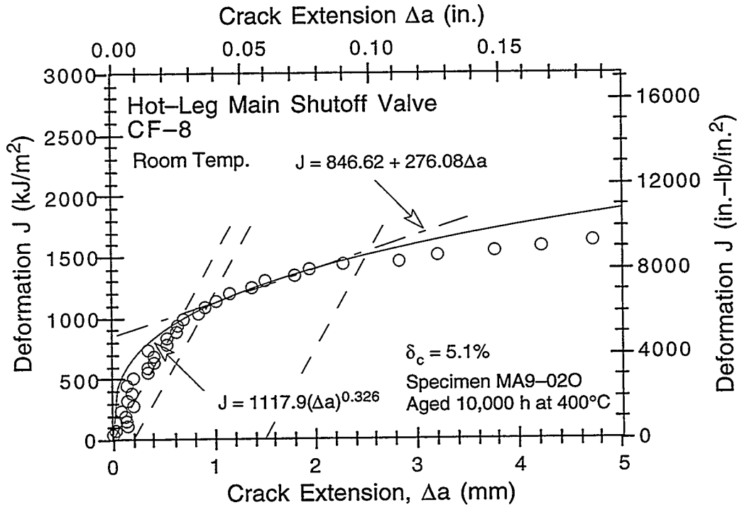
Figure C-24. Deformation J-R Curve at room temperature for material from cooler region of the hot-leg main shutoff valve aged 10,000 h at 400°C
