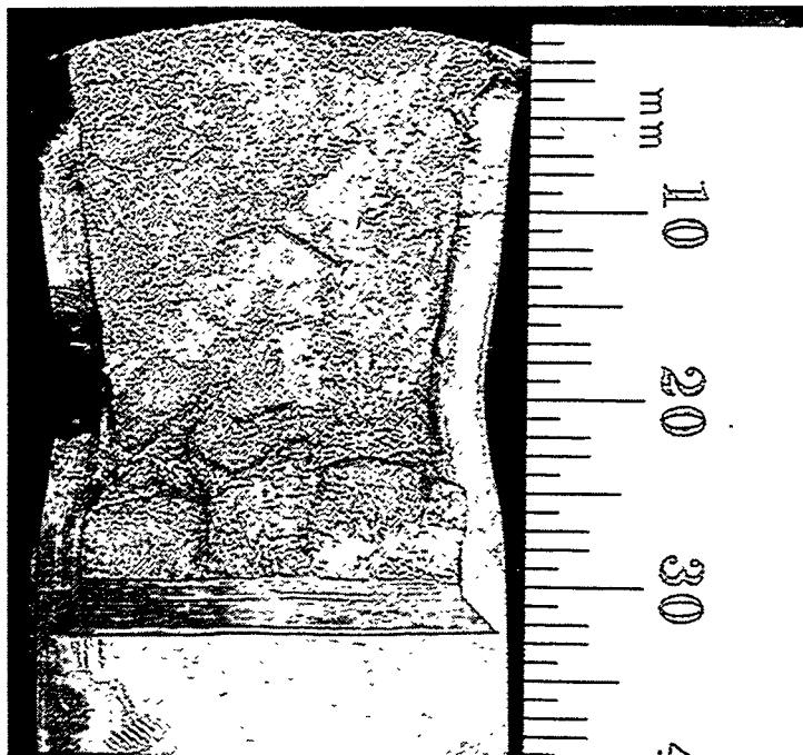
Figure C-35. Fracture surface of pump volute PV tested at room temperature after 13 y of service at 264°C
