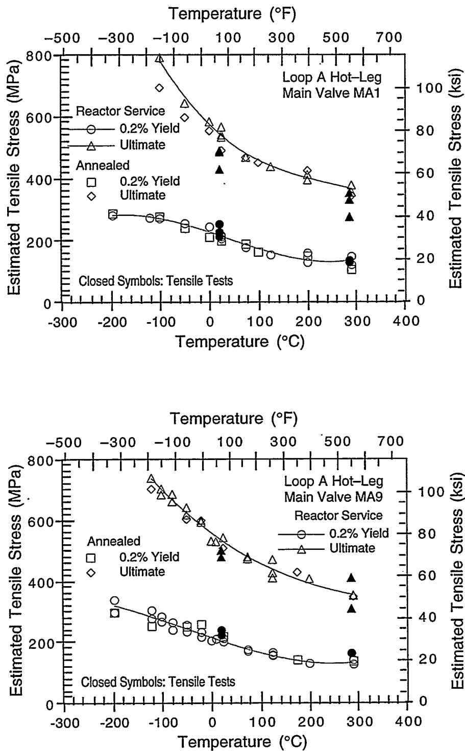
Figure 15. Yield and ultimate stresses estimated from Charpy-impact data and obtained from tensile tests for hot-leg main valve, and estimated tensile stresses of annealed materials. Material MA9 is from a cooler region of the valve.
