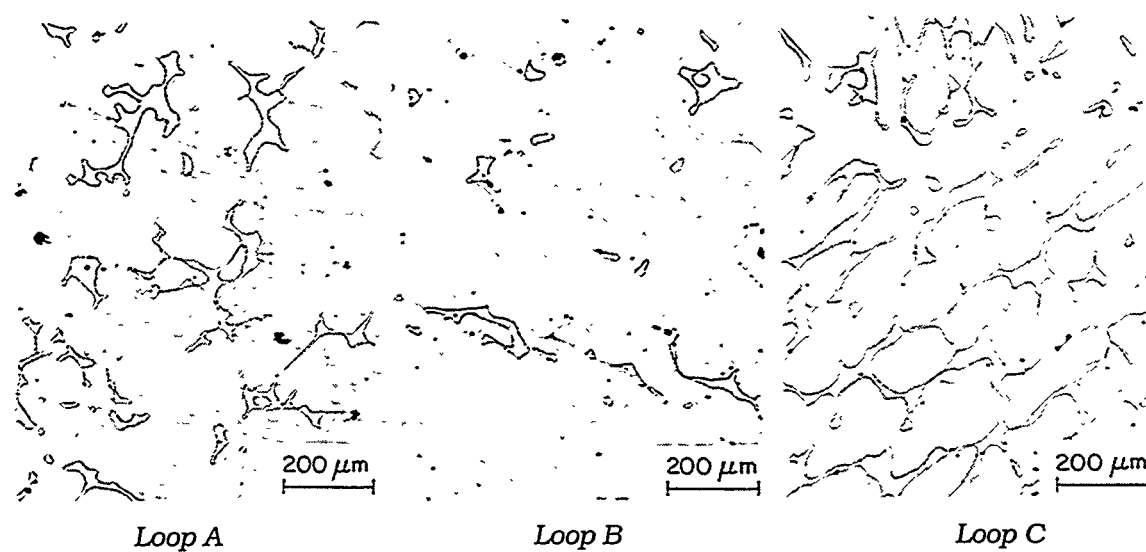
Figure 6. Ferrite morphology of cast materials from Loops A, B, and C hot-leg main shutoff valves from the Shippingport reactor
