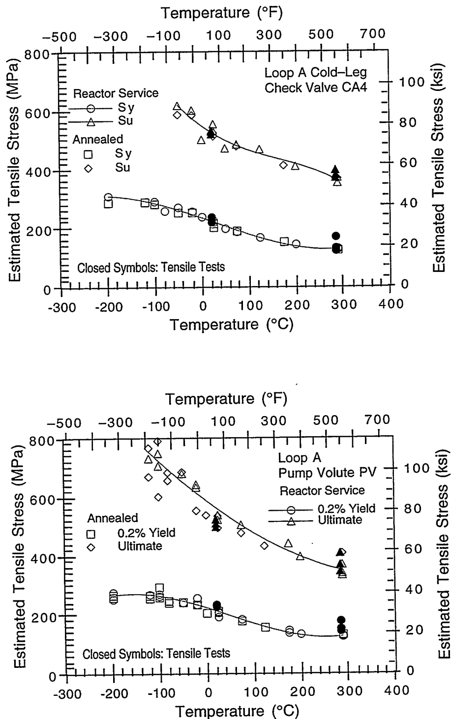
Figure 14. Yield and ultimate stresses estimated from Charpy-impact data and obtained from tensile tests for cold-leg check valve and pump volute, and estimated tensile stresses of annealed materials
