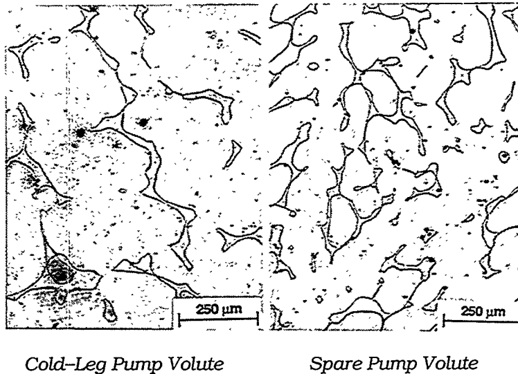
Figure 7. Ferrite morphology of cast materials from the cold-leg and spare pump volutes from the Shippingport reactor
