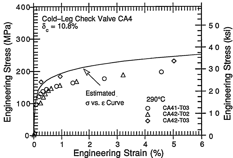
Figure 29. Estimated and measured tensile stress-vs.-strain curves at room temperature and 290°C for the cold-leg check valve after service for \approx 13 y at 264°C
