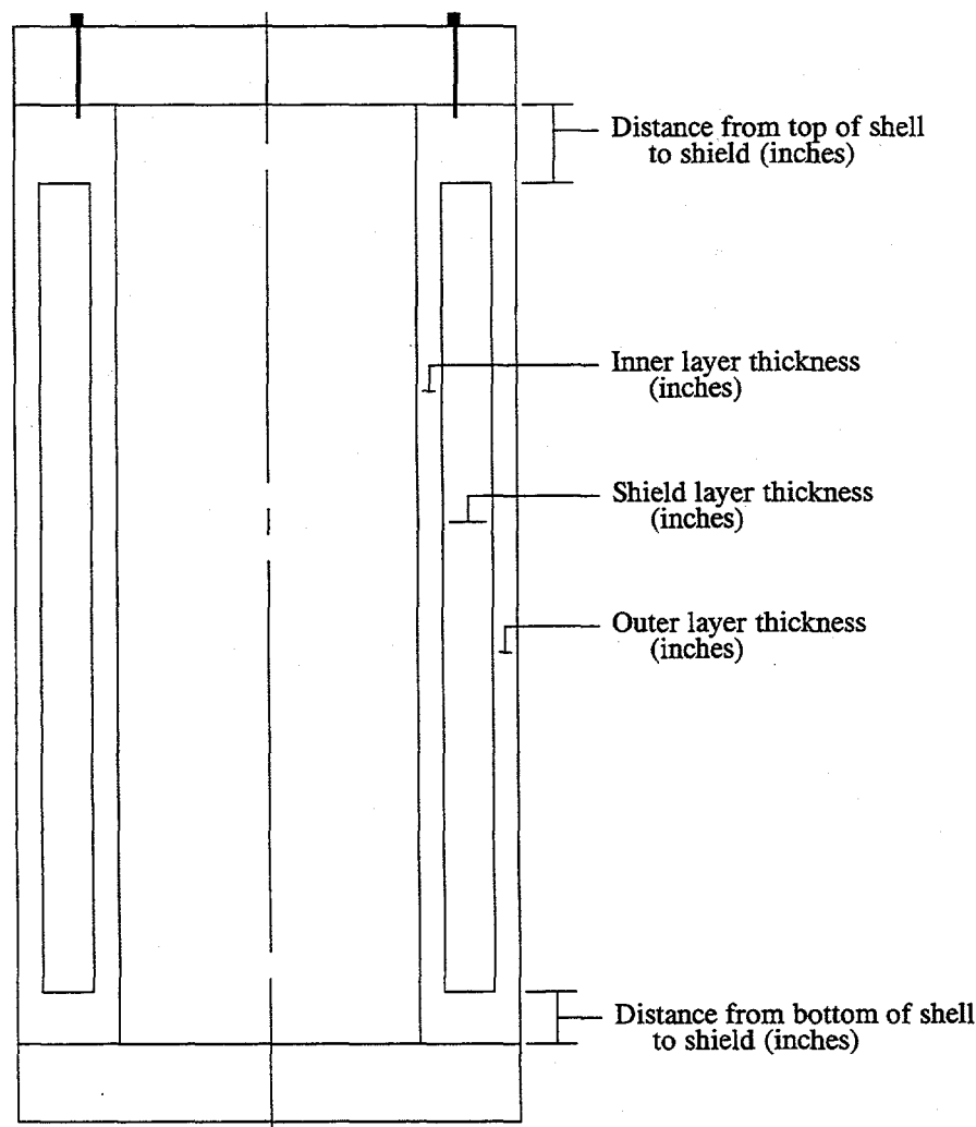
Figure 3-6. Dimensions required to specify a laminated shell.
