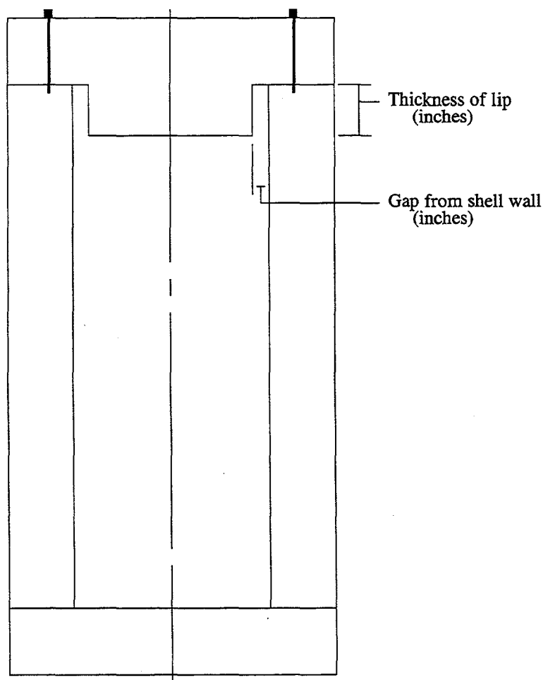
Figure 3-11. Dimensions required to specify the lip for a solid top end cap.
