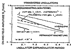
Figure 1. On-axis field performance of selected technologies.
