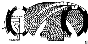
Figure 2. SC bifilar winding design with low field harmonics.
